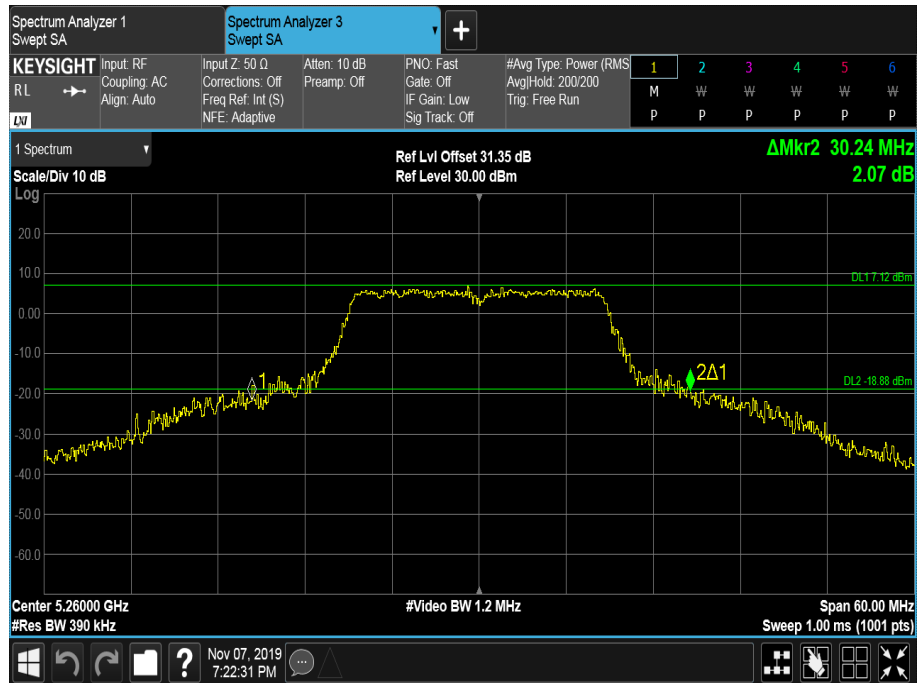
Figure 259 - 5260 MHz - 26 dB Emission Bandwidth
