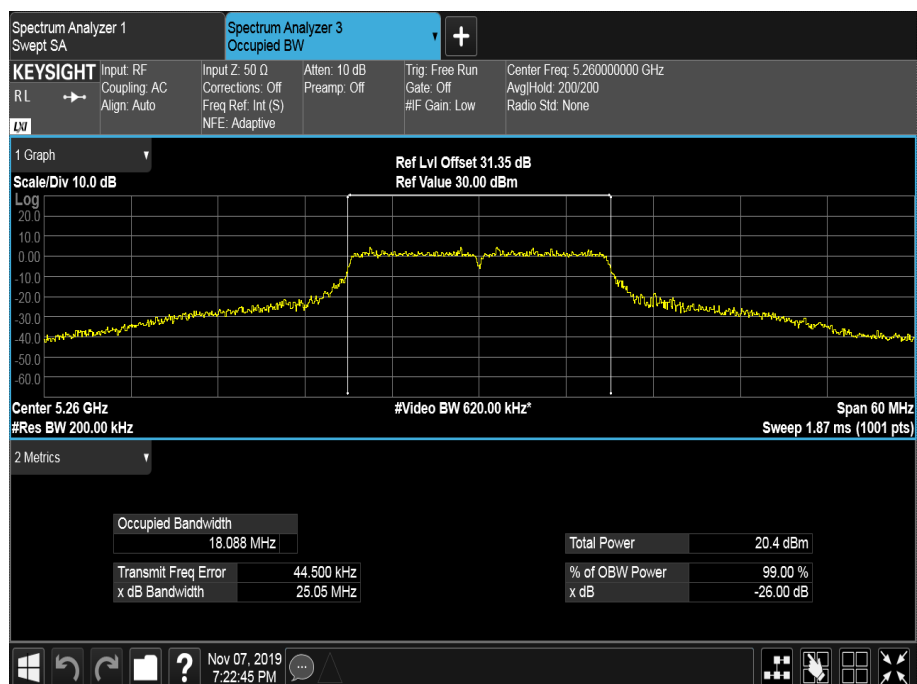
Figure 260 - 5260 MHz - 99% Occupied Bandwidth
