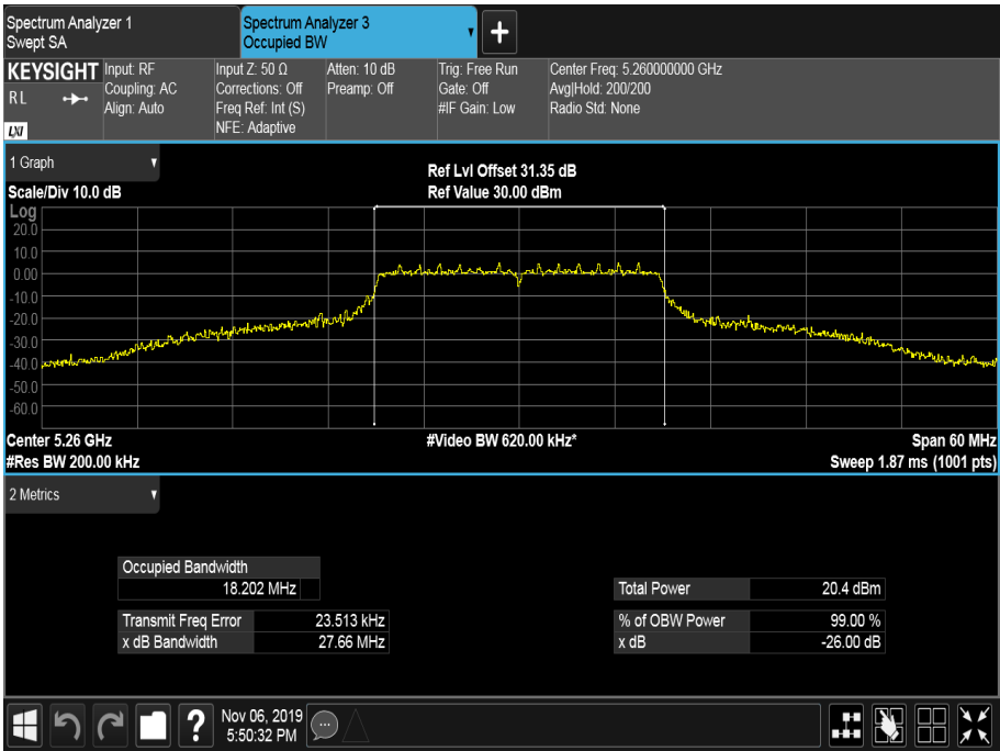
Figure 254 - 5260 MHz - 99% Occupied Bandwidth
