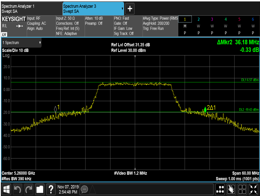
Figure 253 - 5260 MHz - 26 dB Emission Bandwidth
