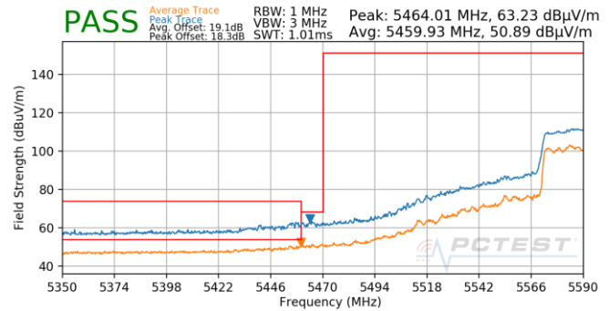
Plot 7-1078. (FCC Only) CDD (Pk & Avg, Ch.122, 802.11ac, MCS3)
