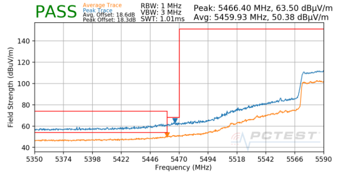
Plot 7-1077. (FCC Only) CDD (Pk & Avg, Ch.122, 802.11ac, MCS0)
