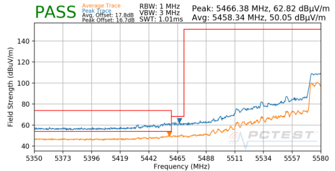
Plot 7-1079. (FCC Only) CDD (Pk & Avg, Ch.122, 802.11ac, MCS5)
