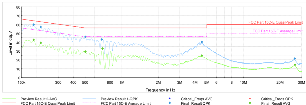
Plot 7-1114. AC Line Conducted Plot with 802.11ax(SU) CDD – Ch.40 (L1), with laptop
