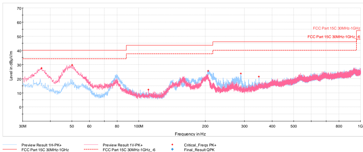
Plot 7-1111. Radiated Spurious Emissions below 1GHz CDD, 802.11ax (SU), Ch.40 with AC/DC Adapter
