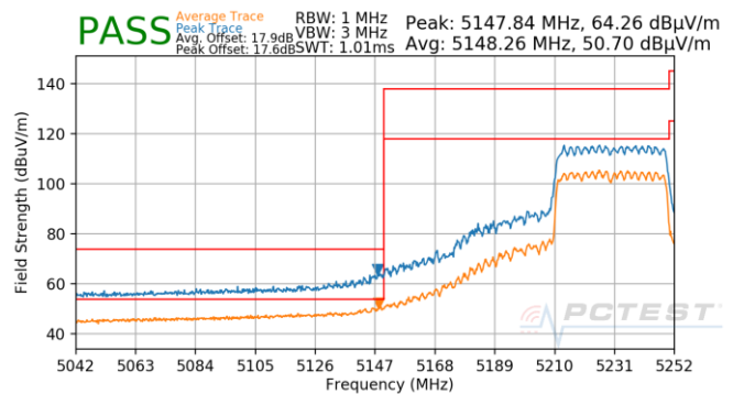
Plot 7-1039. CDD (Pk & Avg, Ch.46, 802.11ax(SU), MCS3)
