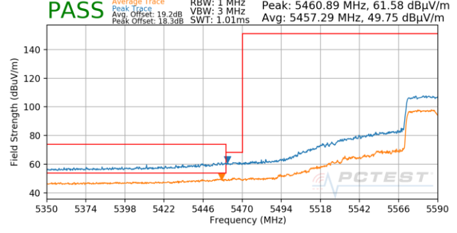
Plot 7-937. (FCC Only) Antenna 4b (Pk & Avg, Ch.122, 802.11ax(SU), MCS11)
