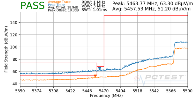
Plot 7-936. (FCC Only) Antenna 4b (Pk & Avg, Ch.122, 802.11ax(SU), MCS3)
