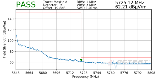
Plot 7-895. (FCC Only) Antenna 4b (Pk, Ch.126, 80.11ax(SU), MCS11)
