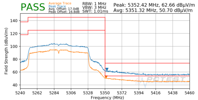
Plot 7-908. Antenna 4b (Pk & Avg, Ch.58, 802.11ac, MCS0)
