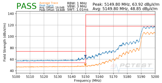
Plot 7-979. SDM (Pk & Avg, Ch.40, 802.11ax(SU), MCS3)
