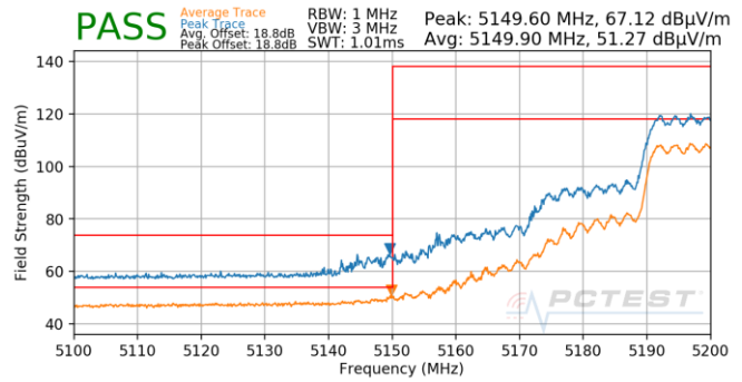
Plot 7-978. SDM (Pk & Avg, Ch.40, 802.11ax(SU), MCS0)
