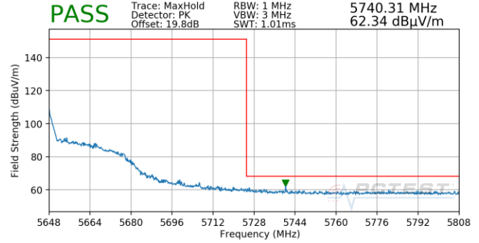
Plot 7-862. (FCC Only) Antenna 4b (Pk, Ch.126, 802.11n, MCS5)
