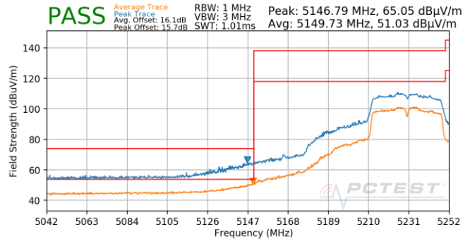
Plot 7-845. Antenna 4b (Pk & Avg, Ch.46, 802.11n, MCS3)
