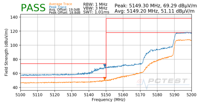
Plot 7-629. Antenna 5b (Pk & Avg, Ch.40, 802.11ax(SU), MCS3)
