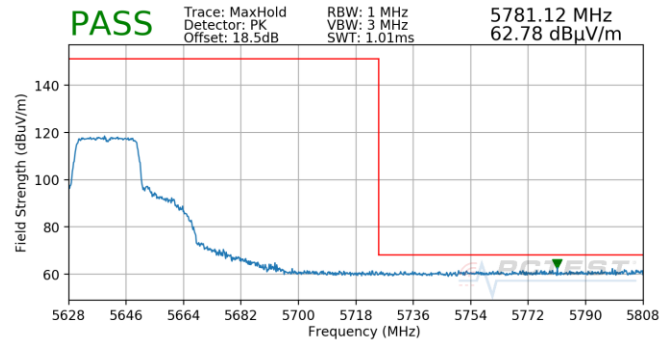
Plot 7-648. (FCC Only) Antenna 5b (Pk & Avg, Ch.128, 802.11ax(SU), MCS11)
