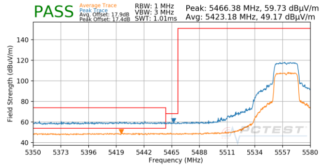
Plot 7-647. Antenna 5b (Pk & Avg, Ch.112, 802.11ax(SU), MCS11)
