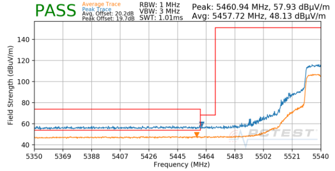
Plot 7-646. Antenna 5b (Pk & Avg, Ch.108, 802.11ax(SU), MCS11)
