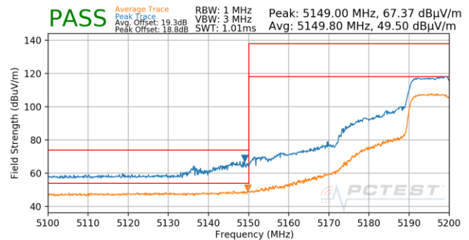
Plot 7-630. Antenna 5b (Pk & Avg, Ch.40, 802.11ax(SU), MCS11)
