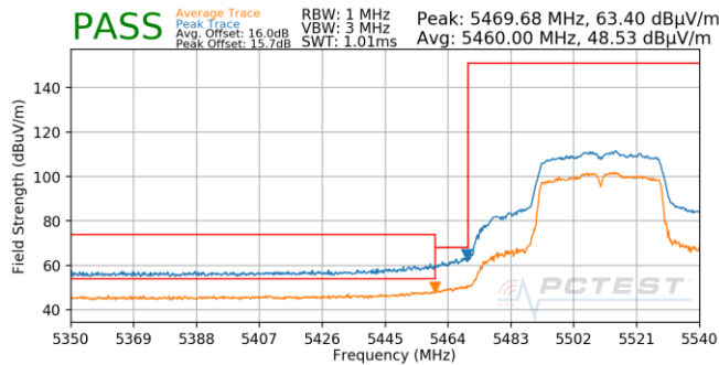
Plot 7-677. Antenna 5b (Pk & Avg, Ch.102, 802.11n, MCS3)
