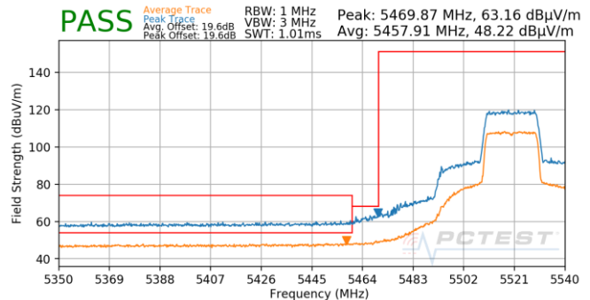
Plot 7-642. Antenna 5b (Pk & Avg, Ch.104, 802.11ax(SU), MCS0)
