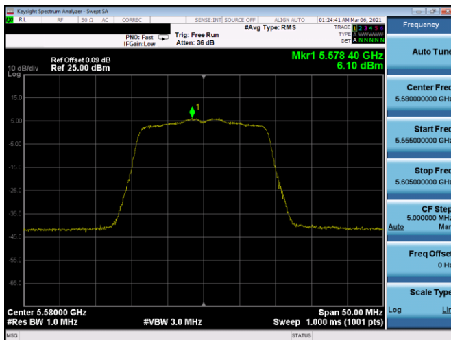
Plot 7-350. PSD SDM Antenna 4b (20MHz BW 802.11n – Ch. 116, MCS8)
