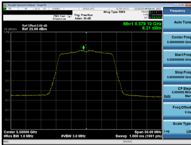
Plot 7-349. PSD SDM Antenna 5b (20MHz BW 802.11n – Ch. 116, MCS8)
