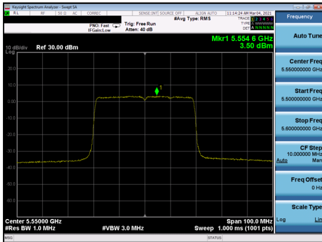
Plot 7-356. PSD CDD Antenna 4b (40MHz BW 802.11ax(SU) - Ch. 110, MCS0)
