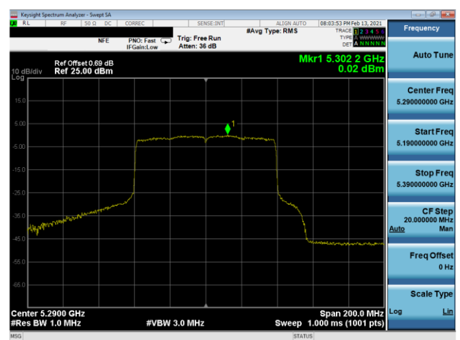
Plot 7-384. PSD CDD Antenna 4b (80MHz BW 802.11ax(SU) - Ch. 58, MCS3)
