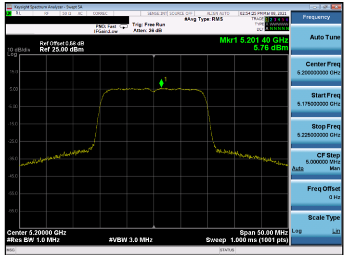
Plot 7-400. PSD SDM Antenna 4b (20MHz BW 802.11ax(SU) - Ch. 40, MCS11)
