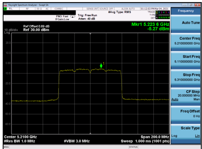
Plot 7-372. PSD CDD Antenna 4b (80MHz BW 802.11ax(SU) – Ch. 42, MCS3)
