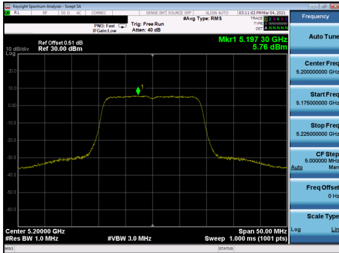
Plot 7-398. PSD SDM Antenna 4b (20MHz BW 802.11n - Ch. 40, MCS13)
