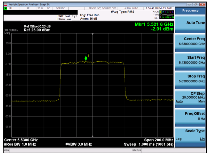
Plot 7-359. PSD CDD Antenna 5b (80MHz BW 802.11ax(SU) - Ch. 106, MCS0)
