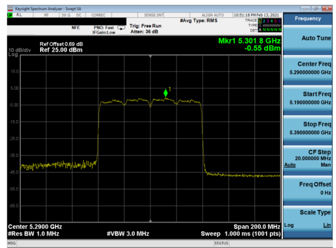
Plot 7-383. PSD CDD Antenna 5b (80MHz BW 802.11ax(SU) - Ch. 58, MCS3)
