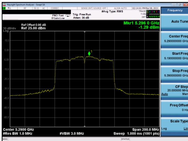
Plot 7-381. PSD CDD Antenna 5b (80MHz BW 802.11ac - Ch. 58, MCS3)
