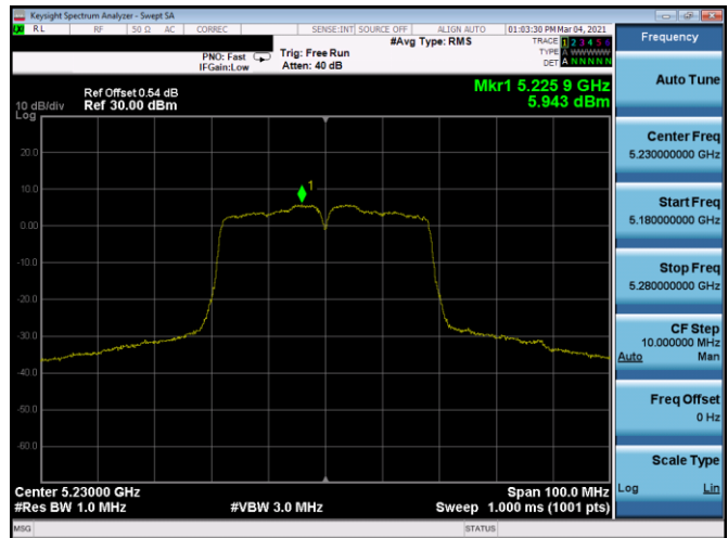
Plot 7-365. PSD SDM Antenna 5b (40MHz BW 802.11n - Ch. 46, MCS11)
