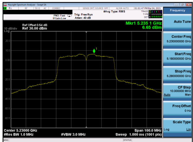
Plot 7-366. PSD SDM Antenna 4b (40MHz BW 802.11n - Ch. 46, MCS11)
