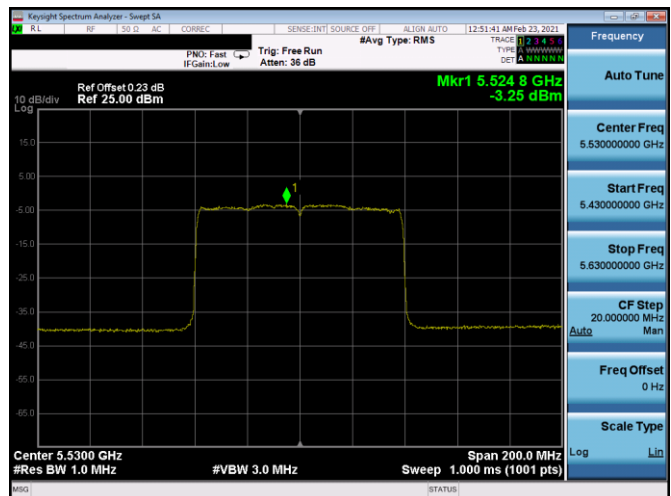
Plot 7-360. PSD CDD Antenna 4b (80MHz BW 802.11ax(SU) - Ch. 106, MCS0)
