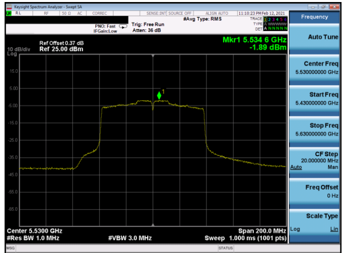
Plot 7-358. PSD CDD Antenna 4b (80MHz BW 802.11ac - Ch. 106, MCS0)
