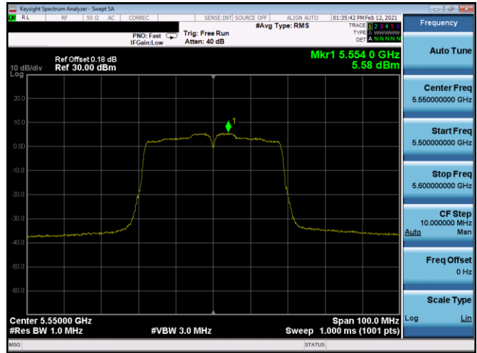
Plot 7-354. PSD SDM Antenna 4b (40MHz BW 802.11n – Ch. 110, MCS8)
