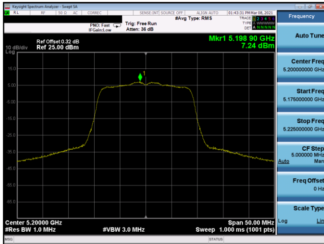
Plot 7-361. PSD SDM Antenna 5b (20MHz BW 802.11n - Ch. 40, MCS11)
