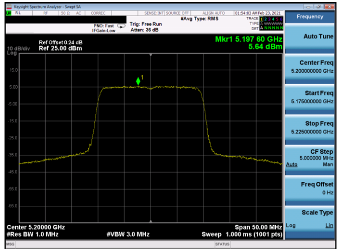
Plot 7-364. PSD SDM Antenna 4b (20MHz BW 802.11ax(SU) - Ch. 40, MCS3)
