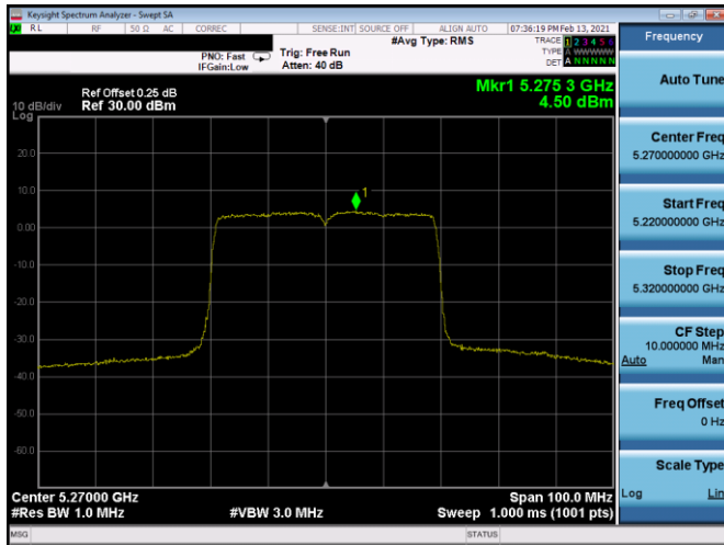
Plot 7-379. PSD SDM Antenna 5b (40MHz BW 802.11ax(SU) - Ch. 54, MCS3)
