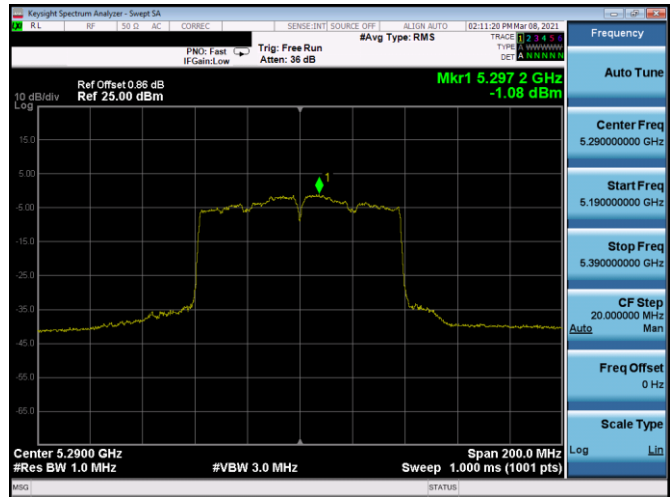
Plot 7-382. PSD CDD Antenna 4b (80MHz BW 802.11ac - Ch. 58, MCS3)
