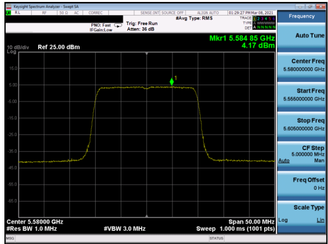
Plot 7-352. PSD SDM Antenna 4b (20MHz BW 802.11ax(SU) – Ch. 116, MCS0)
