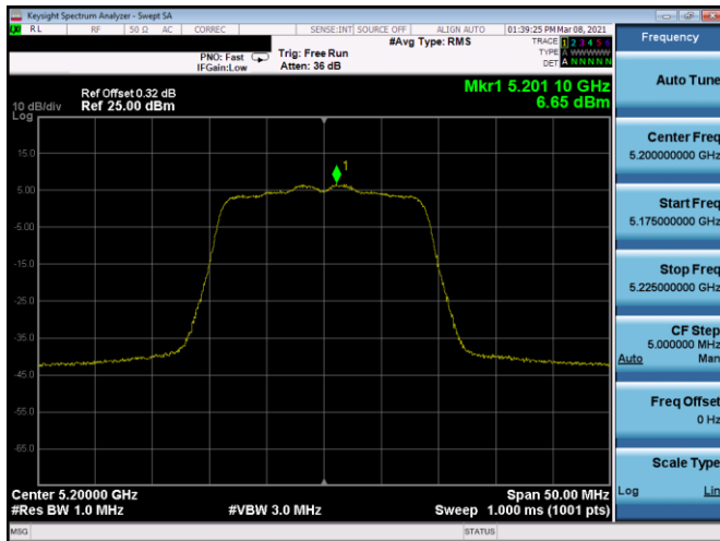
Plot 7-362. PSD SDM Antenna 4b (20MHz BW 802.11n - Ch. 40, MCS11)
