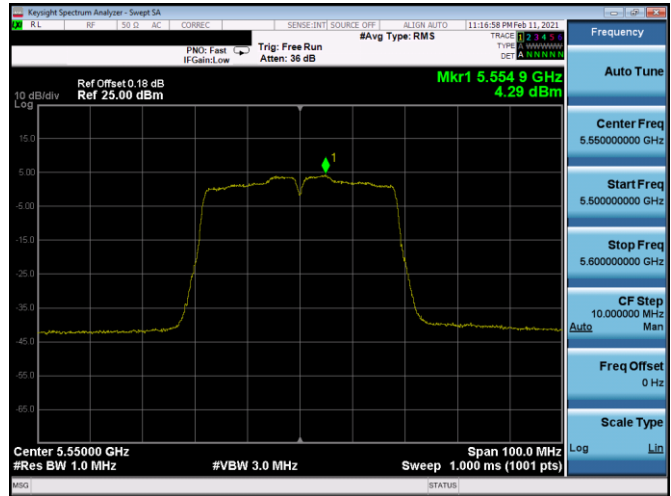
Plot 7-353. PSD SDM Antenna 5b (40MHz BW 802.11n – Ch. 110, MCS8)
