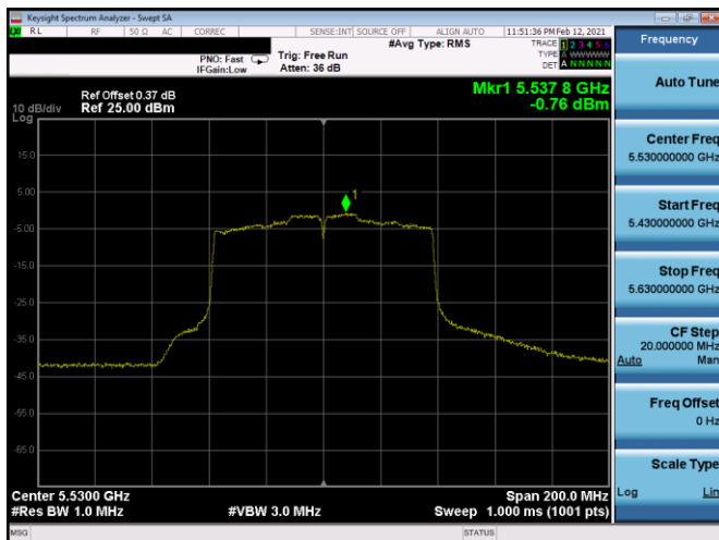
Plot 7-357. PSD CDD Antenna 5b (80MHz BW 802.11ac - Ch. 106, MCS0)
