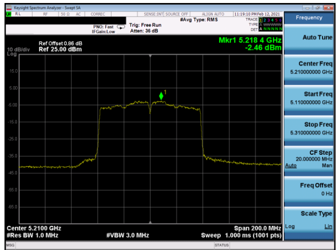
Plot 7-370. PSD CDD Antenna 4b (80MHz BW 802.11ac – Ch. 42, MCS3)
