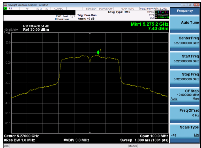
Plot 7-378. PSD SDM Antenna 4b (40MHz BW 802.11n - Ch. 54, MCS11)
