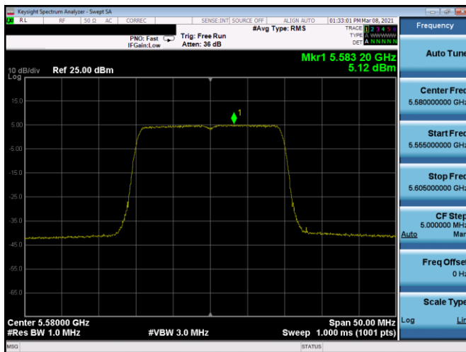
Plot 7-351. PSD SDM Antenna 5b (20MHz BW 802.11ax(SU) – Ch. 116, MCS0)
