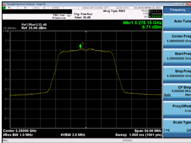
Plot 7-374. PSD SDM Antenna 4b (20MHz BW 802.11n - Ch. 56, MCS11)
