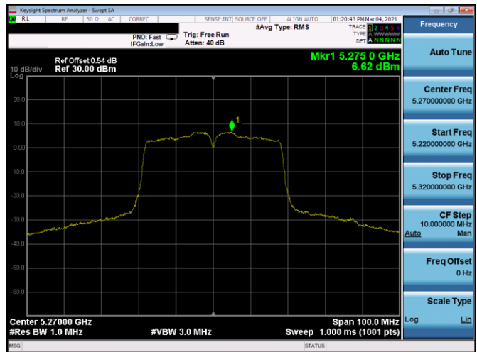
Plot 7-377. PSD SDM Antenna 5b (40MHz BW 802.11n - Ch. 54, MCS11)
