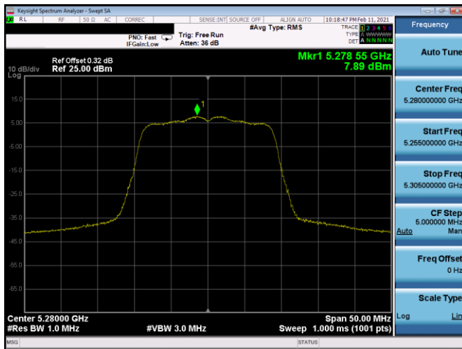
Plot 7-373. PSD SDM Antenna 5b (20MHz BW 802.11n - Ch. 56, MCS11)
