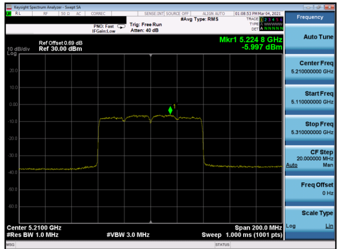
Plot 7-371. PSD CDD Antenna 5b (80MHz BW 802.11ax(SU) – Ch. 42, MCS3)
