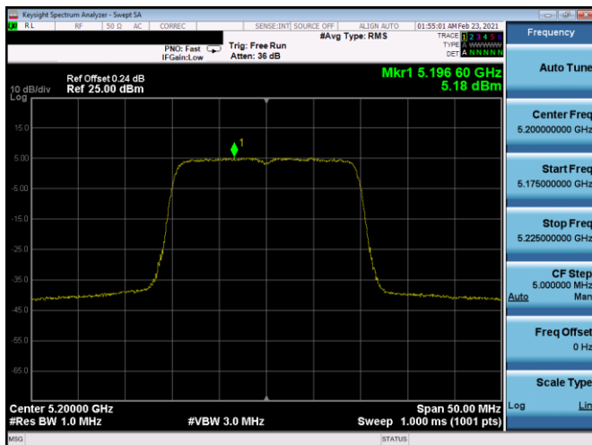
Plot 7-363. PSD SDM Antenna 5b (20MHz BW 802.11ax(SU) - Ch. 40, MCS3)
