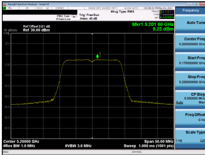
Plot 7-397. PSD SDM Antenna 5b (20MHz BW 802.11n - Ch. 40, MCS13)
