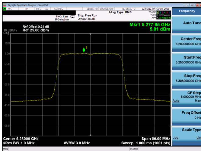
Plot 7-375. PSD SDM Antenna 5b (20MHz BW 802.11ax(SU) - Ch. 56, MCS3)
