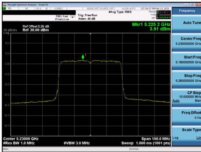
Plot 7-367. PSD CDD Antenna 5b (40MHz BW 802.11ax(SU) – Ch. 46, MCS3)
