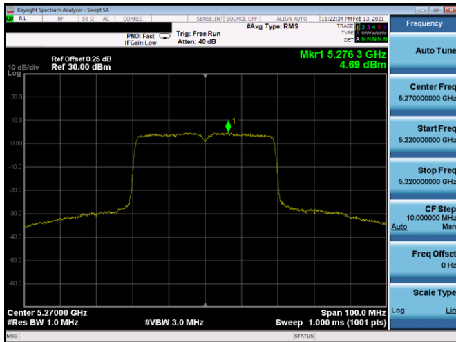
Plot 7-380. PSD SDM Antenna 4b (40MHz BW 802.11ax(SU) - Ch. 54, MCS3)
