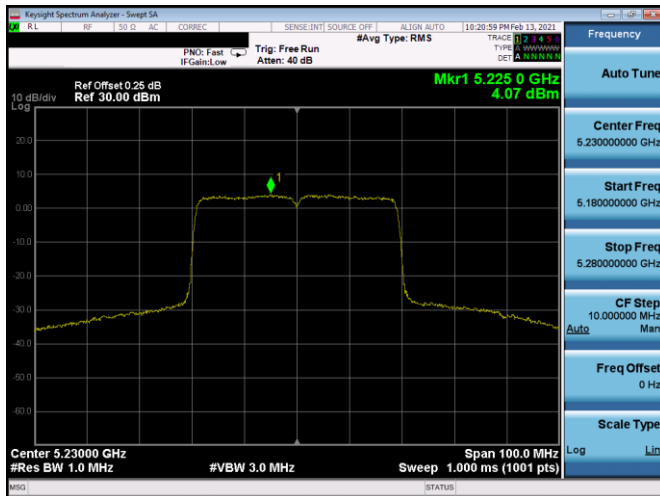
Plot 7-368. PSD CDD Antenna 4b (40MHz BW 802.11ax(SU) – Ch. 46, MCS3)
