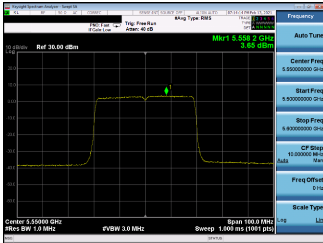
Plot 7-355. PSD CDD Antenna 5b (40MHz BW 802.11ax(SU) - Ch. 110, MCS0)
