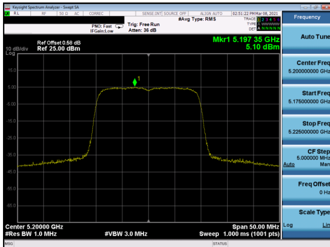
Plot 7-399. PSD SDM Antenna 5b (20MHz BW 802.11ax(SU) - Ch. 40, MCS11)
