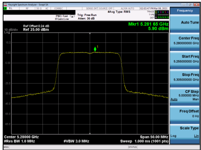
Plot 7-376. PSD SDM Antenna 4b (20MHz BW 802.11ax(SU) - Ch. 56, MCS3)
