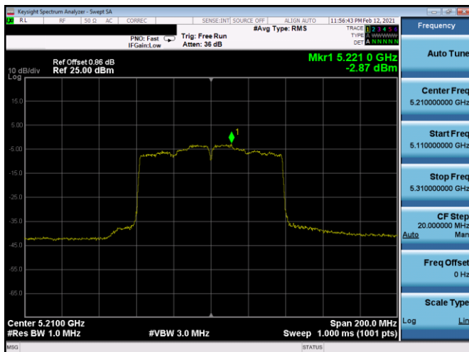
Plot 7-369. PSD CDD Antenna 5b (80MHz BW 802.11ac – Ch. 42, MCS3)
