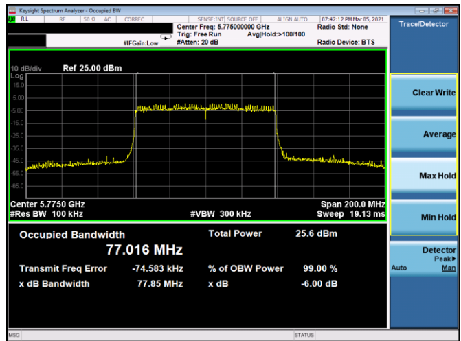
Plot 7-132. 6dB BW & 99% OBW Antenna 4b (80MHz BW 802.11ax(SU) – Ch. 155, MCS0)
