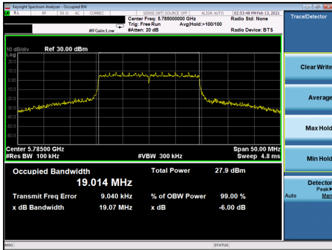
Plot 7-140. 6dB BW & 99% OBW Antenna 4b (20MHz BW 802.11ax(SU) – Ch. 157, MCS11)
