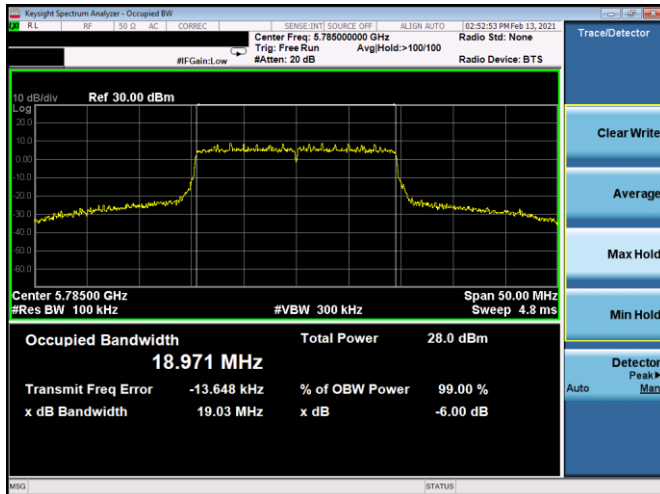
Plot 7-134. 6dB BW & 99% OBW Antenna 4b (20MHz BW 802.11ax(SU) – Ch. 157, MCS3)
