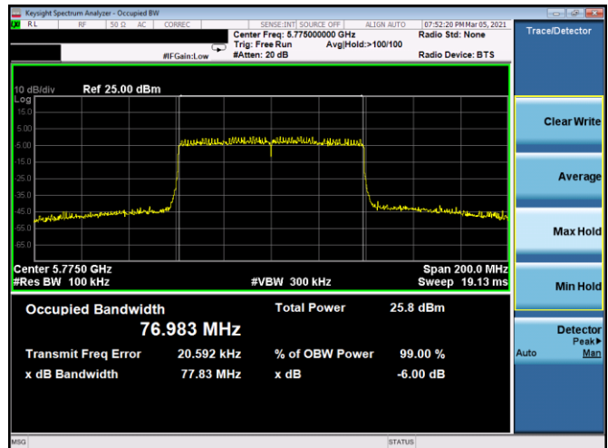
Plot 7-138. 6dB BW & 99% OBW Antenna 4b (80MHz BW 802.11ax(SU) – Ch. 155, MCS3)
