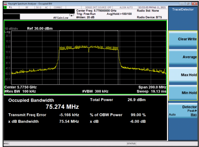
Plot 7-131. 6dB BW & 99% OBW Antenna 4b (80MHz BW 802.11ac – Ch. 155, MCS0)
