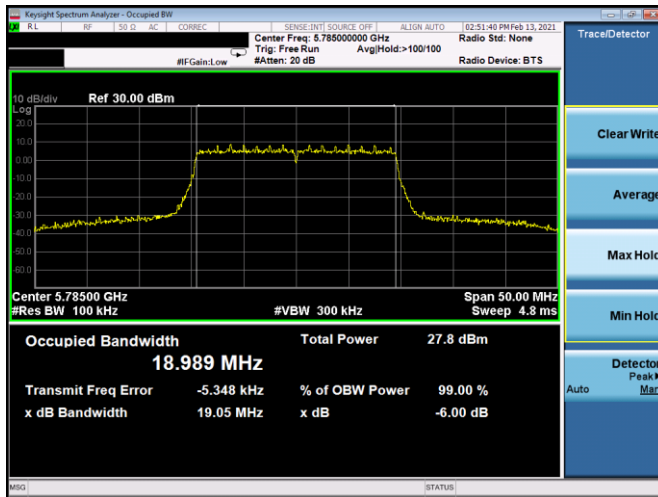
Plot 7-128. 6dB BW & 99% OBW Antenna 4b (20MHz BW 802.11ax(SU) – Ch. 157, MCS0)
