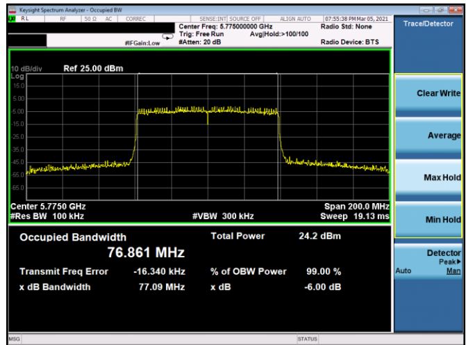
Plot 7-144. 6dB BW & 99% OBW Antenna 4b (80MHz BW 802.11ax(SU) – Ch. 155, MCS11)
