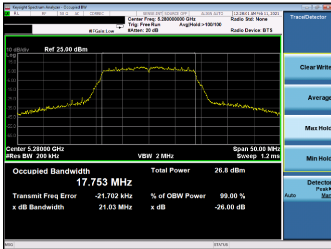
Plot 7-7. 26dB BW & 99% OBW Antenna 5b (20MHz BW 802.11n – Ch. 56, MCS0)
