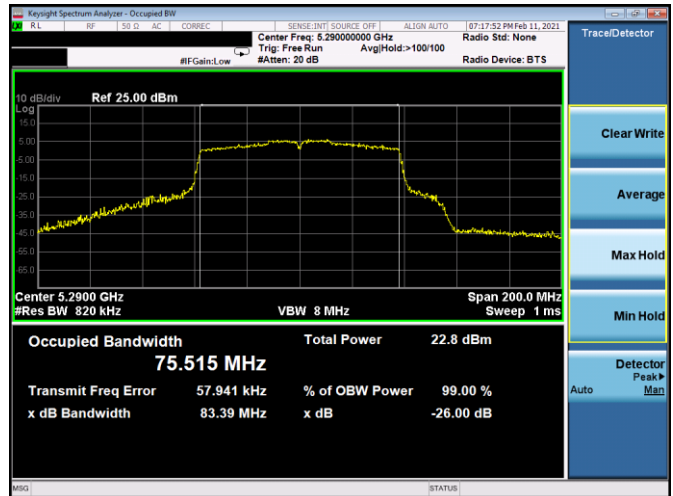
Plot 7-11. 26dB BW & 99% OBW Antenna 5b (80MHz BW 802.11ac – Ch. 58, MCS0)
