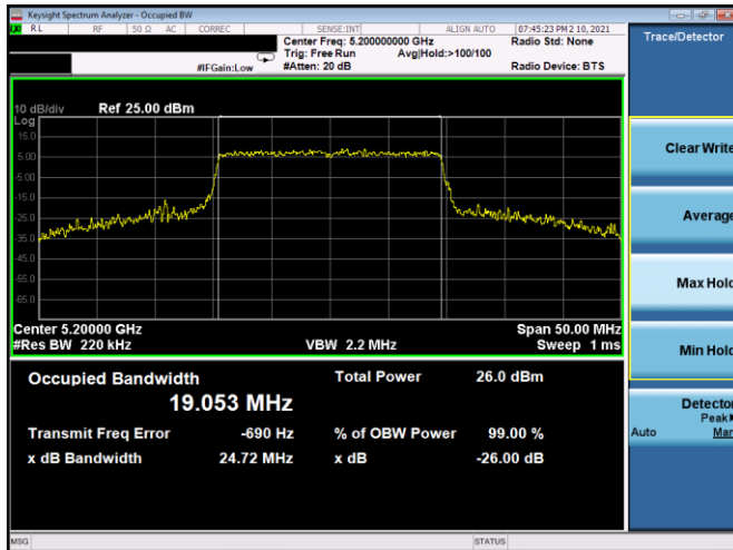
Plot 7-38. 26dB BW & 99% OBW Antenna 5b (20MHz BW 802.11ax(SU) – Ch. 40, MCS11)
