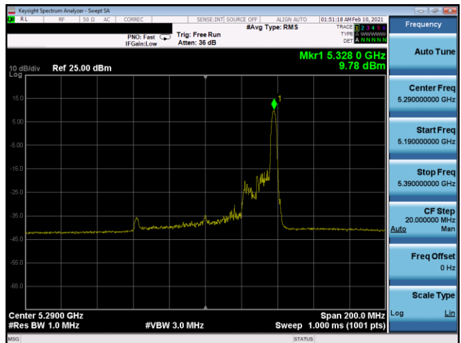
Plot 17-179. PSD Antenna 4b (80MHz BW 11ax Index 36 – RU26 – Ch.58)
