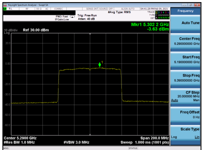
Plot 17-180. PSD Antenna 4b (80MHz BW 11ax – RU996 – Ch.58)
