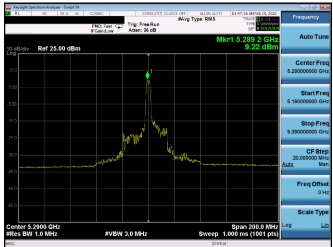
Plot 17-178. PSD Antenna 4b (80MHz BW 11ax Index 18 – RU26 – Ch.58)
