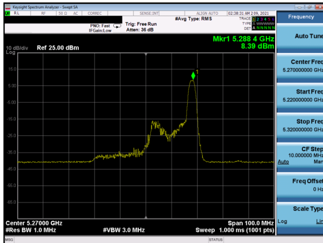
Plot 17-175. PSD Antenna 4b (40MHz BW 11ax Index 17 – RU26 – Ch.54)
