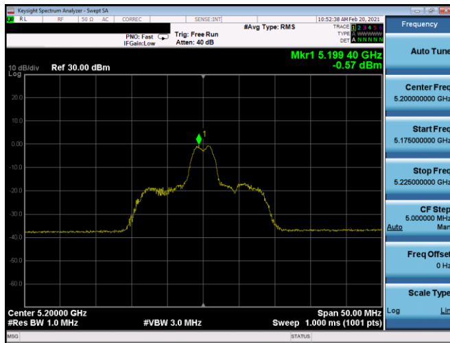
Plot 7-206. ISPD PSD Antenna 4b (20MHz BW 11ax Index 4 - RU26 - Ch.40)
