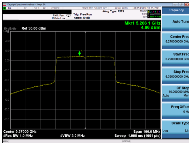
Plot 17-176. PSD Antenna 4b (40MHz BW 11ax – RU484 – Ch.54)
