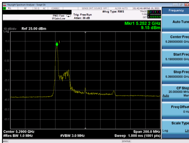
Plot 17-177. PSD Antenna 4b (80MHz BW 11ax Index 0 – RU26 – Ch.58)
