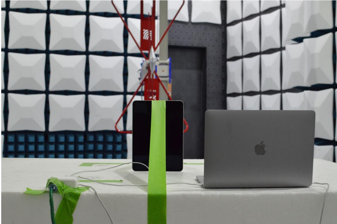
Figure 23: 30MHz-1GHz Test Setup (Rear View)
