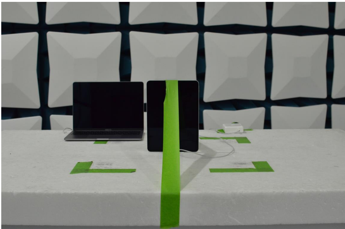
Figure 22: 30MHz-1GHz Test Setup (Front View)
