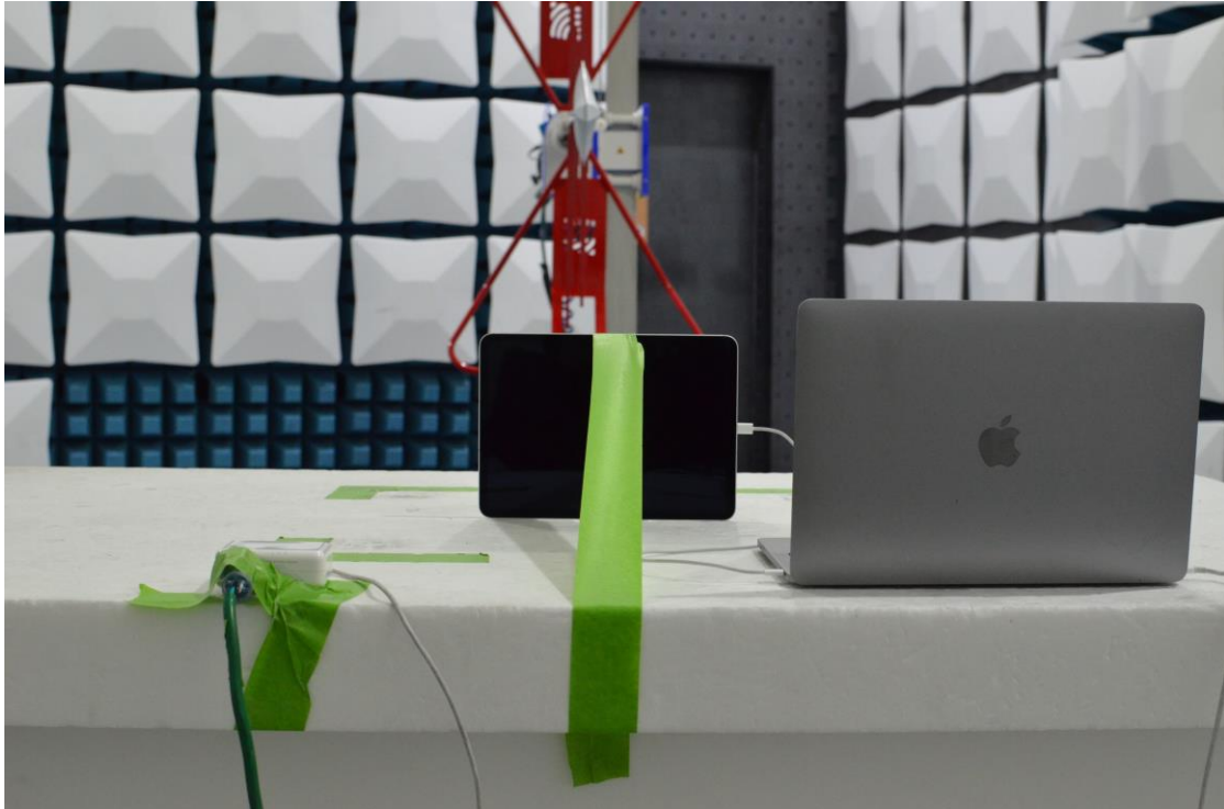
Figure 21: 30MHz-1GHz Test Setup (Rear View)
