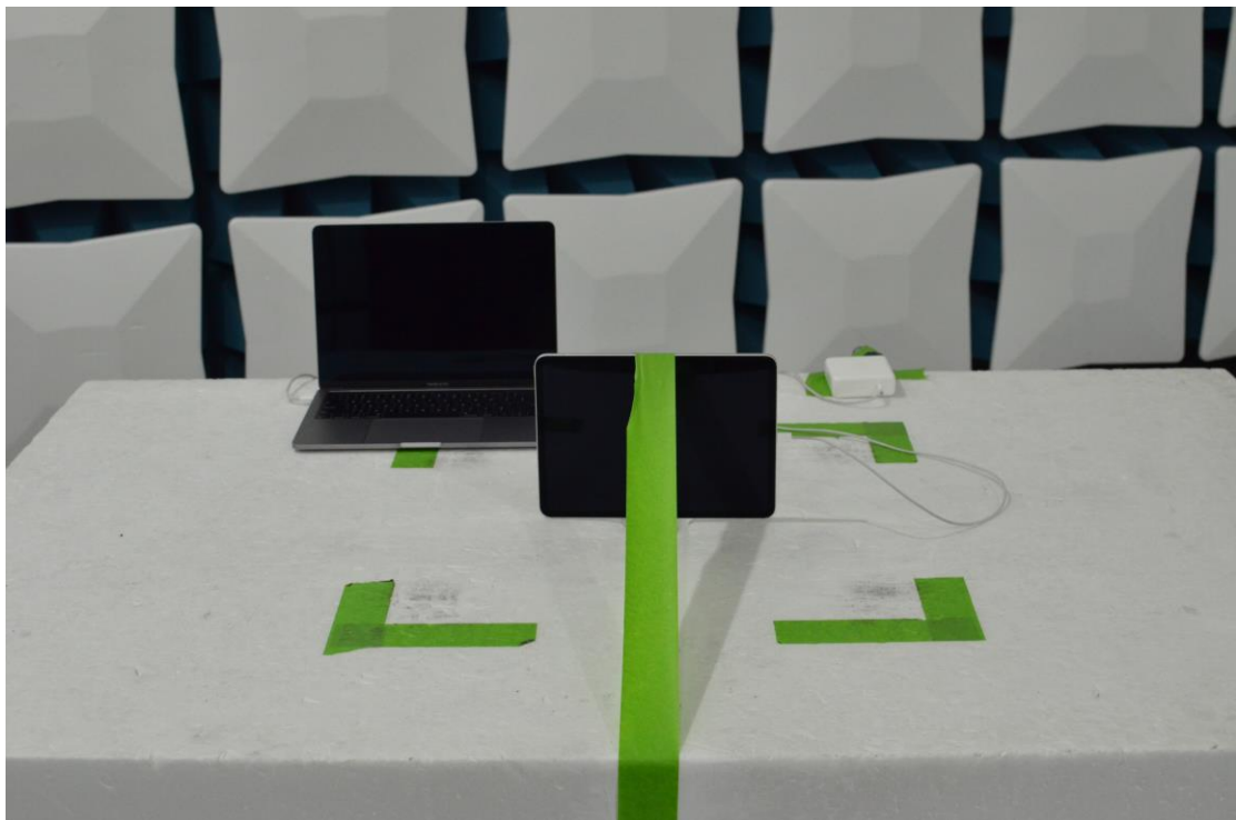
Figure 20: 30MHz-1GHz Test Setup (Front View)
