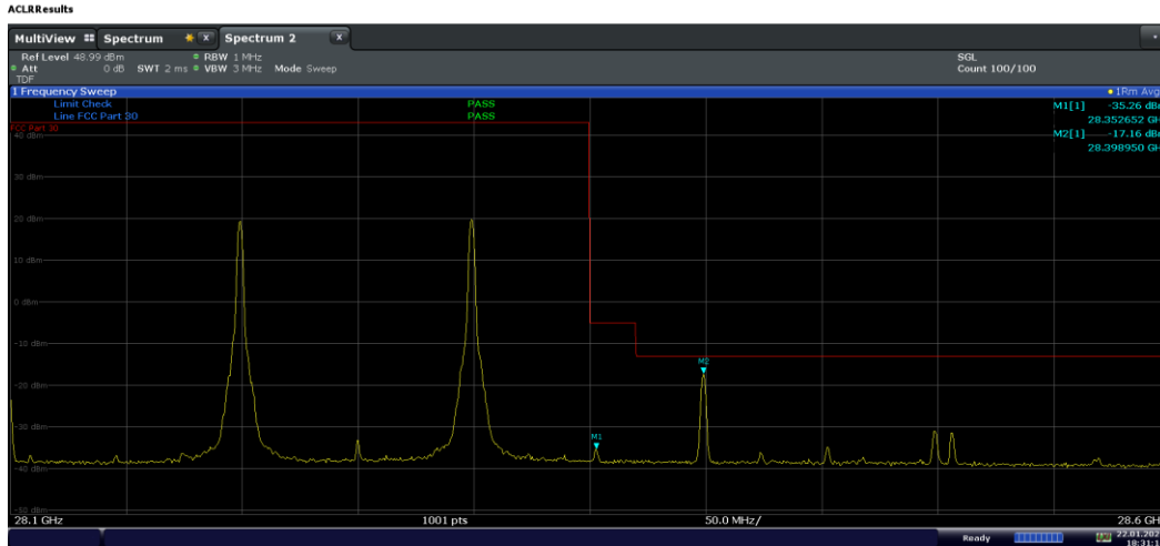
Plot 7-266. Ant M0 Upper BE (Band n261-100+100MHz-2CC SISO Dual Pol – \pi/2 BPSK 1-M RB)
