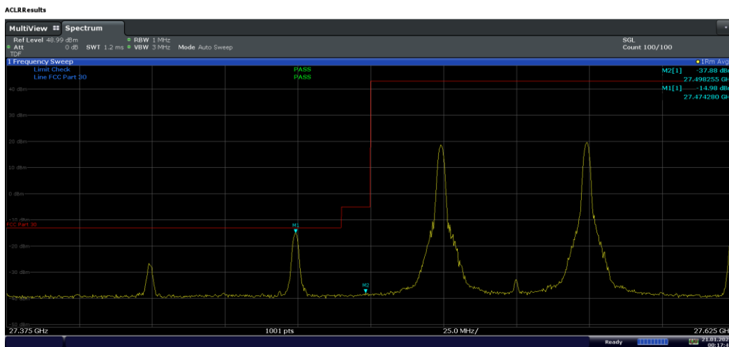
Plot 7-252. Ant M0 Lower BE (Band n261-50+50MHz-2CC SISO Dual Pol – 64QAM 1-M RB)
