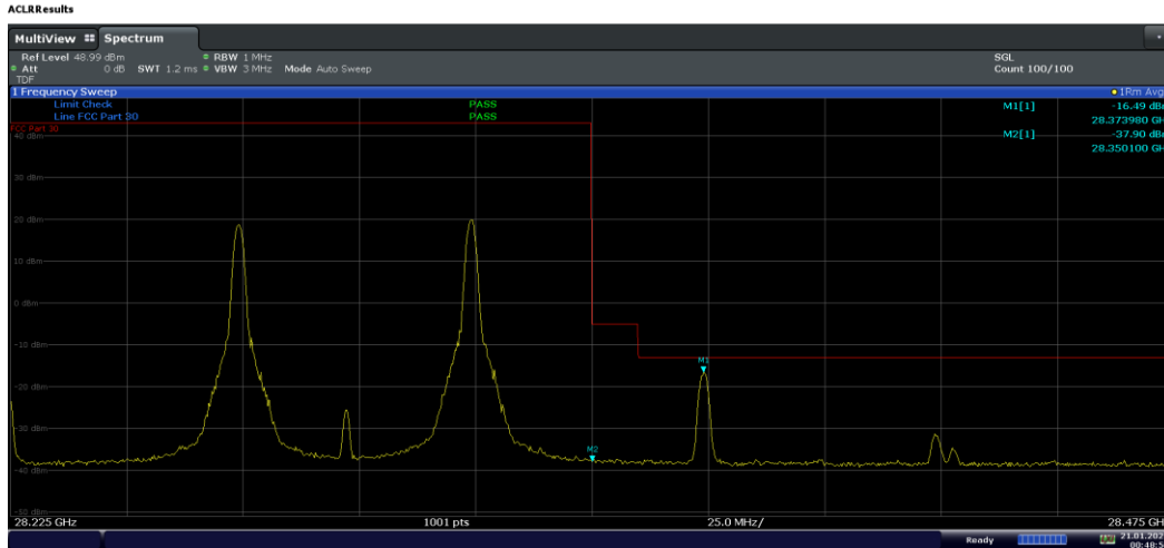
Plot 7-254. Ant M0 Upper BE (Band n261-50+50MHz-2CC SISO Dual Pol – \pi/2 BPSK 1-M RB)
