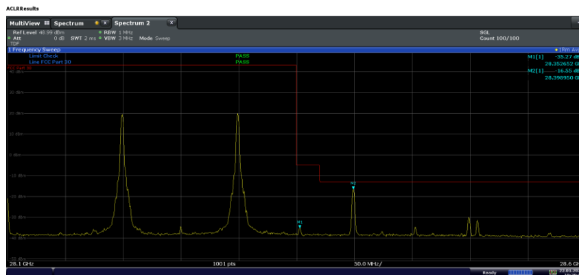
Plot 7-265. Ant M0 Upper BE (Band n261-100+100MHz-2CC SISO Dual Pol – QPSK 1-M RB)
