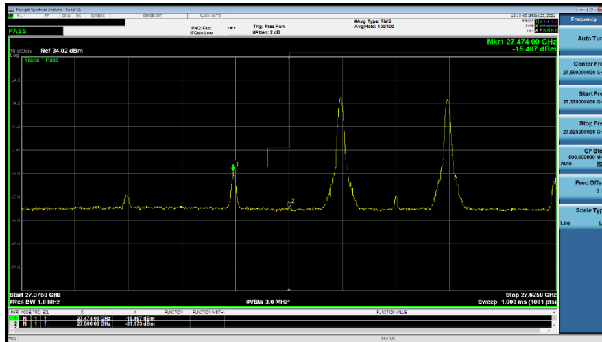
Plot 7-299. Ant M3 Lower BE (Band n261-50+50MHz-2CC SISO CP-OFDM – 16QAM 1-M RB)
