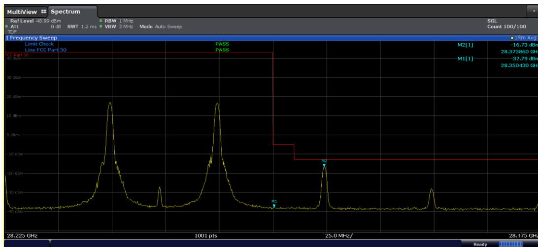
Plot 7-280. Ant M2 Upper BE (Band n261-50+50MHz-2CC SISO Dual Pol – 64QAM 1-M RB)
