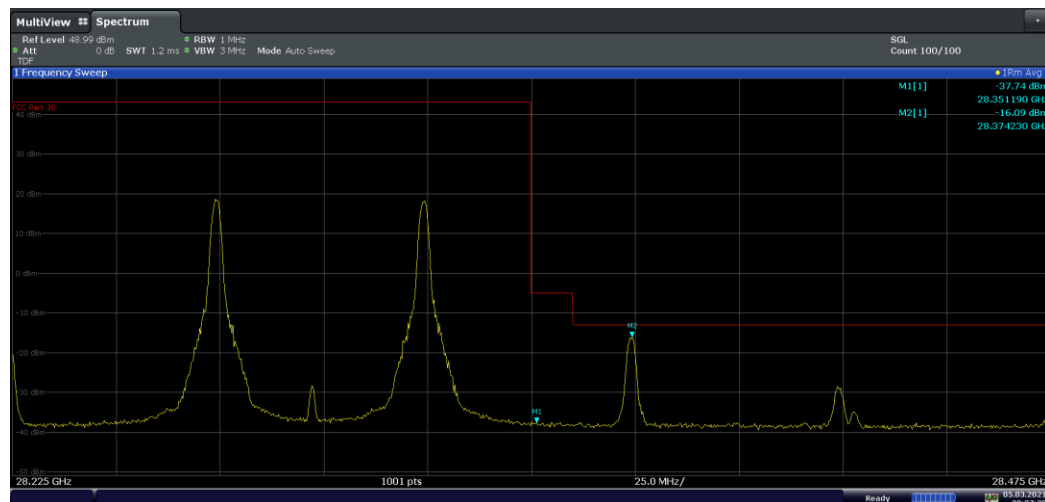
Plot 7-256. Ant M0 Upper BE (Band n261-50+50MHz-2CC SISO Dual Pol – 64QAM 1-M RB)
