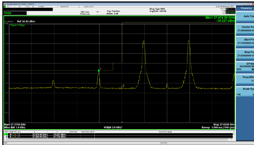
Plot 7-300. Ant M3 Lower BE (Band n261-50+50MHz-2CC SISO CP-OFDM – 64QAM 1-M RB)
