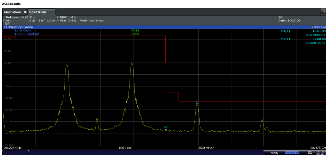
Plot 7-255. Ant M0 Upper BE (Band n261-50+50MHz-2CC SISO Dual Pol – 16QAM 1-M RB)
