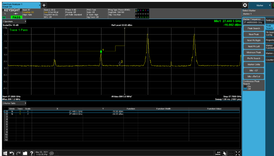
Plot 7-309. Ant M3 Lower BE (Band n261-100+100MHz-2CC SISO CP-OFDM – QPSK 1-M RB)
