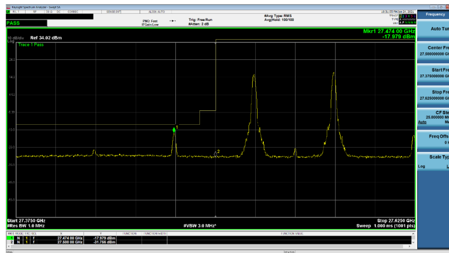
Plot 7-298. Ant M3 Lower BE (Band n261-50+50MHz-2CC SISO Dual Pol- \pi/2 BPSK 1-M RB)
