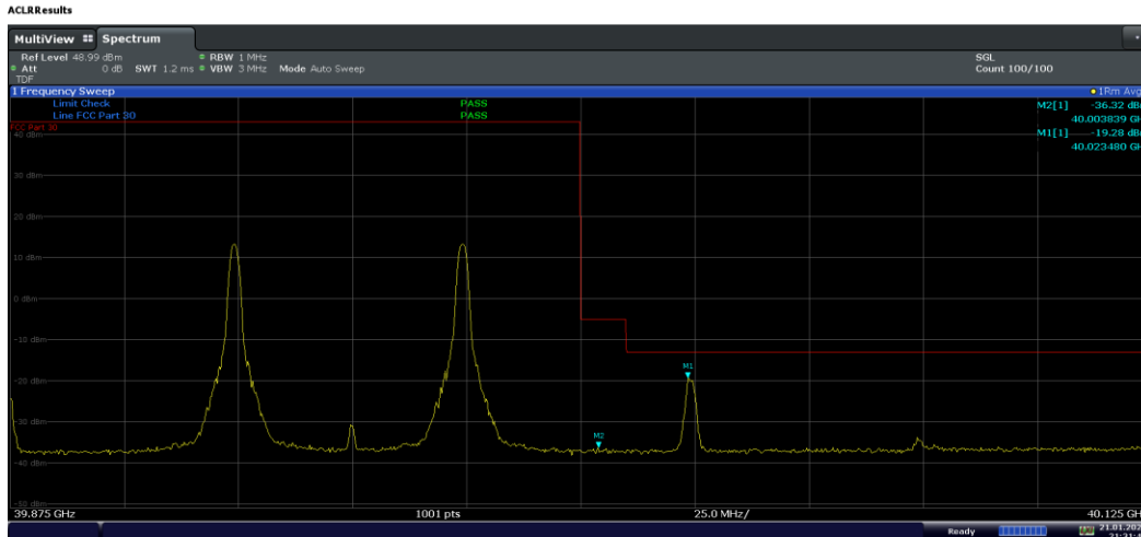
Plot 7-328. Ant M0 Upper BE (Band n260-50+50MHz-2CC SISO Dual Pol – 64QAM 1-M RB)
