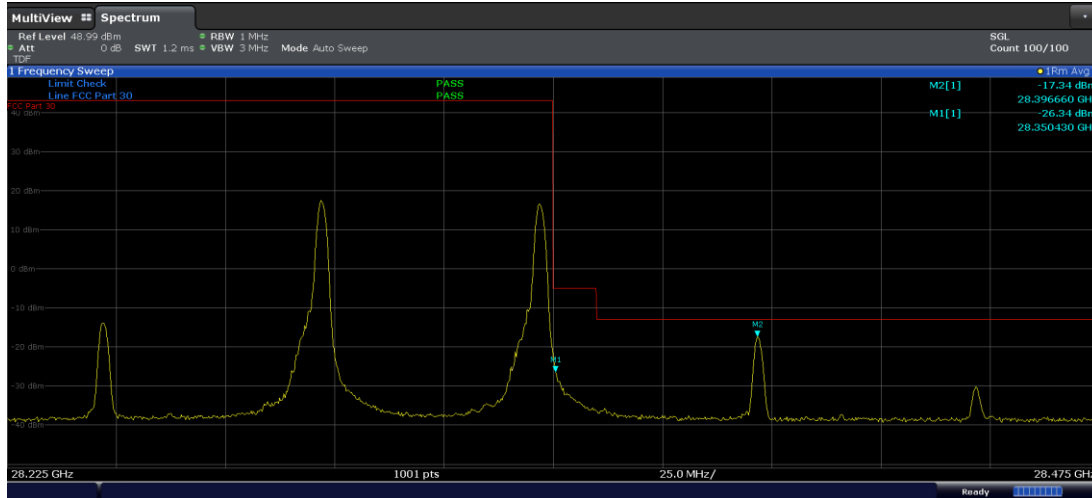
Plot 7-278. Ant M2 Upper BE (Band n261-50+50MHz-2CC SISO Dual Pol – \pi/2 BPSK 1-H RB)
