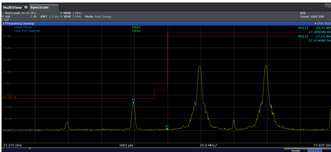
Plot 7-274. Ant M2 Lower BE (Band n261-50+50MHz-2CC SISO Dual Pol – \pi/2 BPSK 1-M RB)
