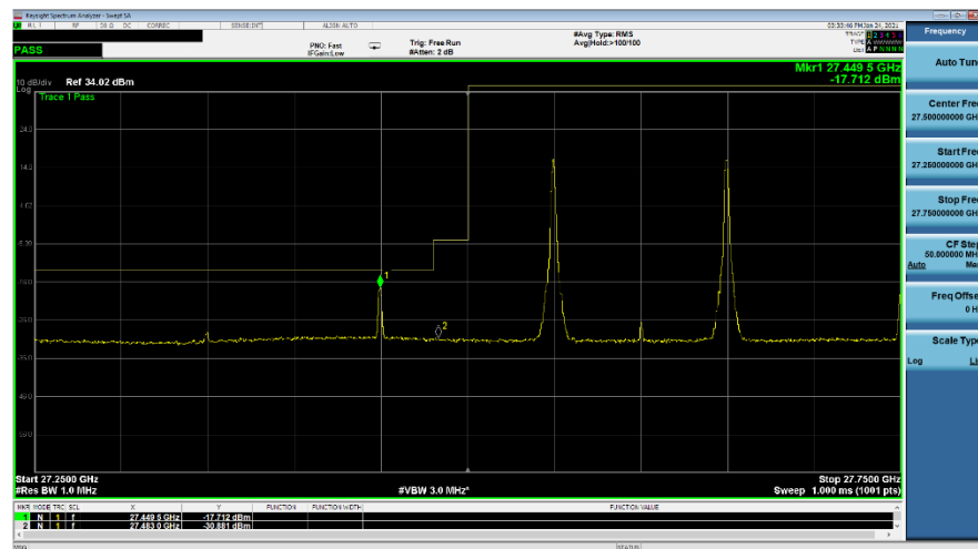
Plot 7-310. Ant M3 Lower BE (Band n261-100+100MHz-2CC SISO Dual Pol- \pi/2 BPSK 1-M RB)
