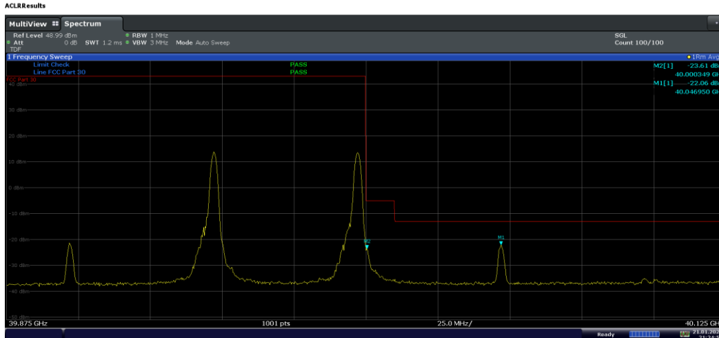
Plot 7-326. Ant M0 Upper BE (Band n260-50+50MHz-2CC SISO Dual Pol – \pi/2 BPSK 1-H RB)
