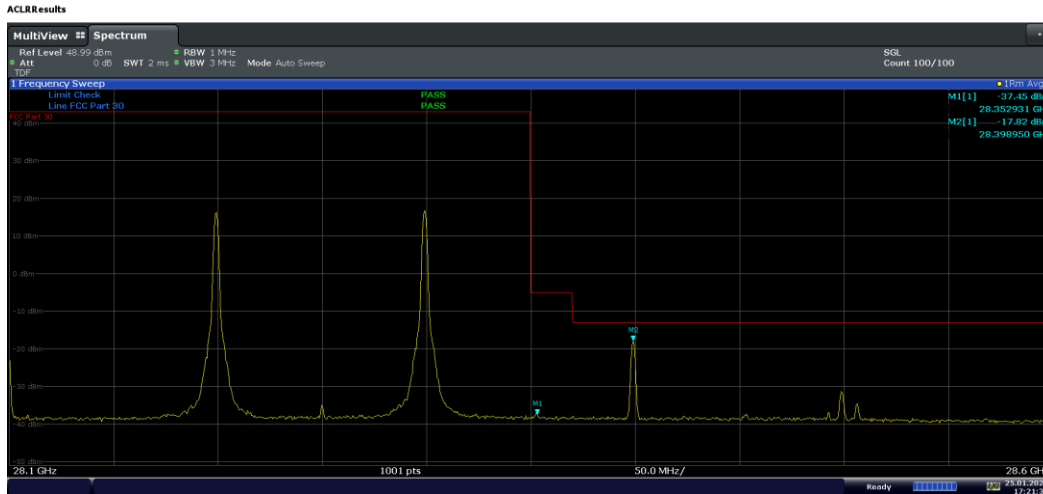
Plot 7-290. Ant M2 Upper BE (Band n261-100+100MHz-2CC SISO Dual Pol- \pi/2 BPSK 1-M RB)
