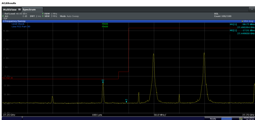
Plot 7-286. Ant M2 Lower BE (Band n261-100+100MHz-2CC SISO Dual Pol - \pi/2 BPSK 1-M RB)
