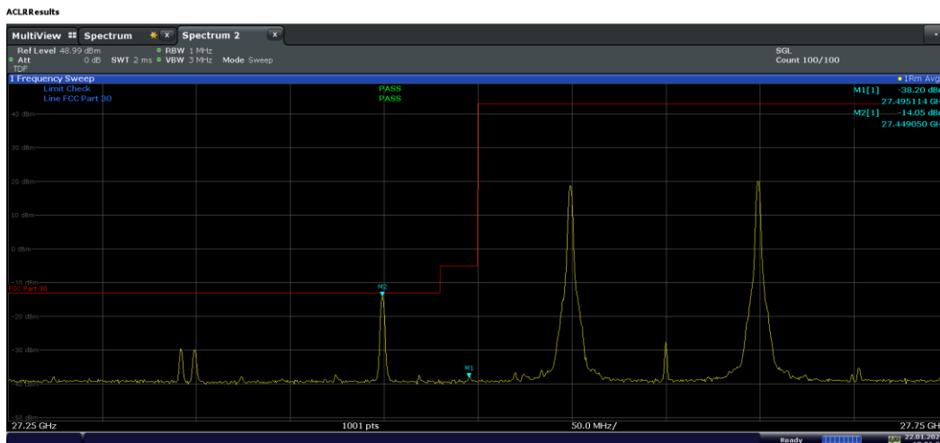
Plot 7-262. Ant M0 Lower BE (Band n261-100+100MHz-2CC SISO Dual Pol – \pi/2 BPSK 1-M RB)
