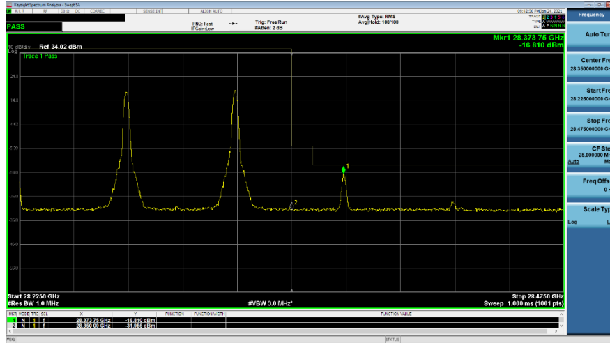
Plot 7-302. Ant M3 Upper BE (Band n261-50+50MHz-2CC SISO Dual Pol- \pi/2 BPSK 1-M RB)
