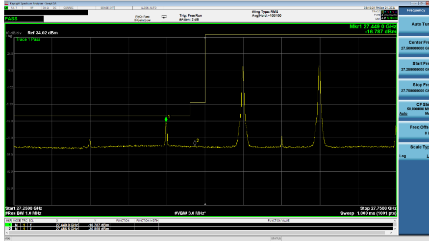
Plot 7-311. Ant M3 Lower BE (Band n261-100+100MHz-2CC SISO Dual Pol– 16QAM 1-M RB)
