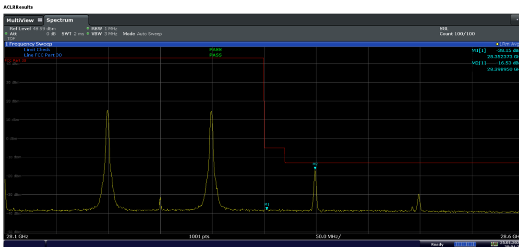
Plot 7-291. Ant M2 Upper BE (Band n261-100+100MHz-2CC SISO CP-OFDM – 16QAM 1-M RB)
