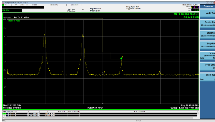
Plot 7-303. Ant M3 Upper BE (Band n261-50+50MHz-2CC SISO CP-OFDM – 16QAM 1-M RB)
