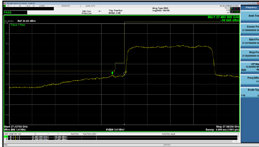
Plot 7-293. Ant M3 Lower BE (Band n261-50MHz-1CC SISO Dual Pol- QPSK Full RB)
