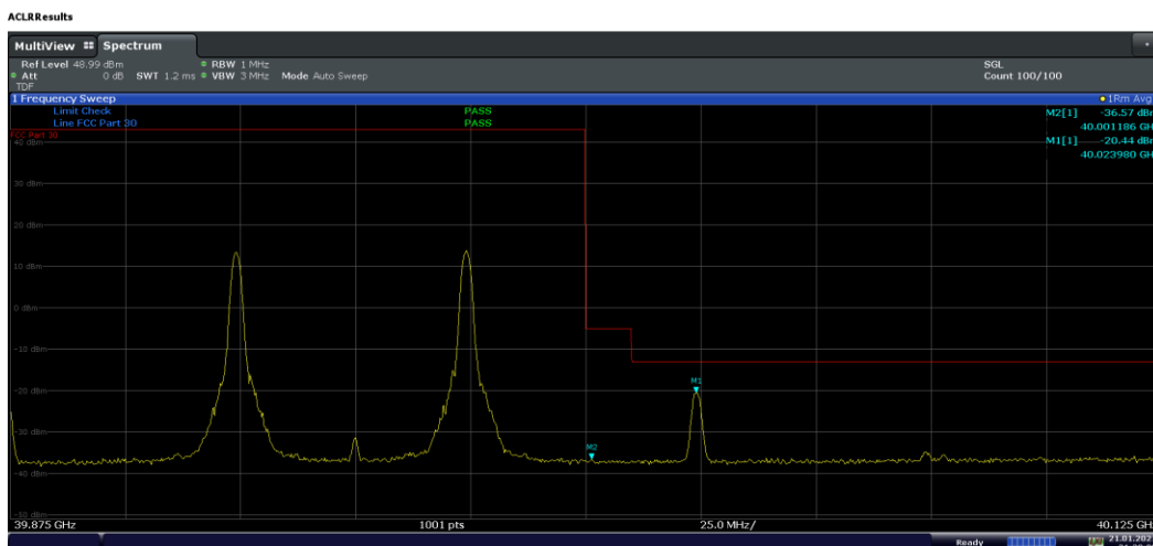
Plot 7-325. Ant M0 Upper BE (Band n260-50+50MHz-2CC SISO Dual Pol – QPSK 1-M RB)
