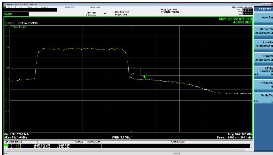
Plot 7-295. Ant M3 Upper BE (Band n261-50MHz-1CC SISO Dual Pol- QPSK Full RB)
