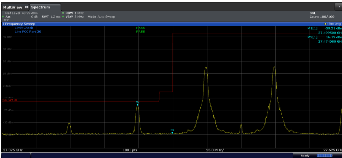
Plot 7-273. Ant M2 Lower BE (Band n261-50+50MHz-2CC SISO Dual Pol – QPSK 1-M RB)
