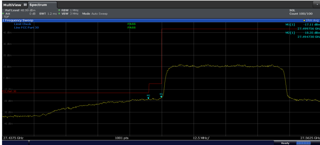
Plot 7-269. Ant M2 Lower BE (Band n261-50MHz-1CC SISO DFTs-OFDM – QPSK Full RB)
