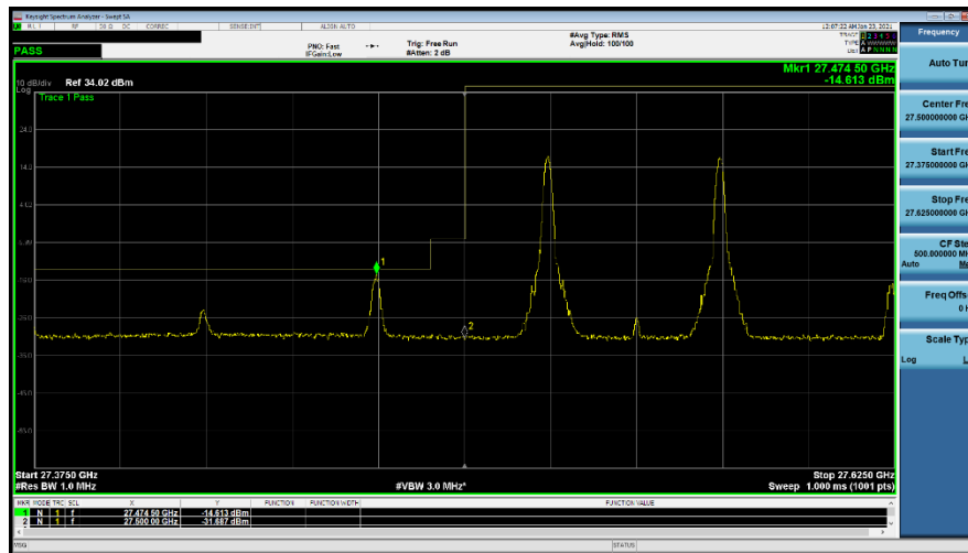
Plot 7-297. Ant M3 Lower BE (Band n261-50+50MHz-2CC SISO CP-OFDM - QPSK 1-M RB)
