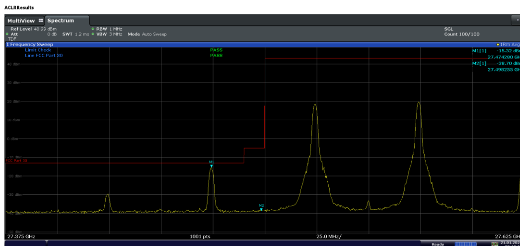
Plot 7-250. Ant M0 Lower BE (Band n261-50+50MHz-2CC SISO Dual Pol – \pi/2 BPSK 1-M RB)
