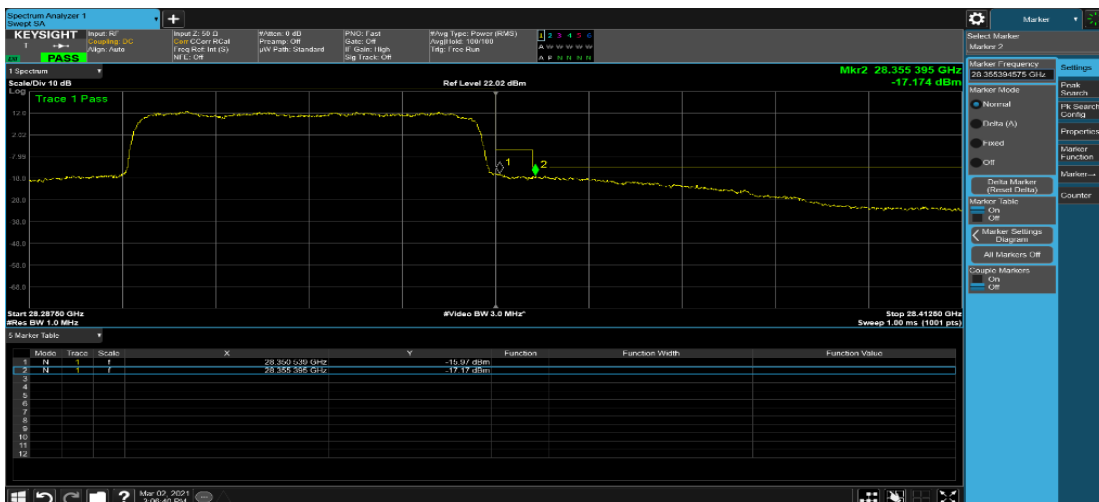
Plot 7-271. Ant M2 Upper BE (Band n261-50MHz-1CC SISO Dual Pol – QPSK Full RB)
