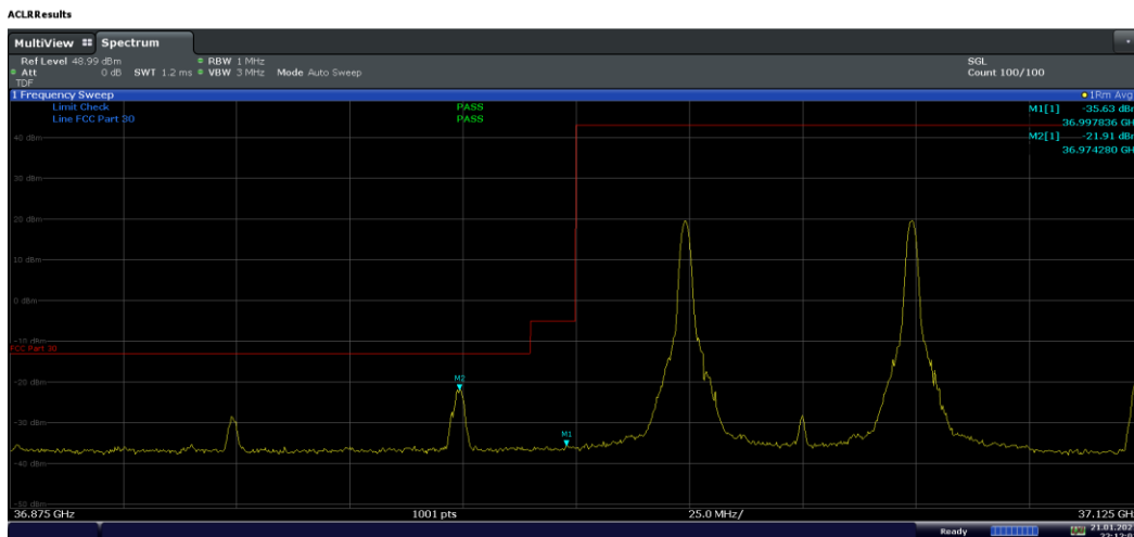
Plot 7-322. Ant M0 Lower BE (Band n260-50+50MHz-2CC SISO Dual Pol - \pi/2 BPSK 1-M RB)
