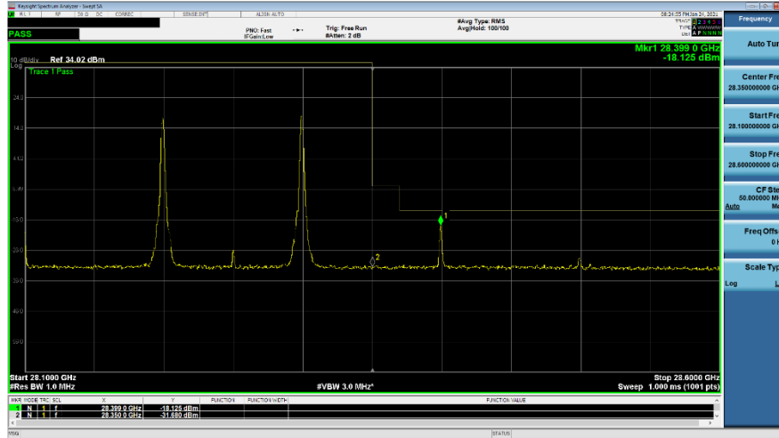
Plot 7-314. Ant M3 Upper BE (Band n261-100+100MHz-2CC SISO Dual Pol- \pi/2 BPSK 1-M RB)
