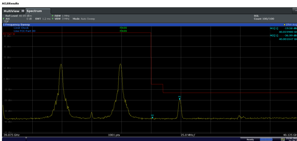
Plot 7-327. Ant M0 Upper BE (Band n260-50+50MHz-2CC SISO Dual Pol – 16QAM 1-M RB)
