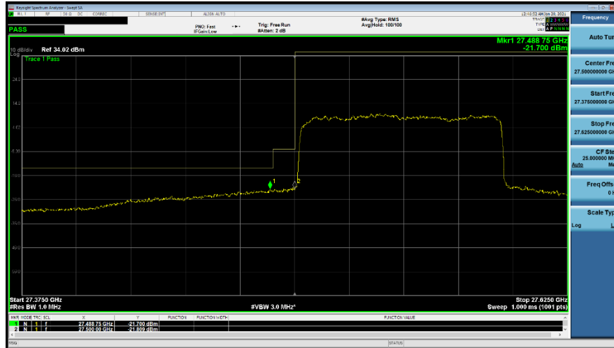
Plot 7-305. Ant M3 Lower BE (Band n261-100MHz-1CC SISO DFTs-OFDM – QPSK Full RB)
