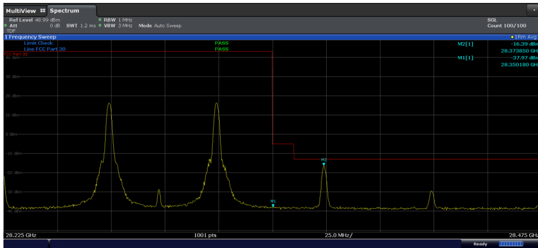
Plot 7-279. Ant M2 Upper BE (Band n261-50+50MHz-2CC SISO Dual Pol – 16QAM 1-M RB)
