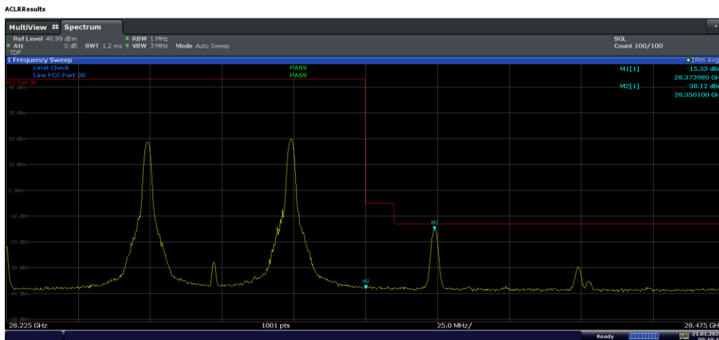
Plot 7-253. Ant M0 Upper BE (Band n261-50+50MHz-2CC SISO Dual Pol – QPSK 1-M RB)
