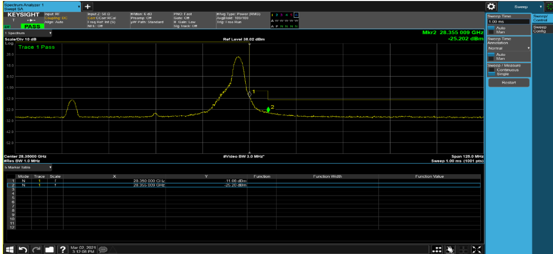
Plot 7-272. Ant M2 Upper BE (Band n261-50MHz-1CC SISO Dual Pol – QPSK 1-H RB)
