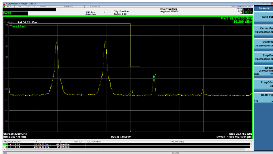
Plot 7-304. Ant M3 Upper BE (Band n261-50+50MHz-2CC SISO Dual Pol- 64QAM 1-M RB)
