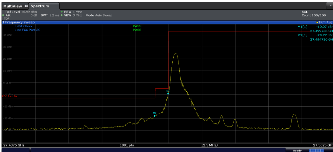
Plot 7-270. Ant M2 Lower BE (Band n261-50MHz-1CC SISO DFTs-OFDM – QPSK 1-L RB)
