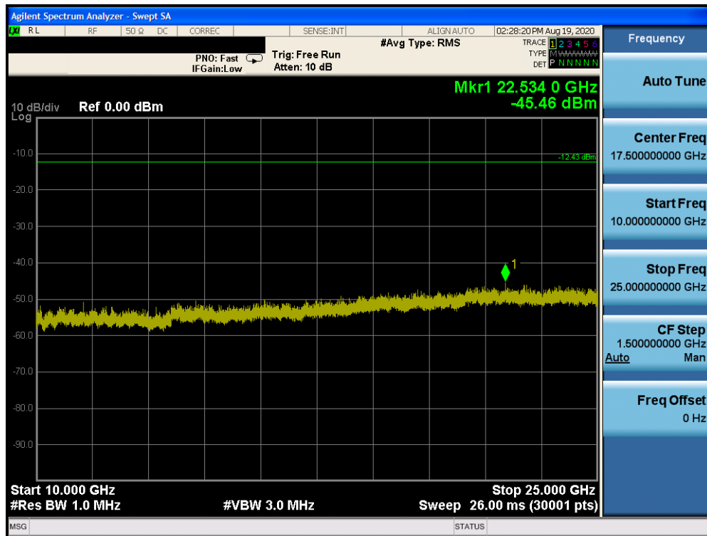
Plot 7-14. Conducted Spurious Plot (Bluetooth (LE), 1Mbps, iPA – Ch. 39)
