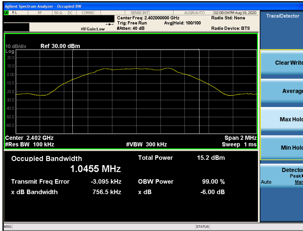
Plot 7-1. 6dB Bandwidth Plot (Bluetooth (LE), 1Mbps, iPA – Ch. 0)
