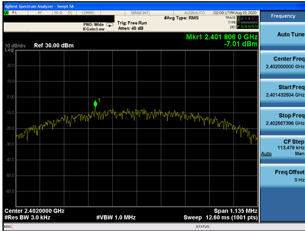
Plot 7-4. Power Spectral Density Plot (Bluetooth (LE), 1Mbps, iPA – Ch. 0)
