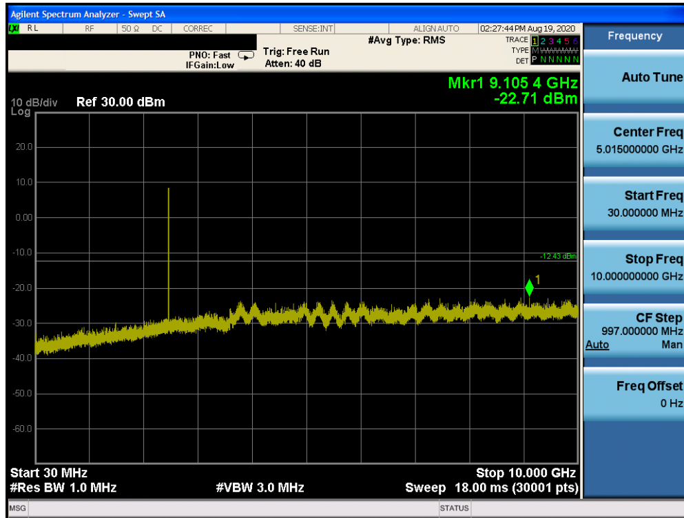
Plot 7-13. Conducted Spurious Plot (Bluetooth (LE), 1Mbps, iPA – Ch. 39)
