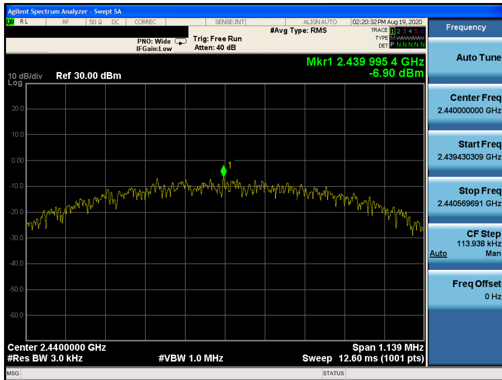
Plot 7-5. Power Spectral Density Plot (Bluetooth (LE), 1Mbps, iPA – Ch. 19)
