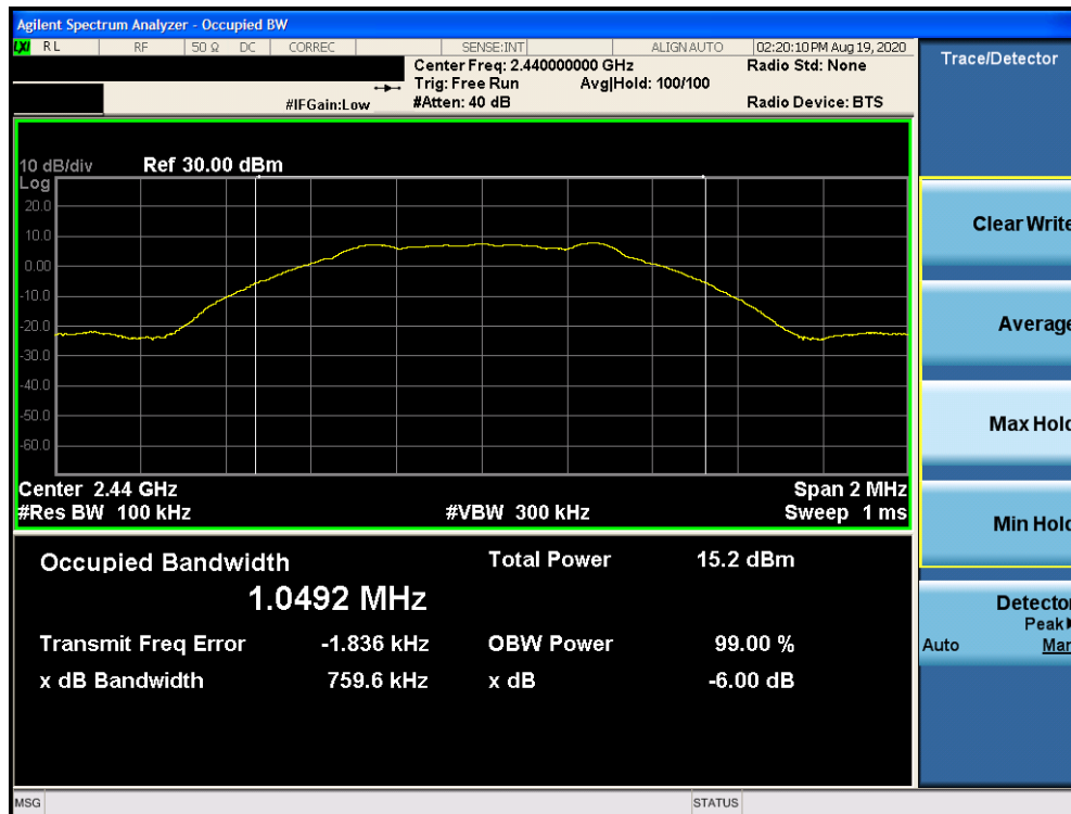
Plot 7-2. 6dB Bandwidth Plot (Bluetooth (LE), 1Mbps, iPA – Ch. 19)
