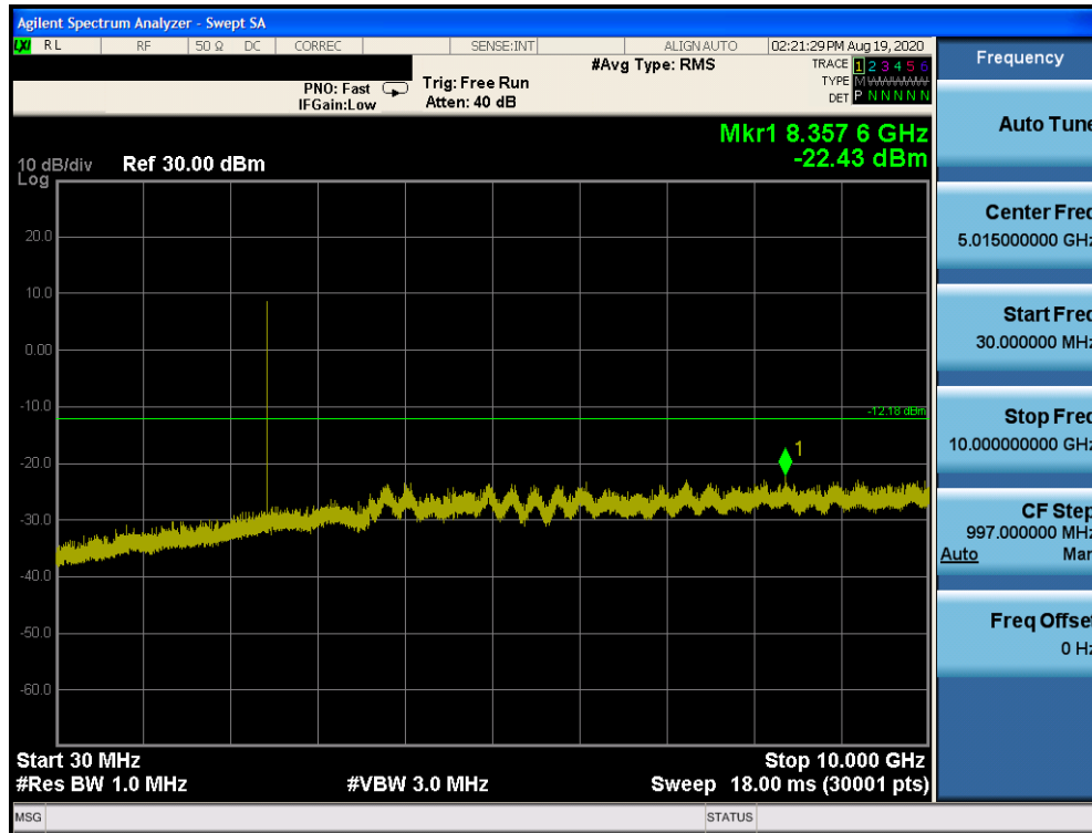
Plot 7-11. Conducted Spurious Plot (Bluetooth (LE), 1Mbps, iPA – Ch. 19)
