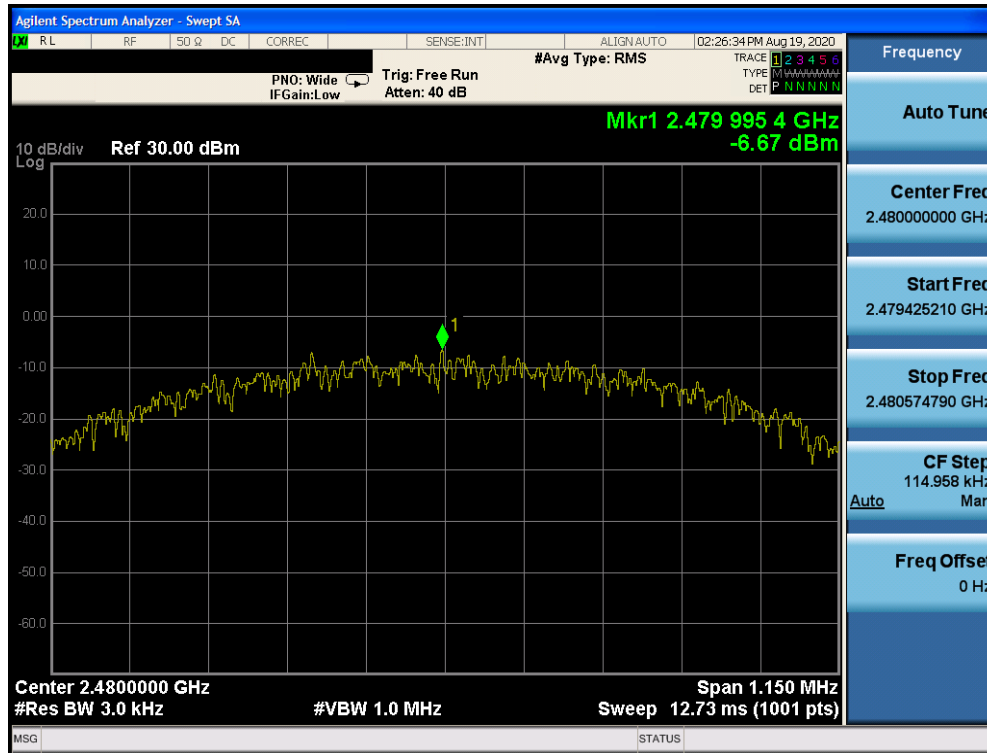
Plot 7-6. Power Spectral Density Plot (Bluetooth (LE), 1Mbps, iPA – Ch. 39)
