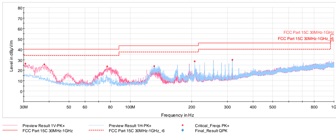
Plot 7-26. Radiated Spurious Emissions 30MHz-1GHz (1Mbps, iPA – Ch.19, with AC/DC Adapter)
