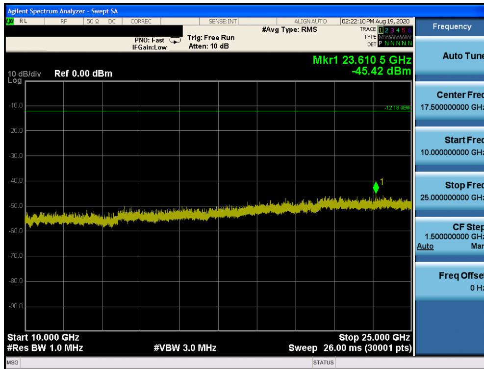
Plot 7-12. Conducted Spurious Plot (Bluetooth (LE), 1Mbps, iPA – Ch. 19)
