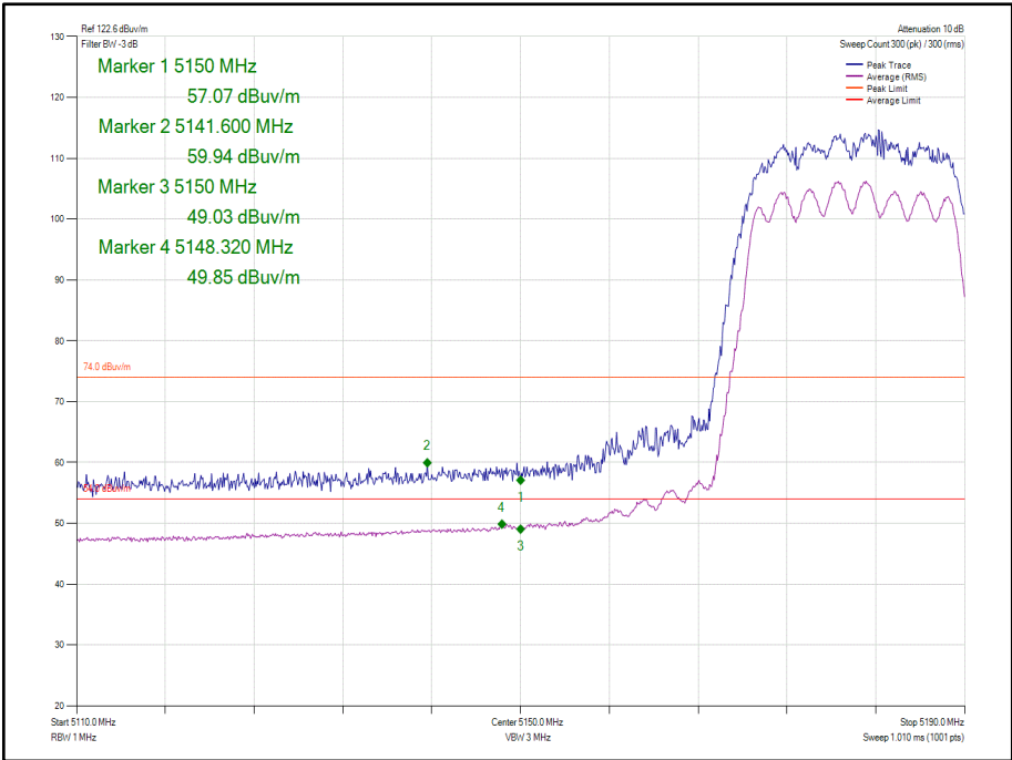
Figure 425 - 802.11n HT20 CDD Cores 0-1 - 5180 MHz Band Edge Frequency 5150 MHz
