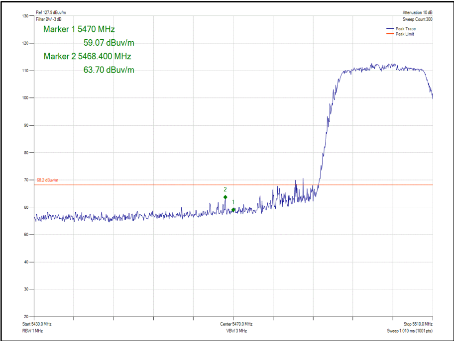
Figure 380 - 802.11n HT20 Core 0 - 5500 MHz Band Edge Frequency 5470 MHz
