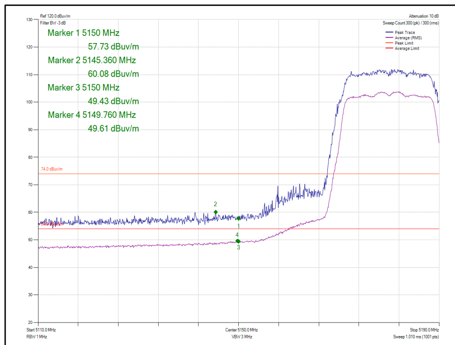
Figure 420 - 802.11n HT20 Core 0 - 5180 MHz Band Edge Frequency 5150 MHz
