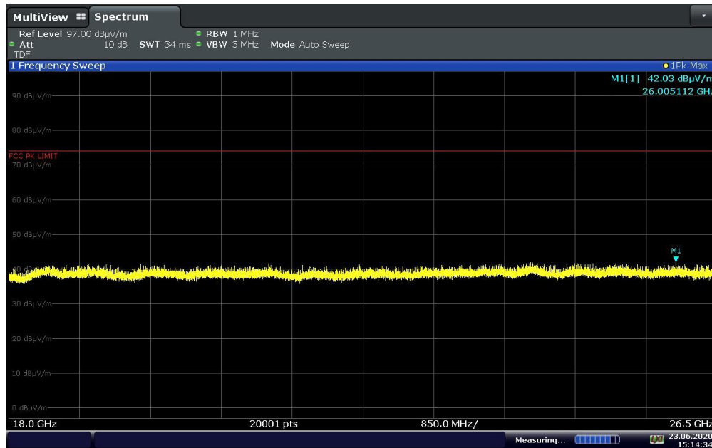
Plot 7-33. Radiated Spurious Emissions above 18GHz (GFSK ePA – Ch. 39, Pol. V)
