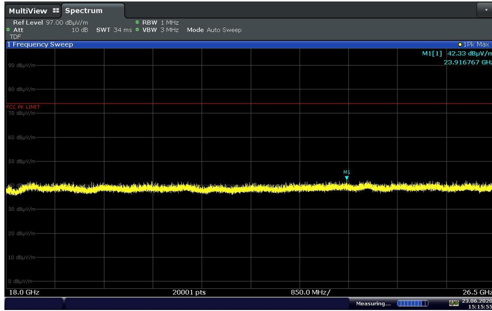
Plot 7-32. Radiated Spurious Emissions above 18GHz (GFSK ePA – Ch. 39, Pol. H)
