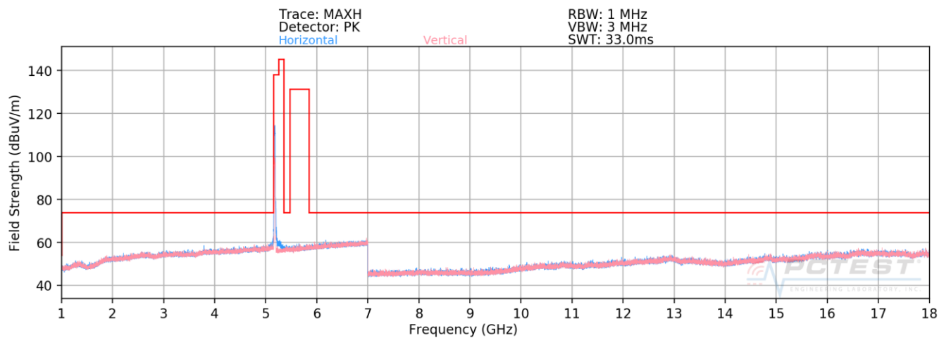
Plot 7-185. Radiated Spurious Plot above 1GHz SISO CORE1 (802.11n – U1 Ch. 36)
