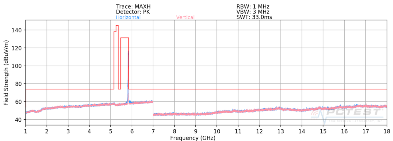
Plot 7-184. Radiated Spurious Plot above 1GHz SISO CORE0 (802.11n – U3 Ch. 165)
