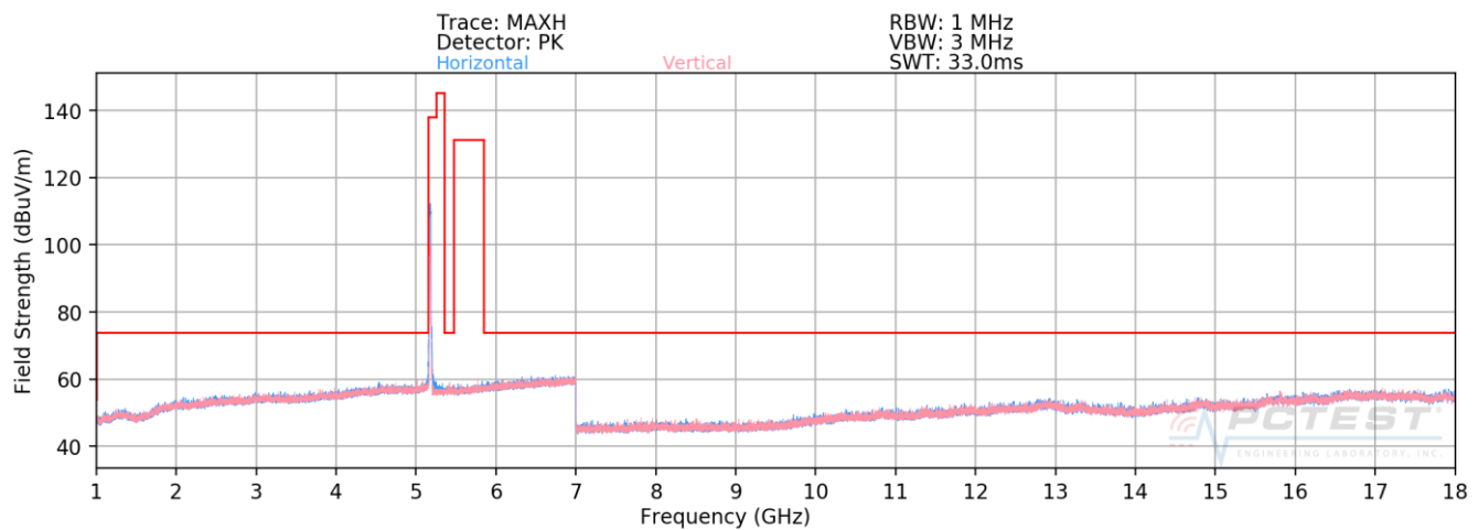
Plot 7-173. Radiated Spurious Plot above 1GHz SISO CORE0 (802.11n – U1 Ch. 36)
