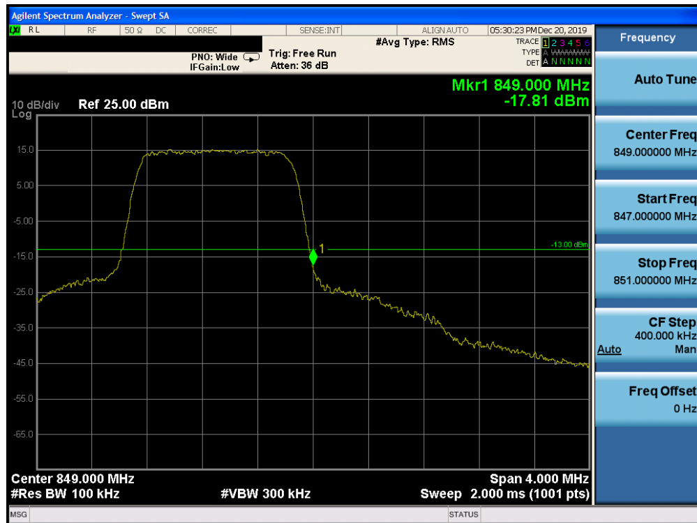
Plot 7-198. Upper Band Edge Plot (Band 5 – 1.4MHz QPSK – RB Size 6)
