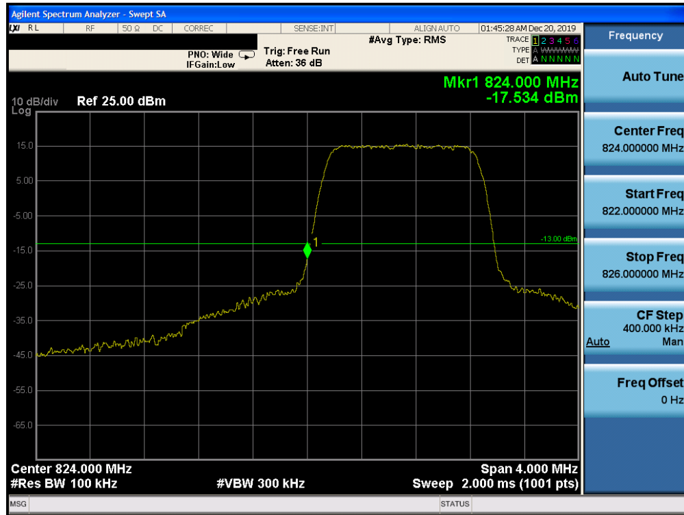
Plot 7-197. Lower Band Edge Plot (Band 5 – 1.4MHz QPSK – RB Size 6)
