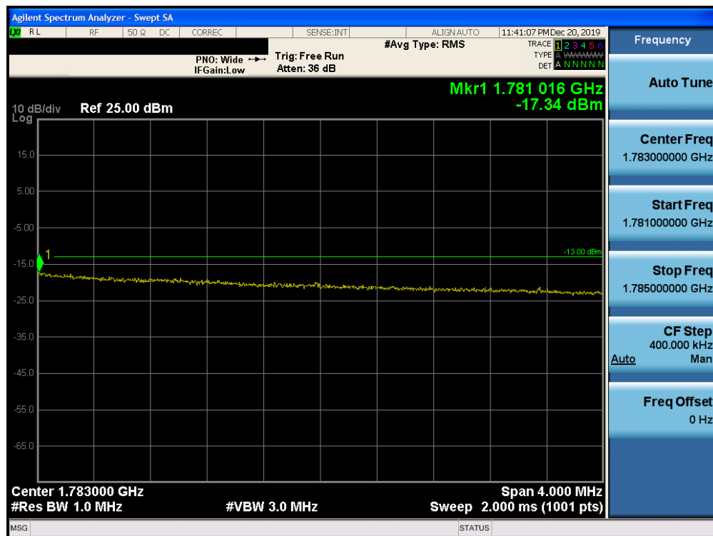
Plot 7-244. Upper Extended Band Edge Plot (Band 66 – 10.0MHz QPSK – RB Size 50)
