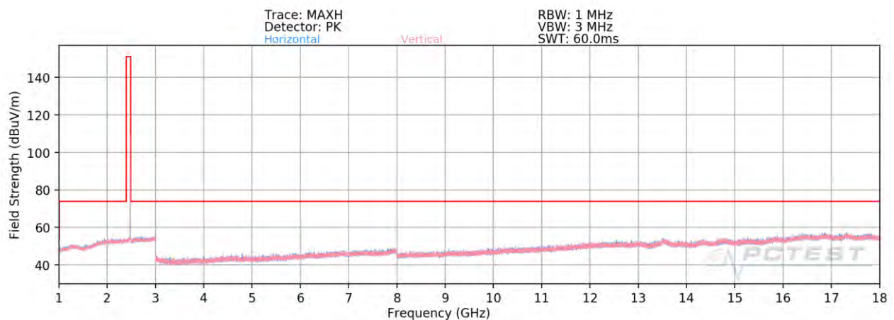
Plot 7-86. Radiated Spurious Plot Above 1GHz Ant 2a (4Mbps, HDR4 ePA – Ch. 75, Ant. Pol. H & V)
