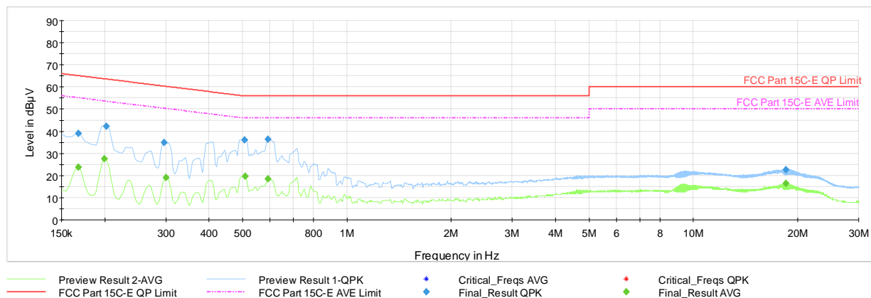
Plot 7-81. Line-Conducted Test Plot- Ch.39 TxBF (L1, with AC/DC Adapter)
