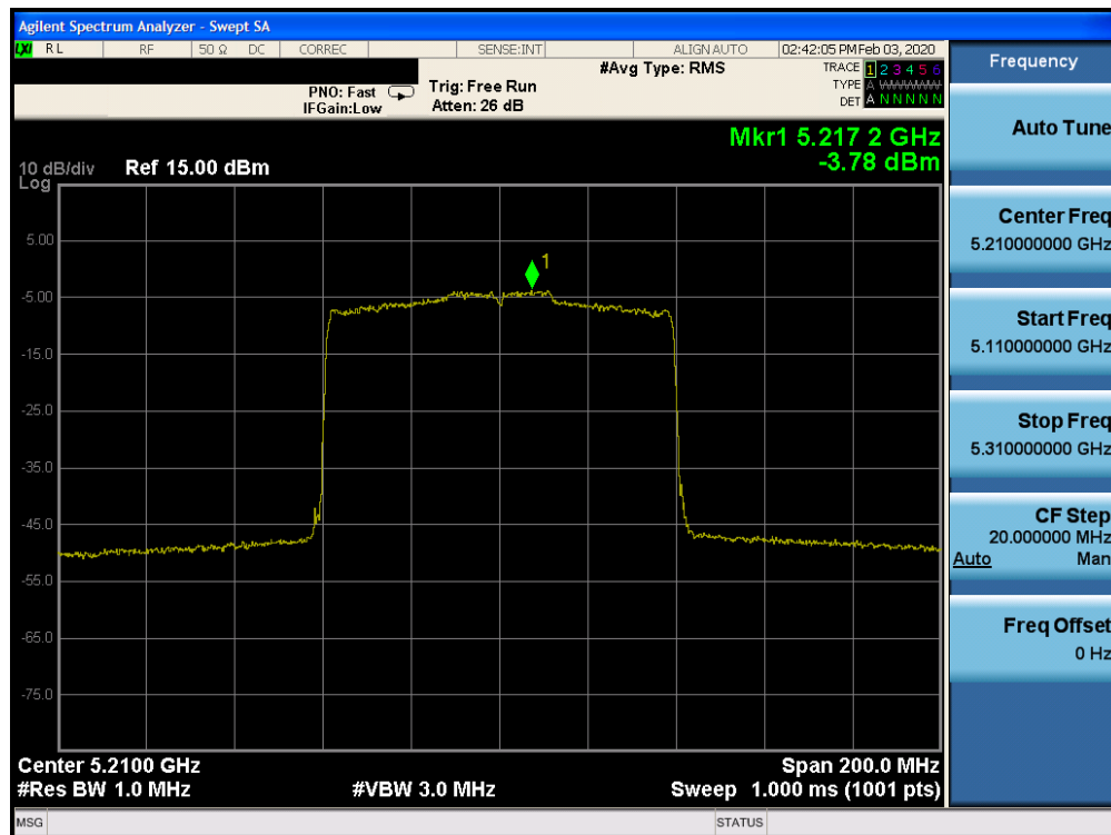
Plot 7-672. Power Spectral Density Plot ISCED CDD CORE 1 (80MHz BW 802.11ax – RU996 (UNII Band 1) – Ch. 42)
