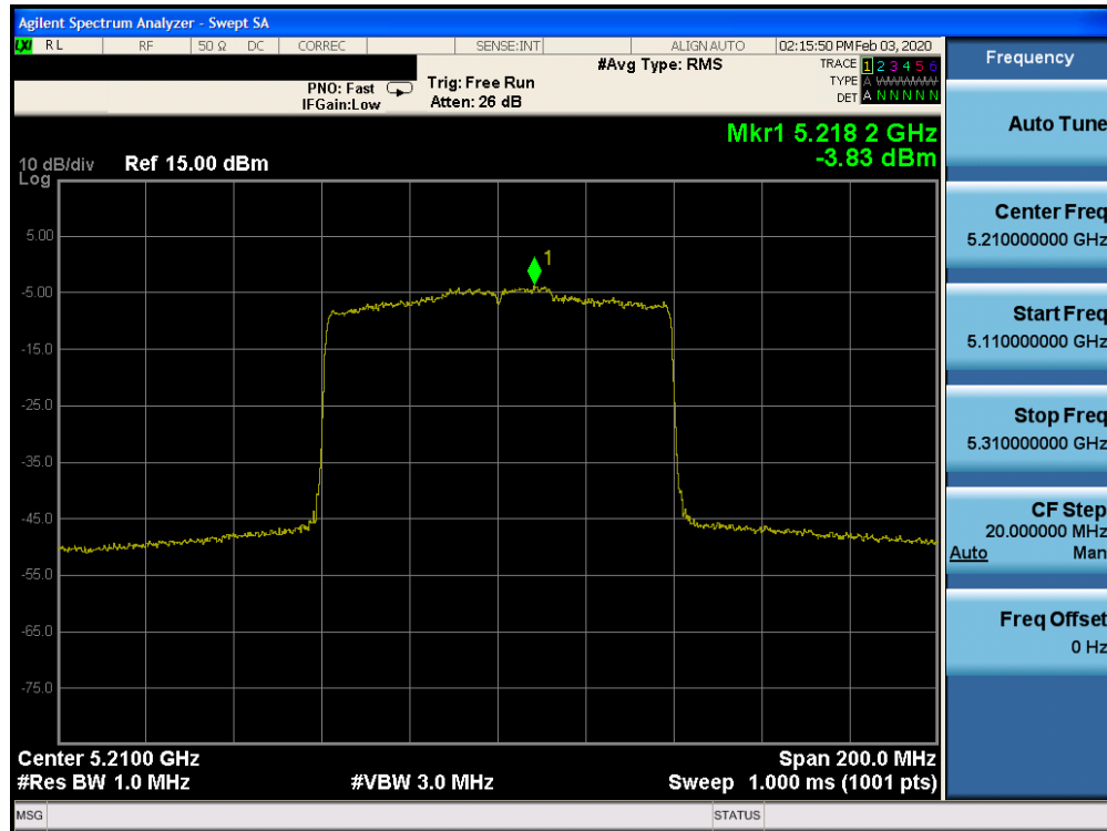
Plot 7-671. Power Spectral Density Plot ISCED CDD CORE 0 (80MHz BW 802.11ax – RU996 (UNII Band 1) – Ch. 42)
