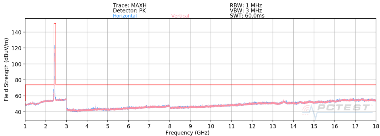
Plot 7-135. Radiated Spurious Plot above 1GHz CDD (802.11ax OFDMA – RU26 – Ch. 1)
