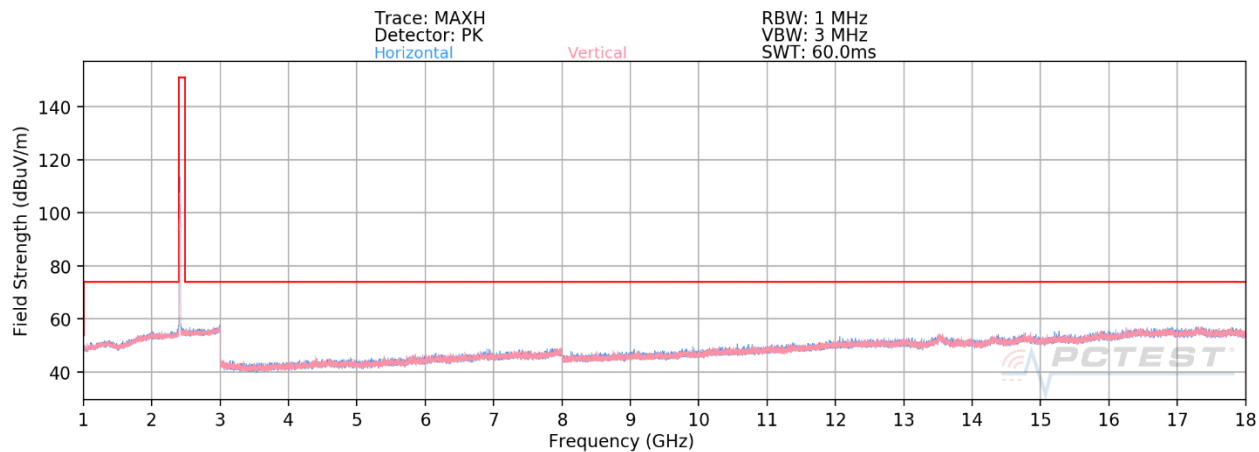
Plot 7-123. Radiated Spurious Plot above 1GHz SISO CORE 0 (802.11ax OFDMA – RU26 – Ch. 1)
