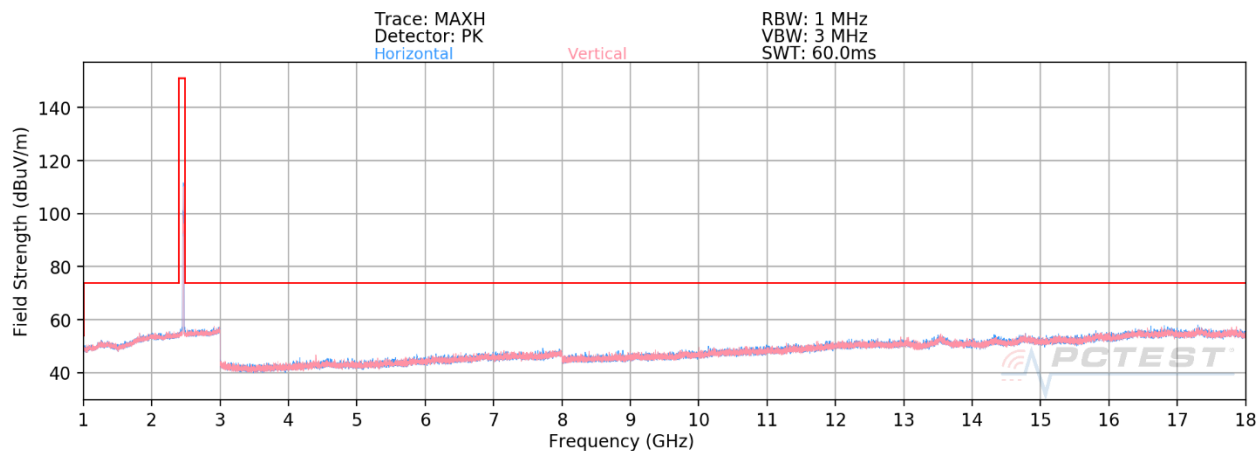
Plot 7-131. Radiated Spurious Plot above 1GHz SISO CORE 1 (802.11ax OFDMA – RU26 – Ch. 11)
