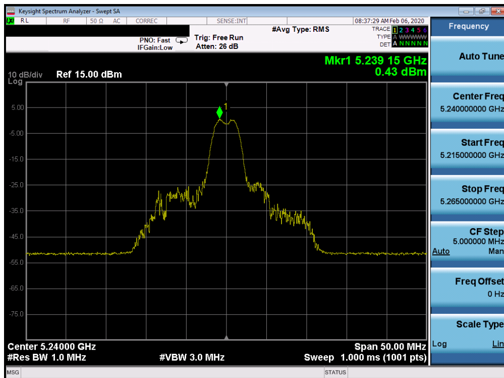
Plot 7-613. Power Spectral Density Plot ISED CDD CORE 1 (20MHz BW 802.11ax Index 4 – RU26 (UNII Band 1) – Ch. 48)
