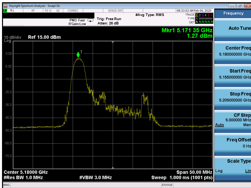
Plot 7-599. Power Spectral Density Plot ISCED CDD CORE 1 (20MHz BW 802.11ax Index 0 – RU26 (UNII Band 1) – Ch. 36)
