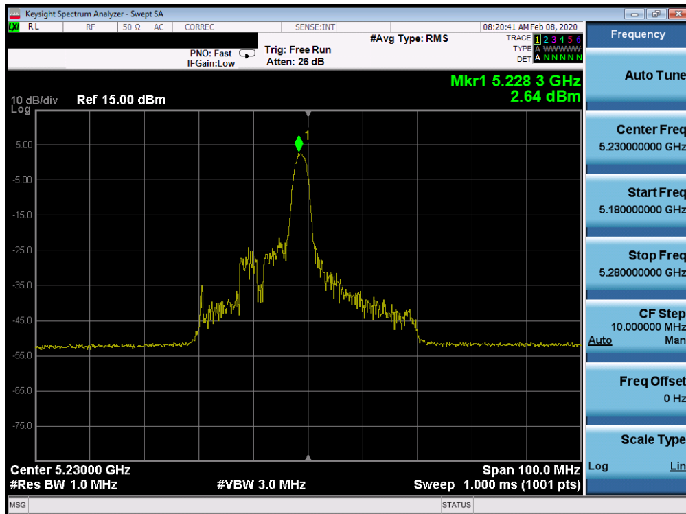
Plot 7-631. Power Spectral Density Plot ISED CDD CORE 1 (40MHz BW 802.11ax Index 8 – RU26 (UNII Band 1) – Ch. 46)
