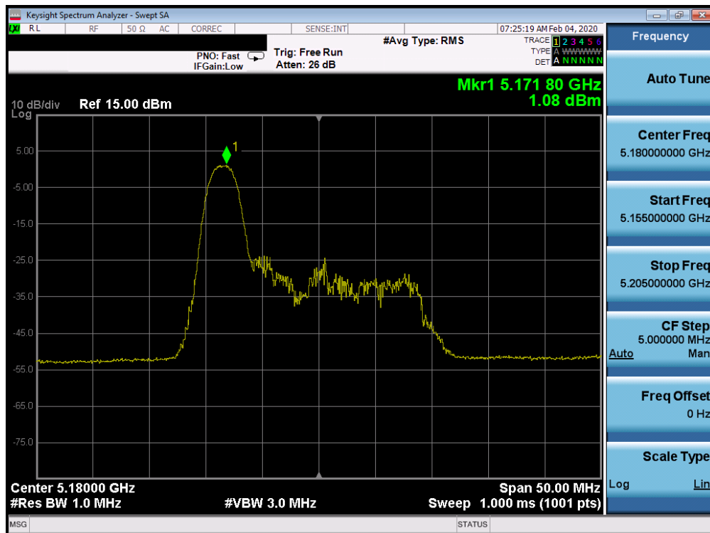
Plot 7-598. Power Spectral Density Plot ISCED CDD CORE 0 (20MHz BW 802.11ax Index 0 – RU26 (UNII Band 1) – Ch. 36)
