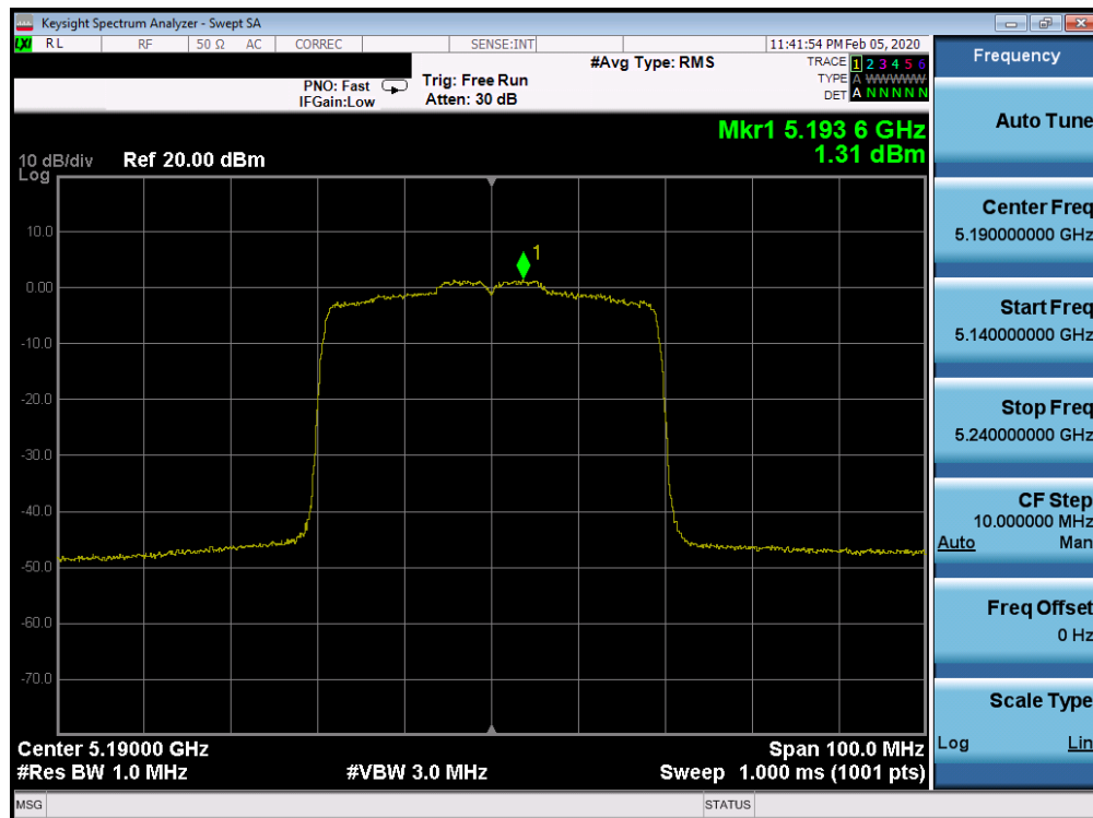
Plot 7-635. Power Spectral Density Plot ISCED CDD CORE 1 (40MHz BW 802.11ax – RU484 (UNII Band 1) – Ch. 38)
