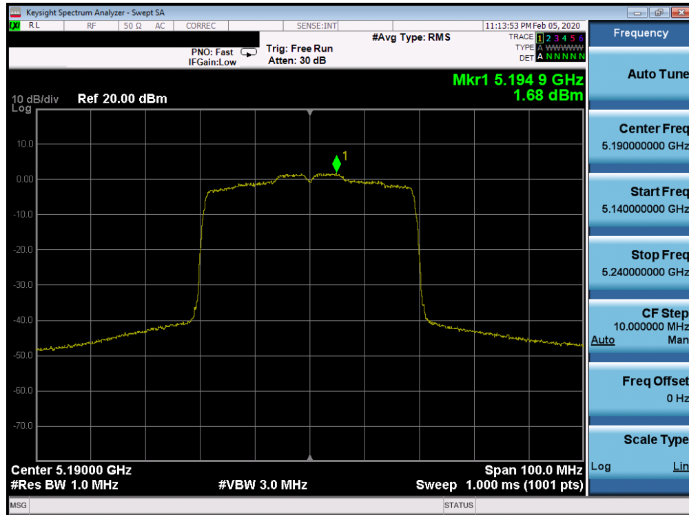
Plot 7-634. Power Spectral Density Plot ISCED CDD CORE 0 (40MHz BW 802.11ax – RU484 (UNII Band 1) – Ch. 38)
