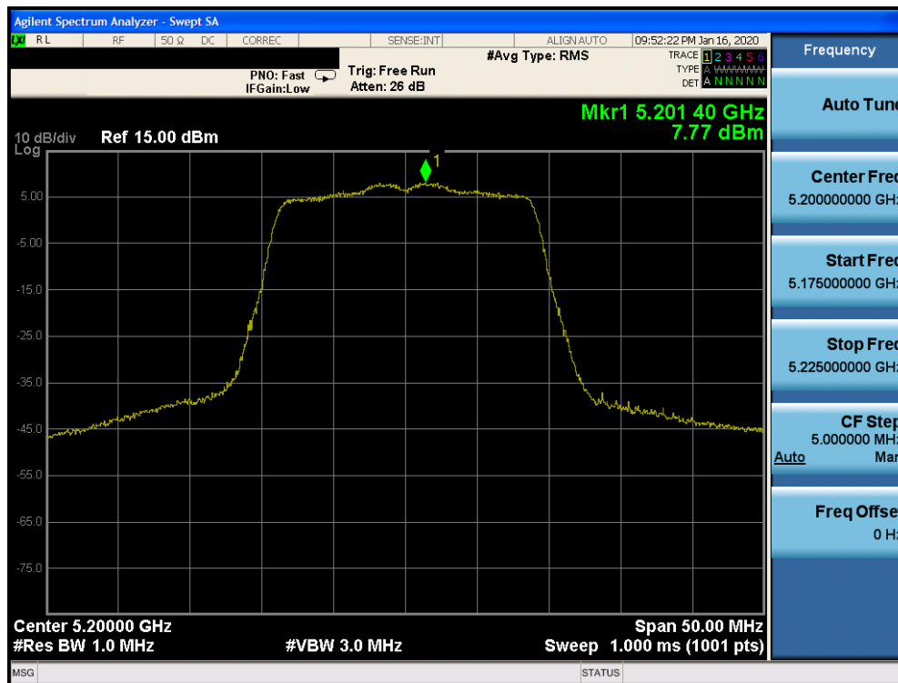
Plot 7-112. Power Spectral Density Plot CDD CORE 0 (20MHz BW 802.11n (UNII Band 1) – Ch. 40)
