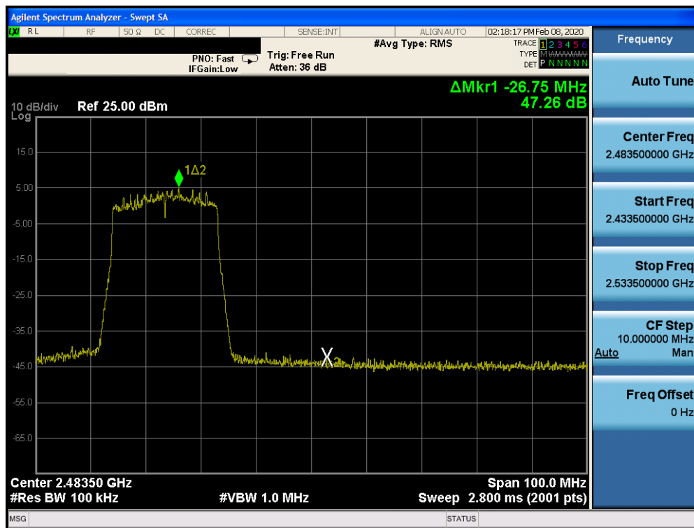
Plot 7-82. Band Edge SISO CORE 0 (802.11ax OFDMA – RU242 – Ch. 10)
