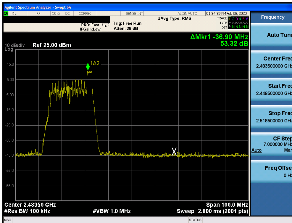
Plot 7-88. Band Edge SISO CORE 1 (802.11ax OFDMA – RU26 Index 8 – Ch. 10)
