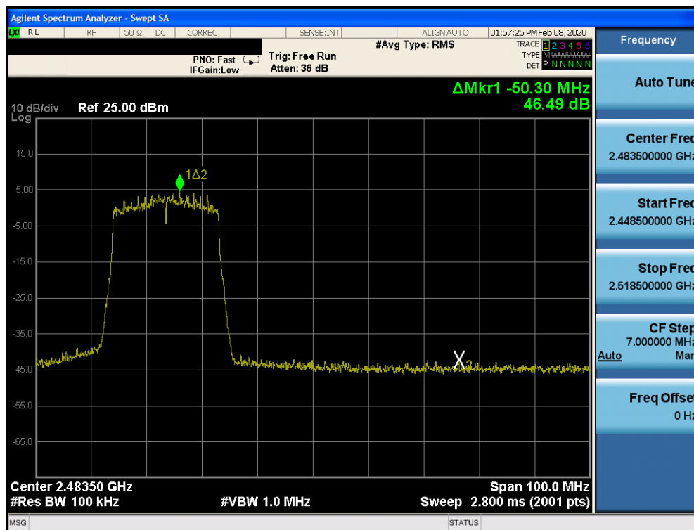
Plot 7-94. Band Edge SISO CORE 1 (802.11ax OFDMA – RU242 – Ch. 10)
