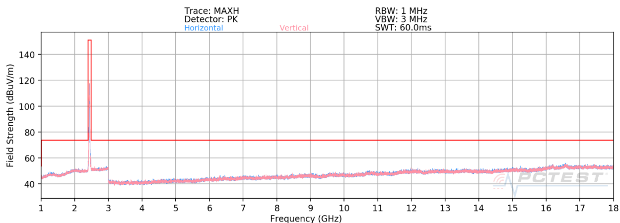
Plot 7-122. Radiated Spurious Plot above 1GHz SISO CORE 0 (802.11ax OFDMA – RU26 – Ch. 6)
