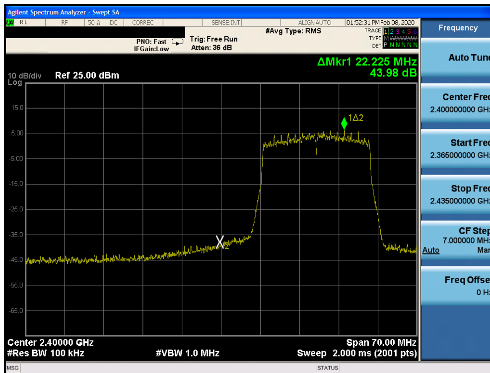
Plot 7-92. Band Edge SISO CORE 1 (802.11ax OFDMA – RU242 – Ch. 2)
