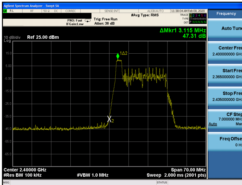
Plot 7-85. Band Edge SISO CORE 1 (802.11ax OFDMA – RU26 Index 0 – Ch. 1)
