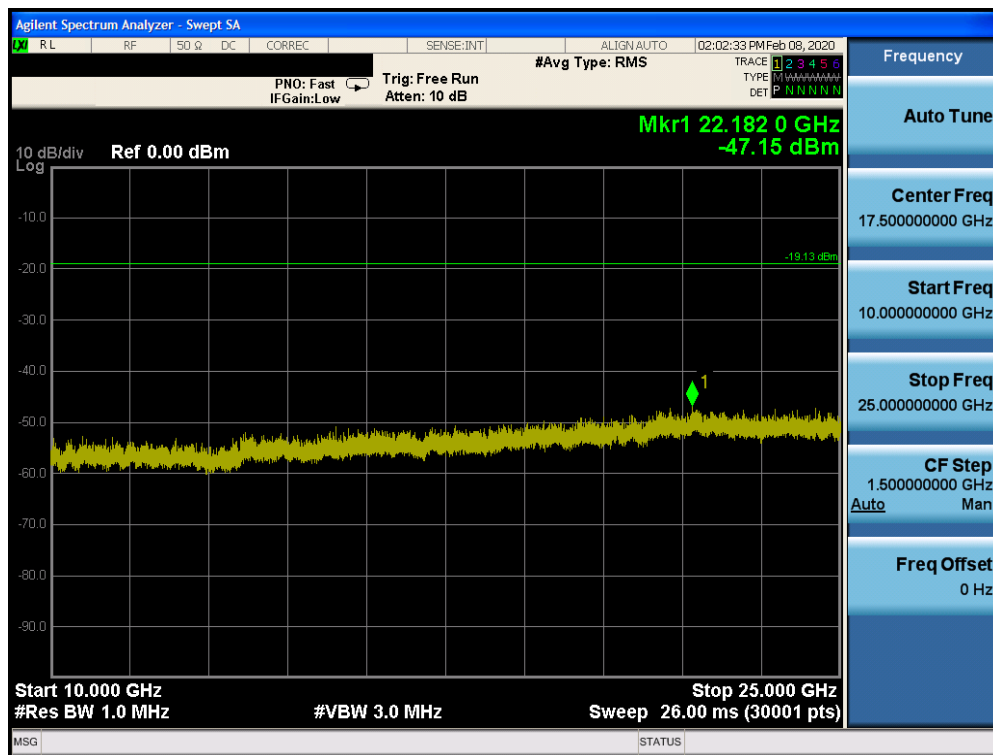
Plot 7-120. Conducted Spurious Plot SISO CORE 1 (802.11ax OFDMA – RU242 – Ch. 11)
