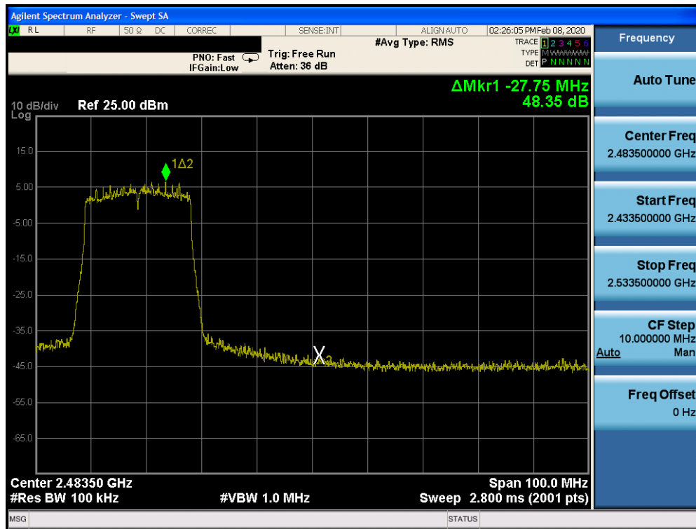
Plot 7-81. Band Edge SISO CORE 0 (802.11ax OFDMA – RU242 – Ch. 9)
