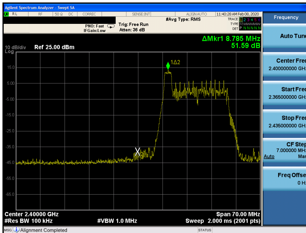
Plot 7-86. Band Edge SISO CORE 1 (802.11ax OFDMA – RU26 Index 0 – Ch. 2)
