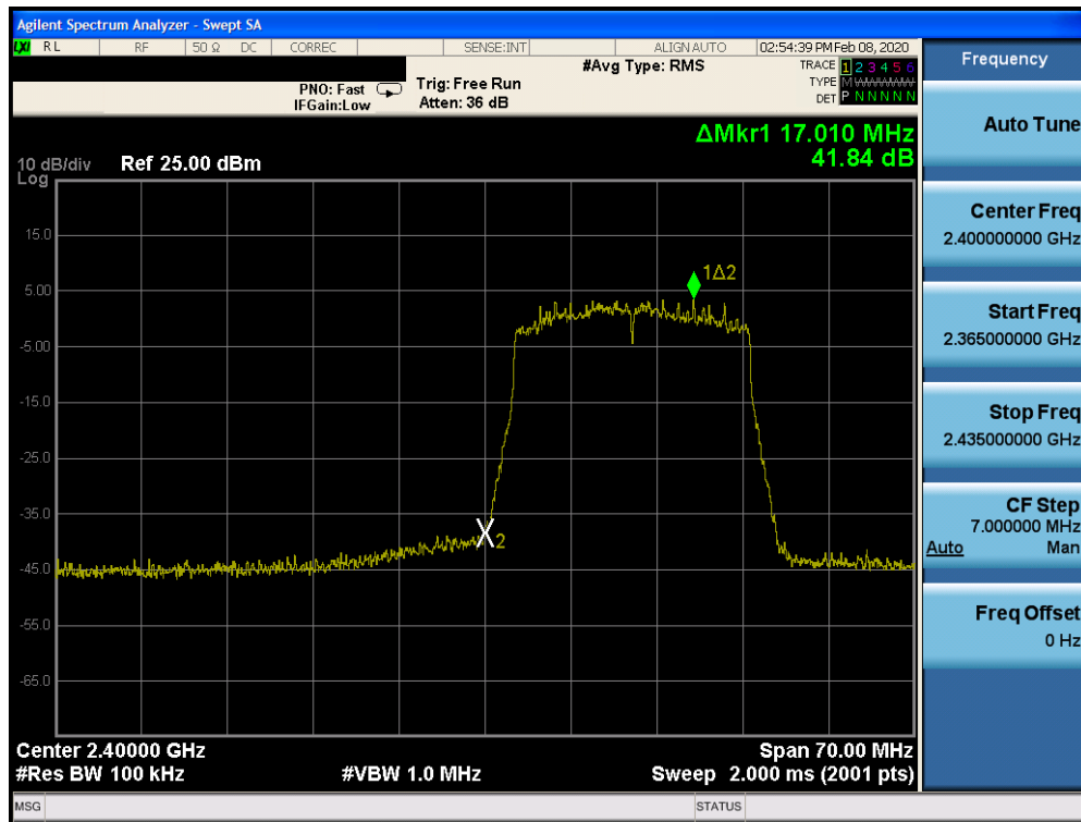
Plot 7-79. Band Edge SISO CORE 0 (802.11ax OFDMA - RU242 - Ch. 1)
