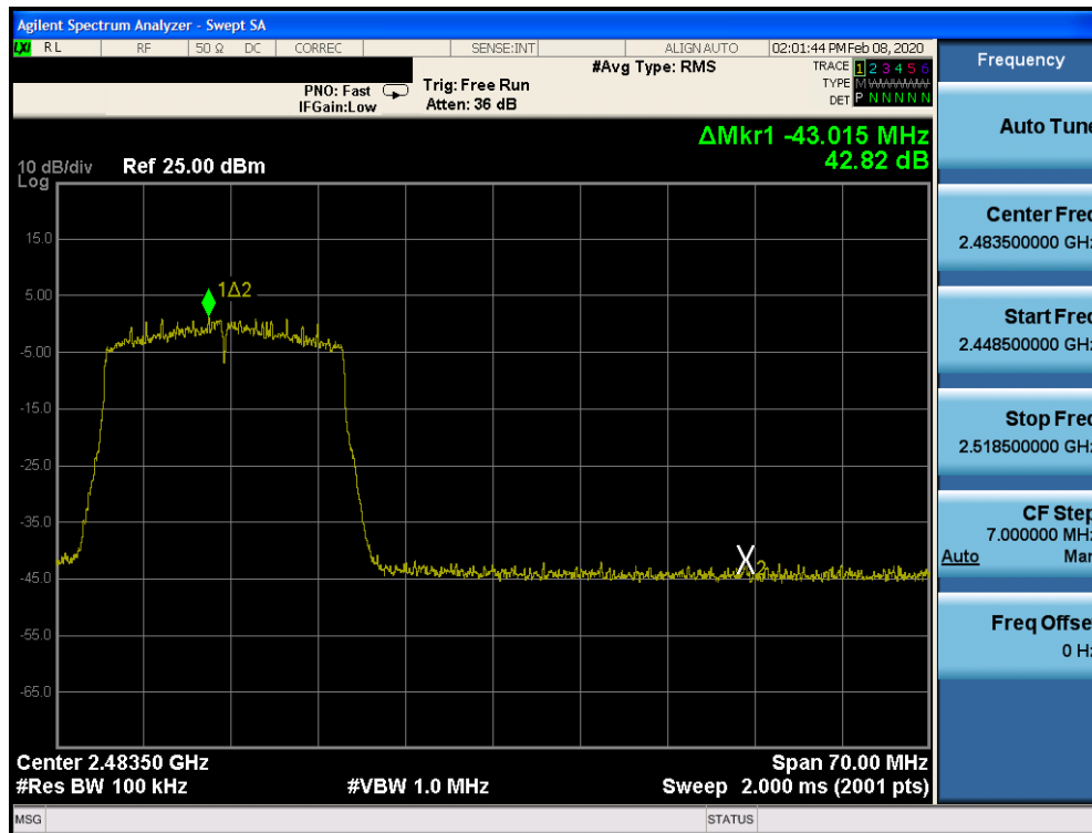
Plot 7-95. Band Edge SISO CORE 1 (802.11ax OFDMA – RU242 – Ch. 11)
