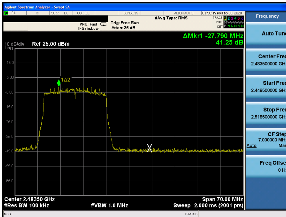
Plot 7-96. Band Edge SISO CORE 1 (802.11ax OFDMA – RU242 – Ch. 12)
