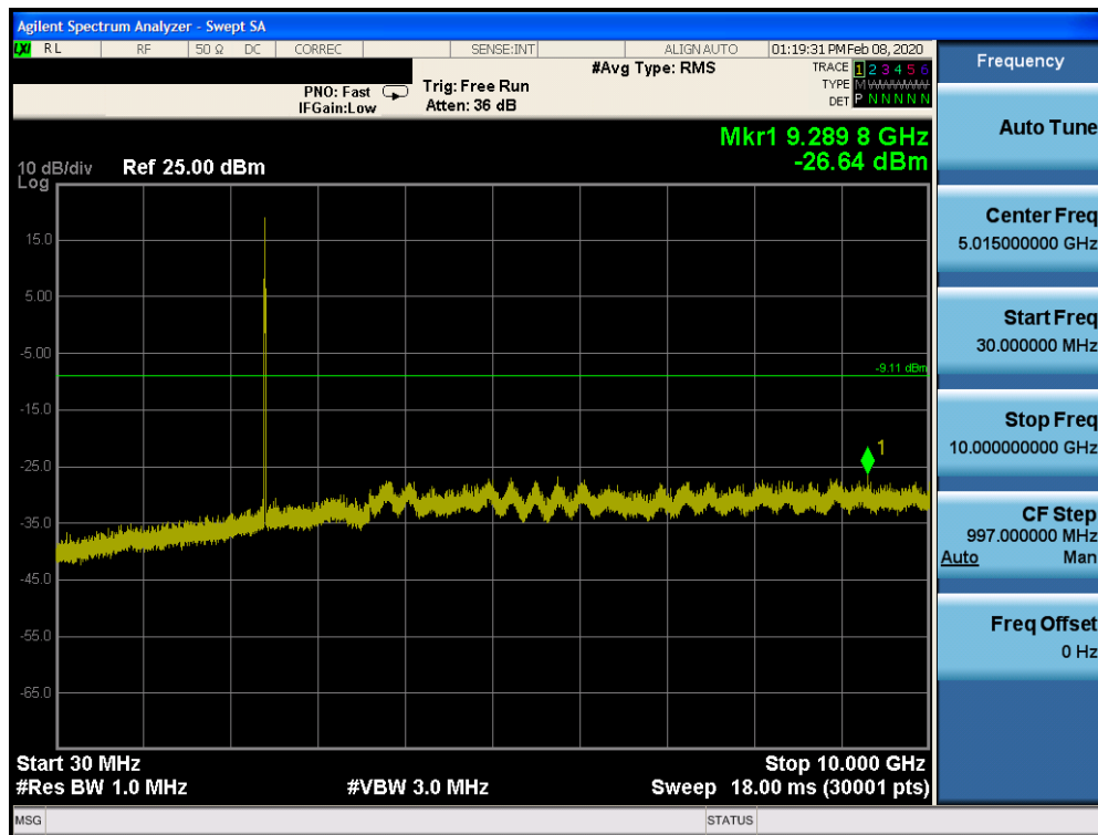
Plot 7-109. Conducted Spurious Plot SISO CORE 1 (802.11ax OFDMA – RU26 – Ch. 1)
