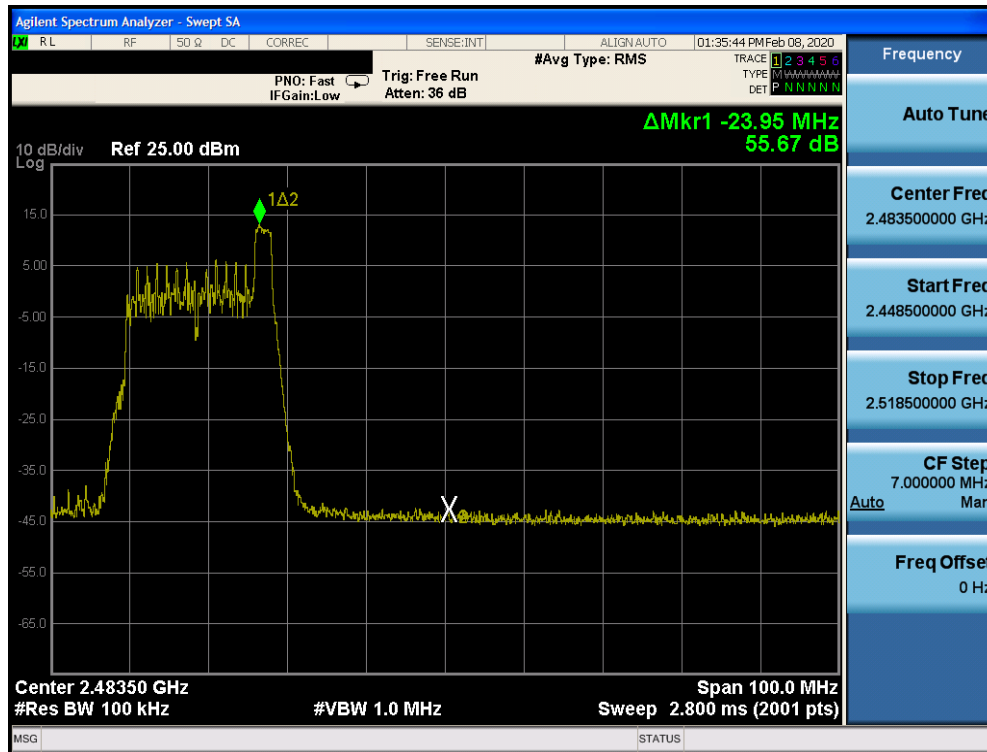
Plot 7-87. Band Edge SISO CORE 1 (802.11ax OFDMA – RU26 Index 8 – Ch. 9)
