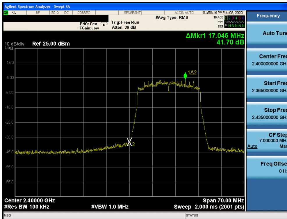
Plot 7-91. Band Edge SISO CORE 1 (802.11ax OFDMA – RU242 – Ch. 1)
