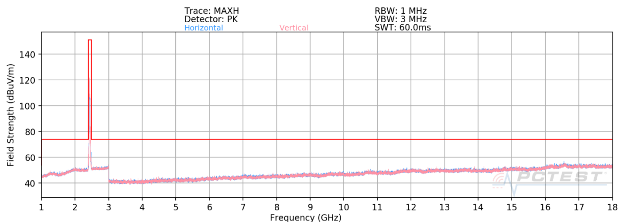
Plot 7-134. Radiated Spurious Plot above 1GHz CDD (802.11ax OFDMA – RU26 – Ch. 6)
