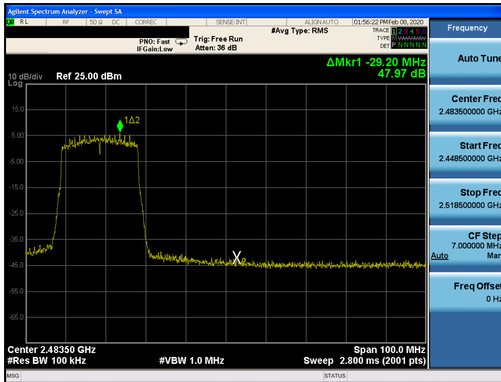
Plot 7-93. Band Edge SISO CORE 1 (802.11ax OFDMA – RU242 – Ch. 9)
