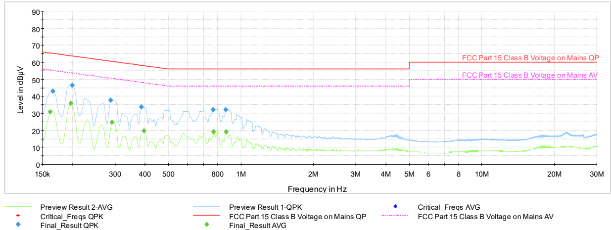
Plot 7-133. Line Conducted Plot with 802.11n CDD Ch.6 (N, with AC/DC Adapter)
