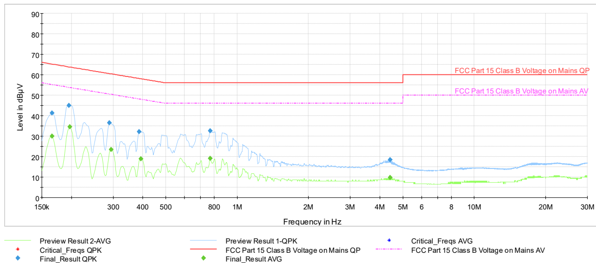
Plot 7-106. Line Conducted Plot with Bluetooth LE (N – 1Mbps, ePA, Ch.19 with AC/DC Adapter)
