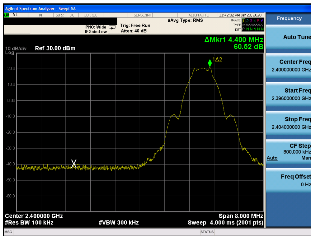
Plot 7-65. Band Edge Plot Ant WF7 (Bluetooth (LE), 1Mbps ePA – Ch. 0)
