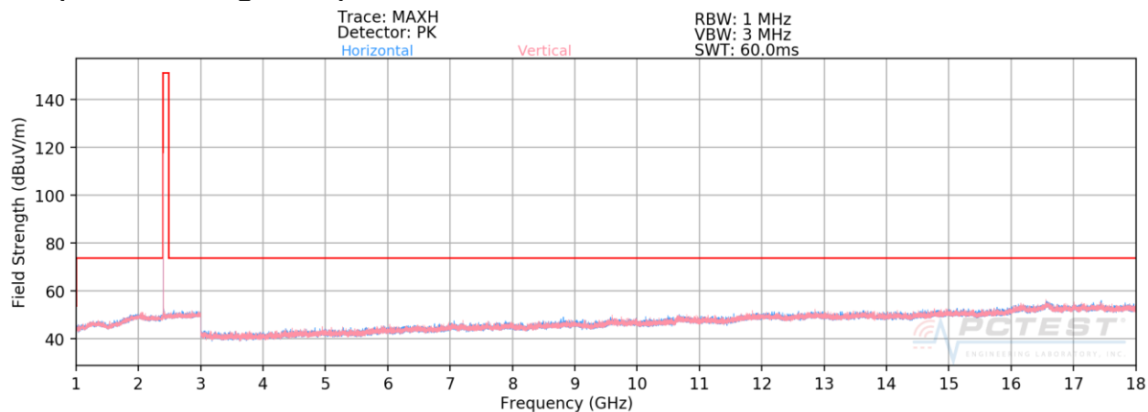
Plot 7-63. Radiated Spurious Plot above 1GHz TXBF (BT GFSK ePA – Ch. 0)
