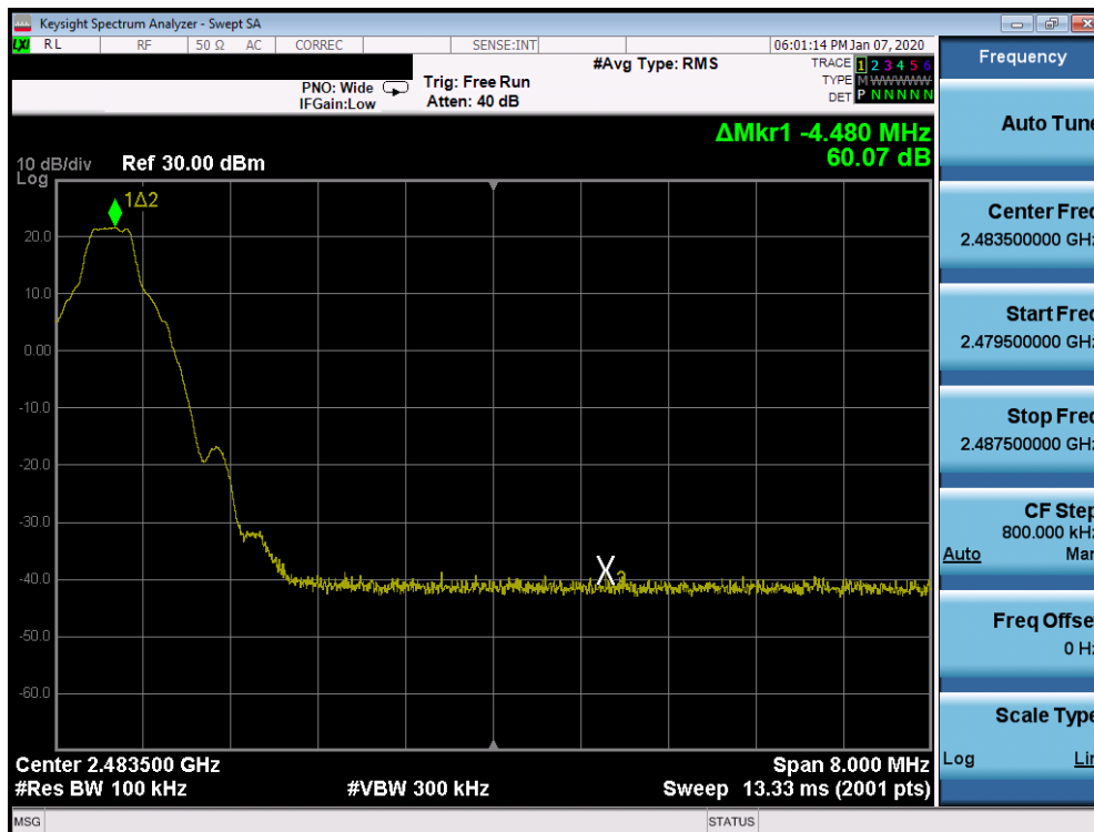
Plot 7-22. Band Edge Plot Ant WF7 (Bluetooth with Hopping Disabled, GFSK, ePA – Ch. 78)
