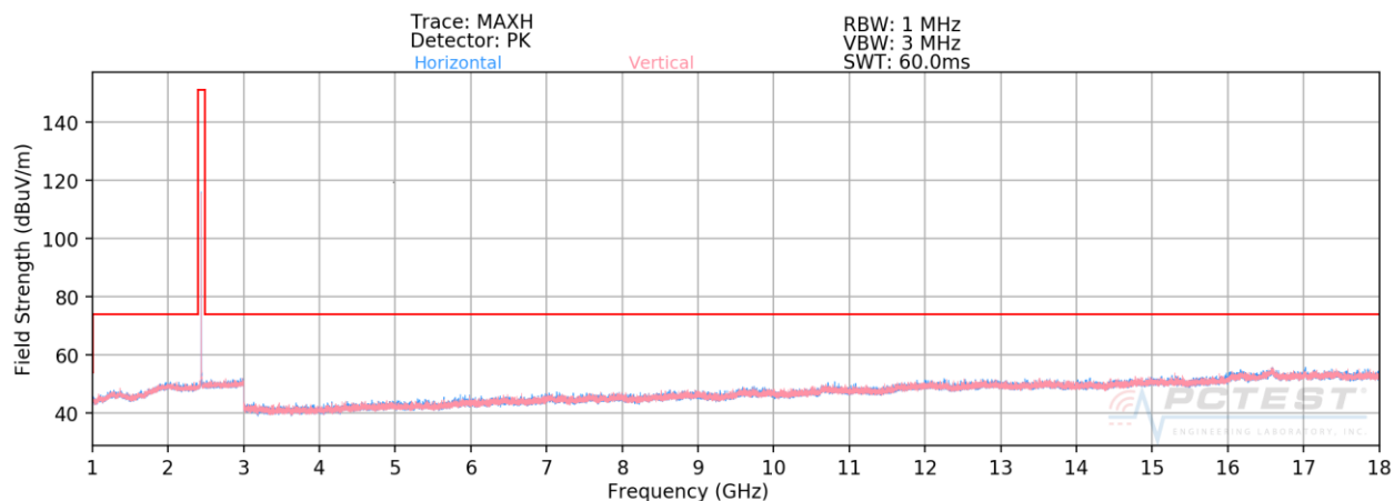
Plot 7-64. Radiated Spurious Plot above 1GHz TXBF (BT GFSK ePA – Ch. 39)
