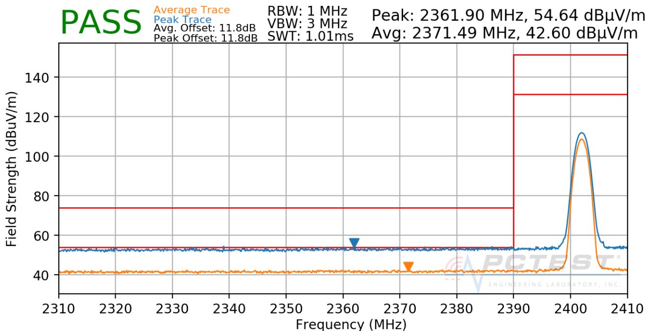
Plot 7-69. Radiated Restricted Lower Band Edge Measurement Ant WF8 (Average & Peak)
