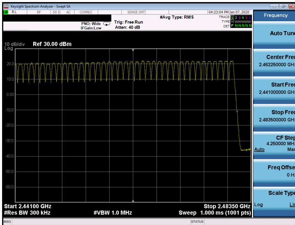
Plot 7-38. High End Spectrum Channel Hopping Plot Ant WF8 (Bluetooth, GFSK, ePA)
