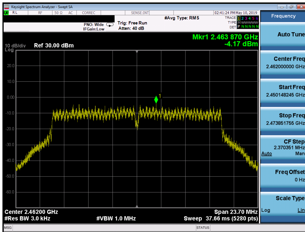
Plot 7-33. Power Spectral Density Plot SISO CORE 1 (802.11g – Ch. 11)
