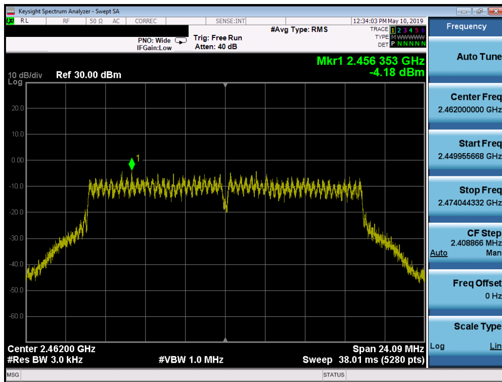
Plot 7-24. Power Spectral Density Plot SISO CORE 0 (802.11g – Ch. 11)
