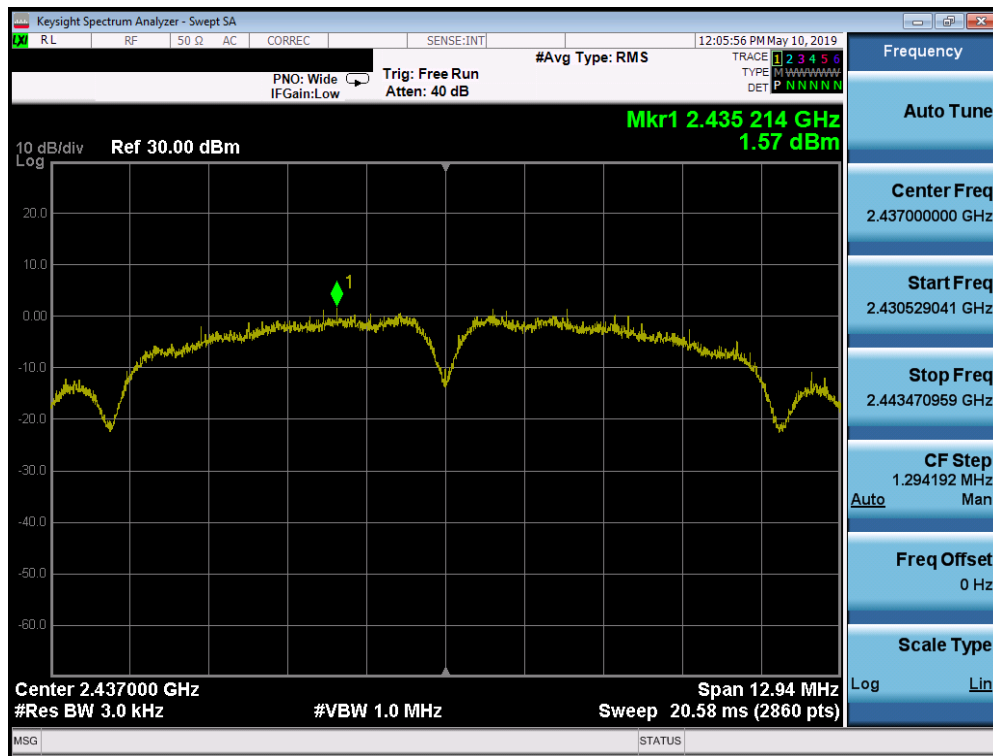
Plot 7-20. Power Spectral Density Plot SISO CORE 0 (802.11b – Ch. 6)
