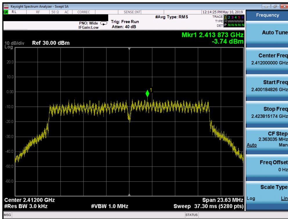
Plot 7-22. Power Spectral Density Plot SISO CORE 0 (802.11g – Ch. 1)
