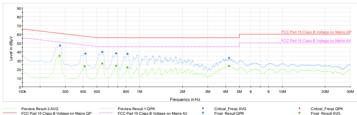
Plot 7-50. AC Line-Conducted Test Plot - Ch.39 (N, with AC/DC Adapter)
