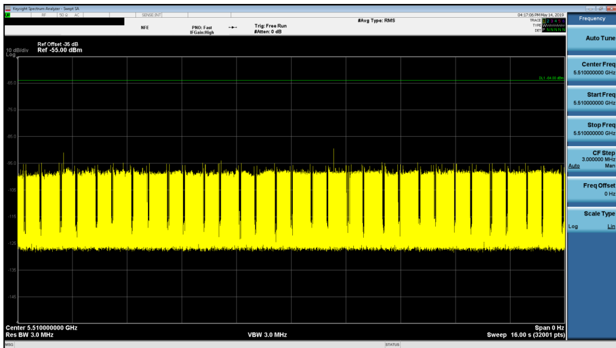
Figure 9-21. 5510MHz - Channel Loading - Mode 4 (40MHz)
