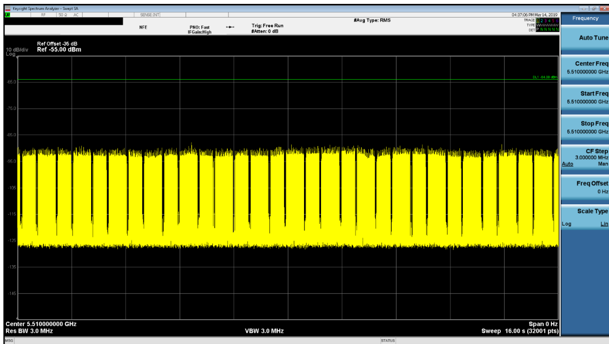
Figure 9-15. 5510MHz - Channel Loading - Mode 3 (40MHz)
