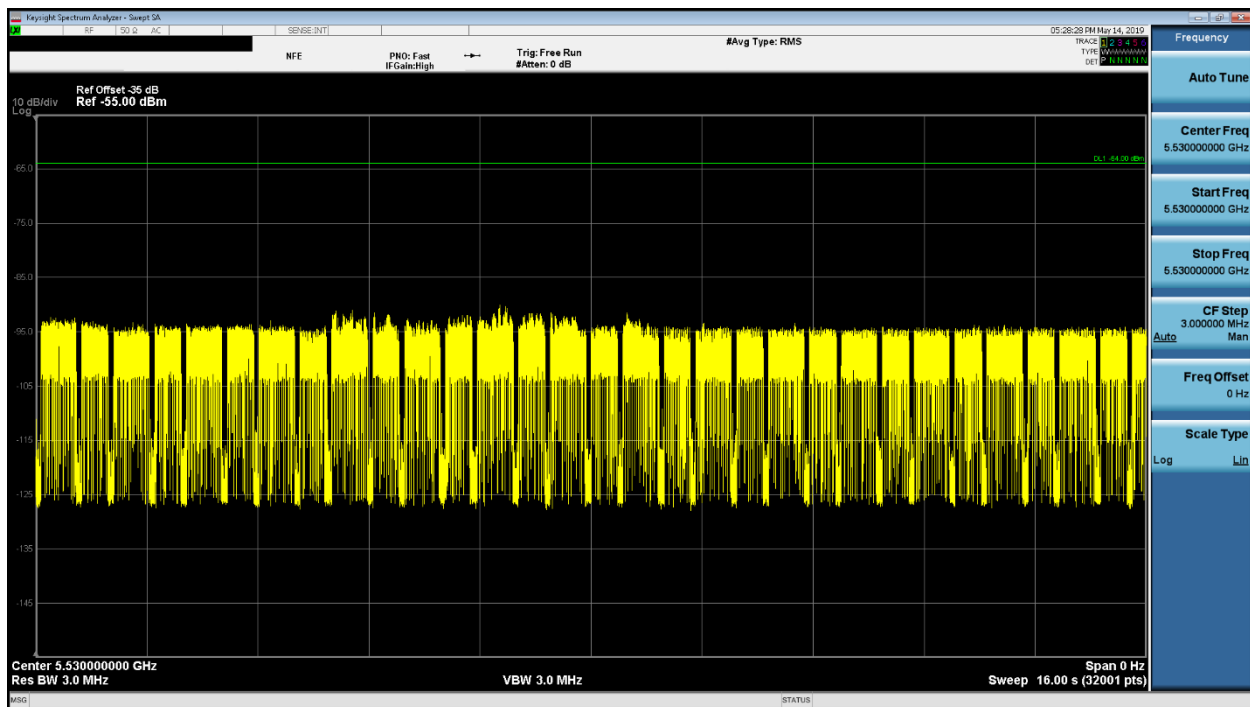
Figure 9-11. 5530MHz - Channel Loading - Mode 2 (80MHz)
