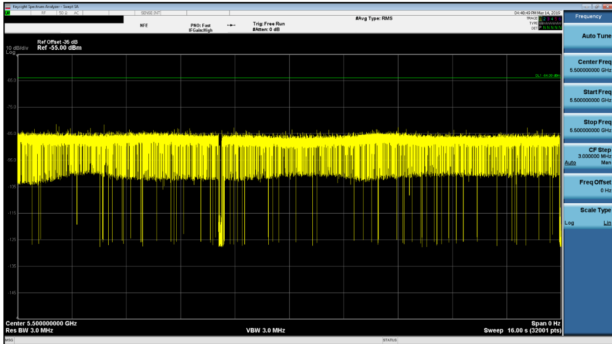
Figure 9-1. 5500MHz - Channel Loading - Mode 1 (20MHz)
