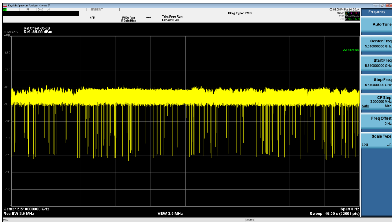
Figure 9-3. 5510MHz - Channel Loading - Mode 1 (40MHz)
