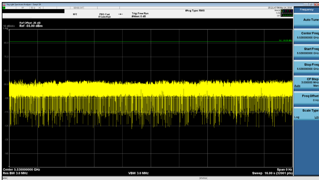
Figure 9-5. 5530MHz - Channel Loading - Mode 1 (80MHz)
