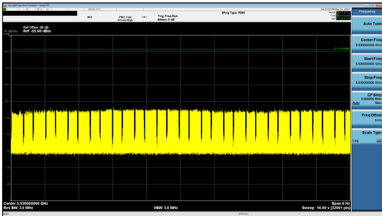
Figure 9-23. 5530MHz - Channel Loading - Mode 4 (80MHz)
