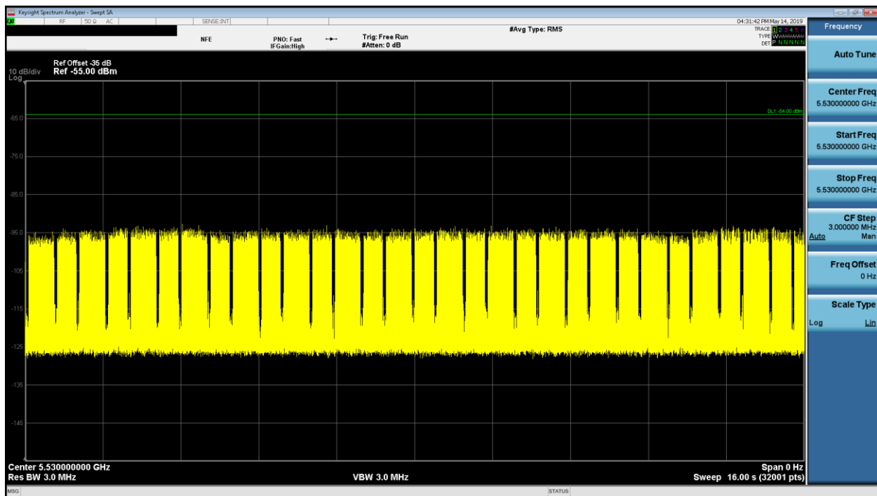
Figure 9-17. 5530MHz - Channel Loading - Mode 3 (80MHz)
