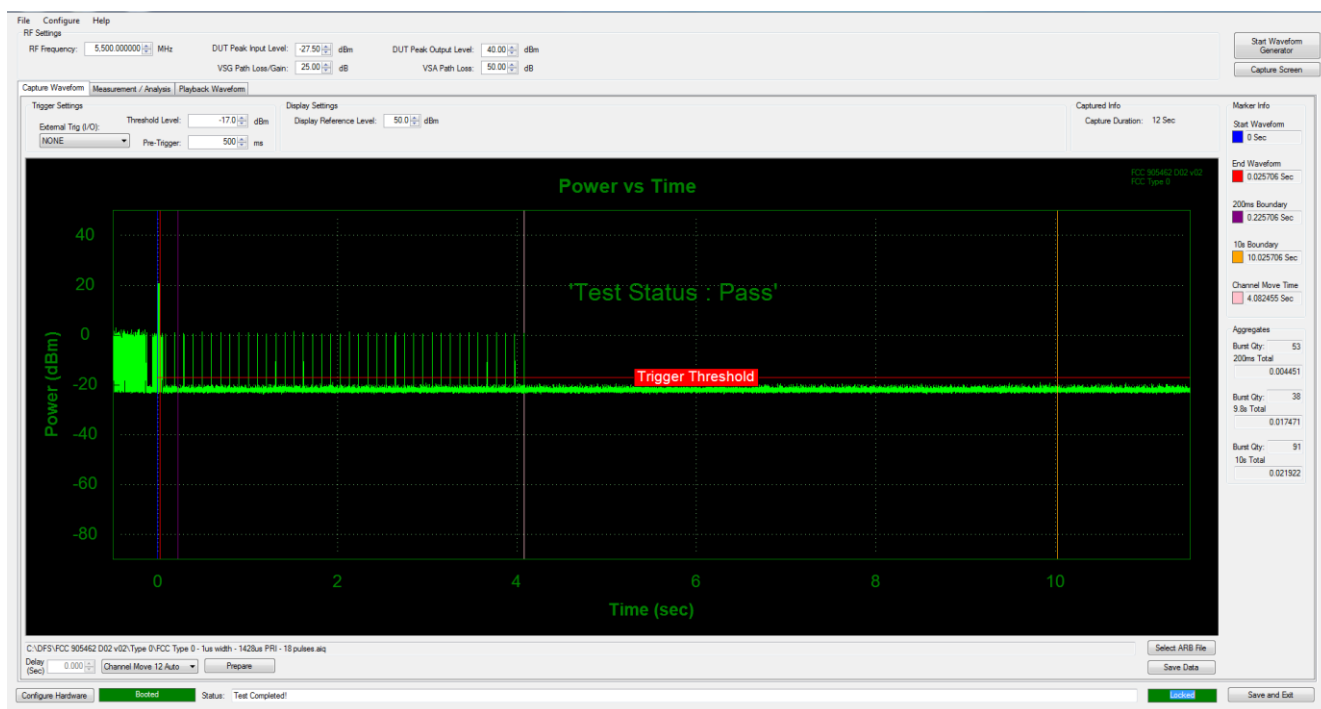
Figure 9-34. 5500MHz - Channel Move/ Closing Transmission Time - Mode 4 (20 MHz)
