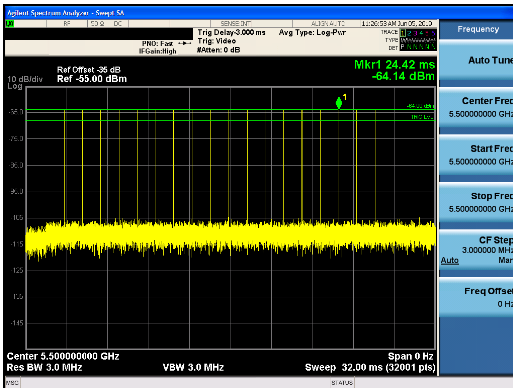
Figure 7-3. 5500MHz – Radar Pulse Type 0 (20MHz)
