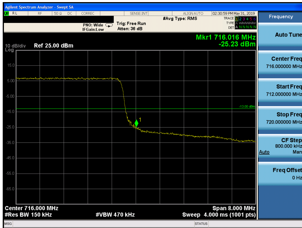
Plot 7-209. Upper Band Edge Plot (Band 17 - 10.0MHz QPSK - Full RB Configuration)
