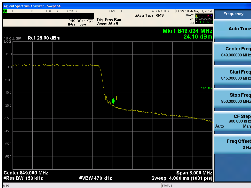
Plot 7-225. Upper Band Edge Plot (Band 26 - 10.0MHz QPSK - Full RB Configuration)
