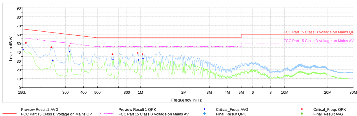
Plot 7-29. AC Line Conducted Plot with Bluetooth LE (L1, with Laptop)
