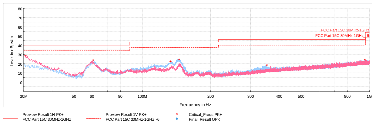
Plot 7-28. Radiated Spurious Plot below 1GHz (ePA – Ch.39, Pol. H & V, with AC/DC Adapter)
