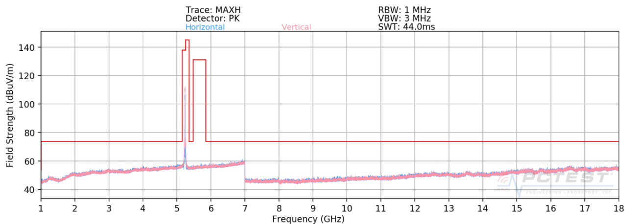
Plot 7-173. Radiated Spurious Plot above 1GHz SISO CORE0 (802.11n – U1 Ch. 48)
