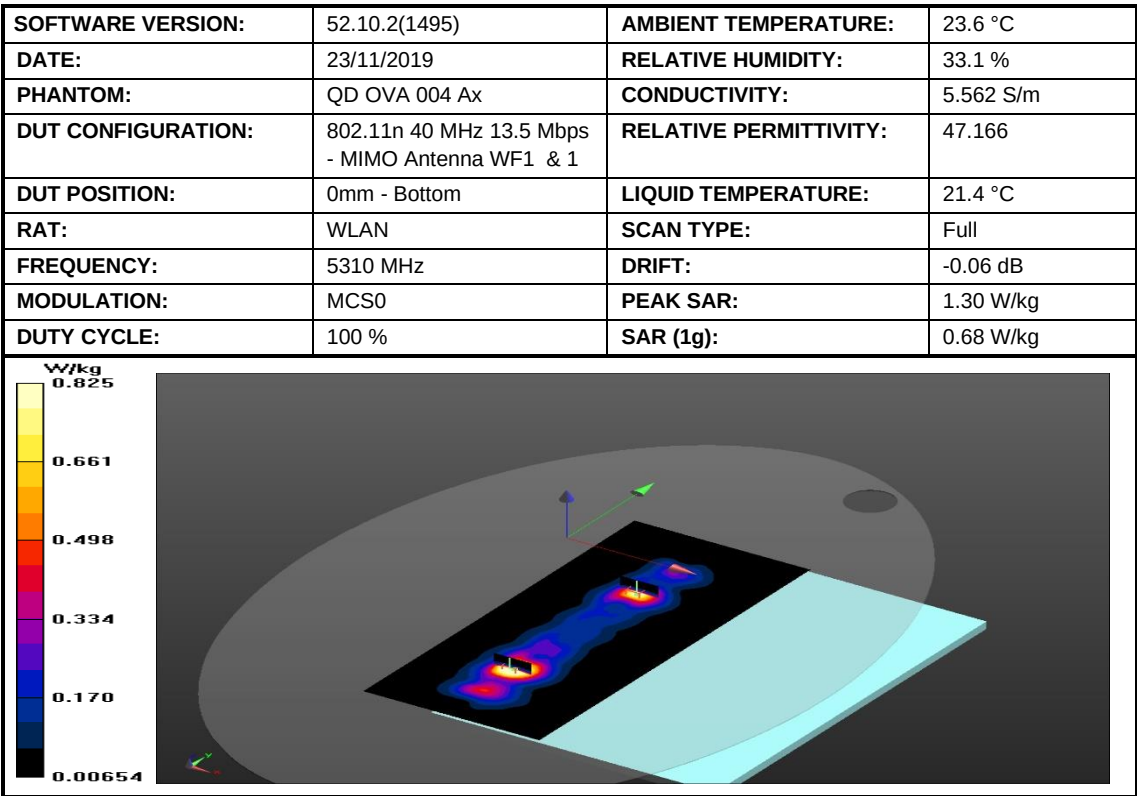
Figure 16: SAR Body Testing Results for the A2179 at 5310 MHz.
