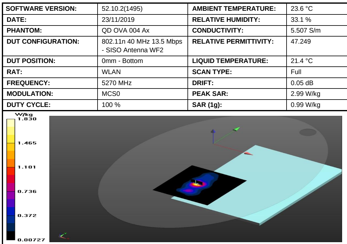
Figure 12: SAR Body Testing Results for the A2179 at 5270 MHz.
