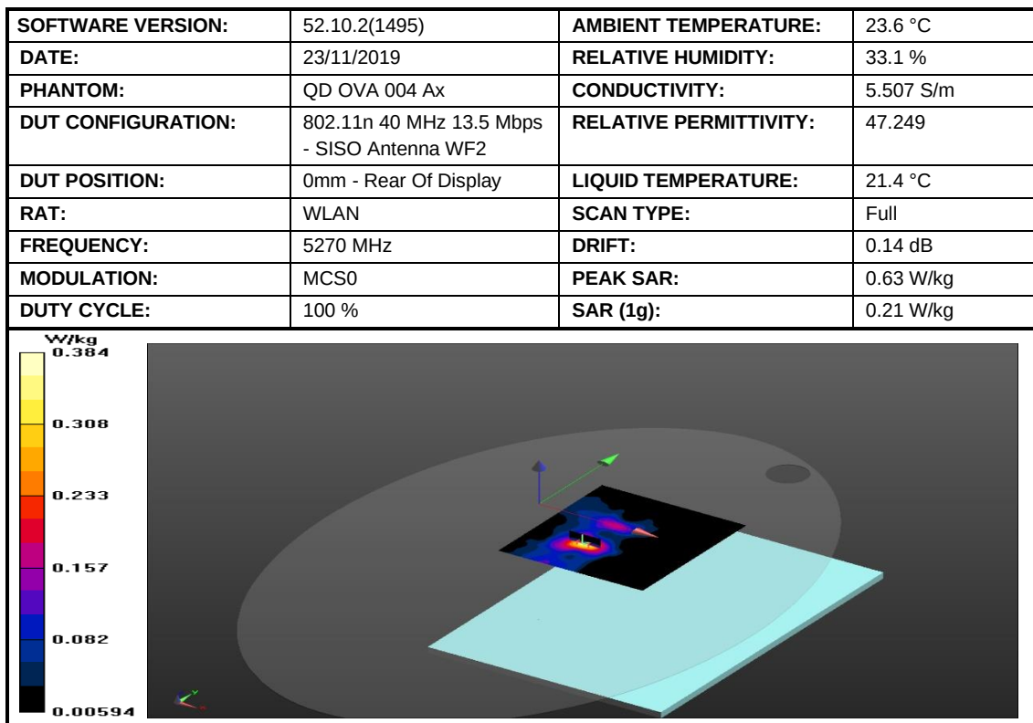
Figure 13: SAR Body Testing Results for the A2179 at 5270 MHz.
