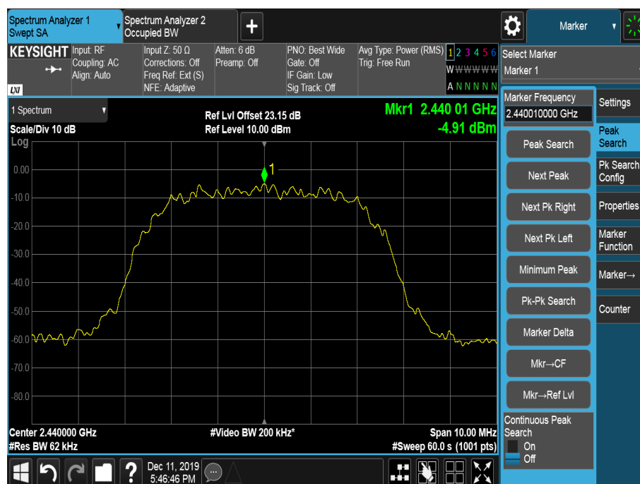
Figure 35 – 2440 MHz
