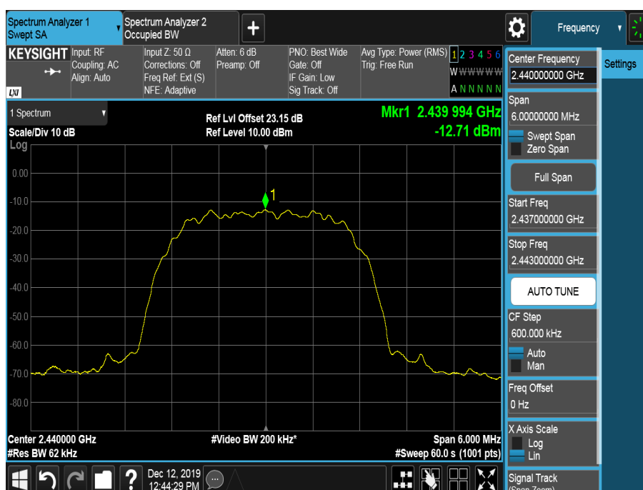
Figure 26 – 2440 MHz
