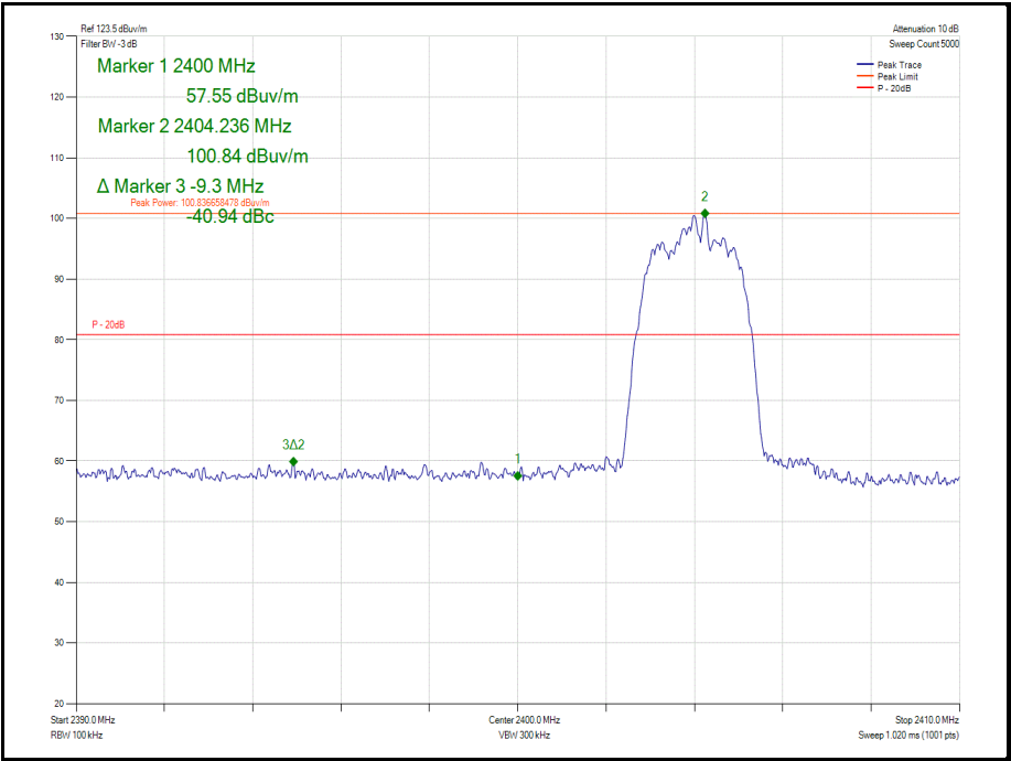
Figure 53 - GFSK/4DH5- 2404 MHz – Band Edge Frequency 2400.0 MHz (Plot should show P- 30dB limit in place of P- 20dB)
