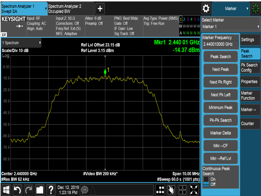
Figure 29 – 2440 MHz
