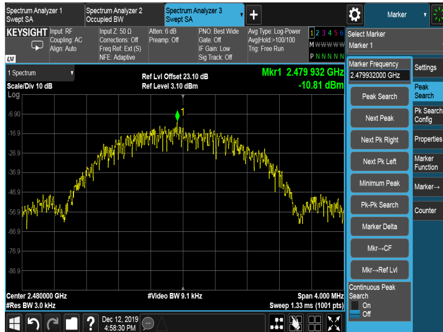
Figure 24 – 2480 MHz
