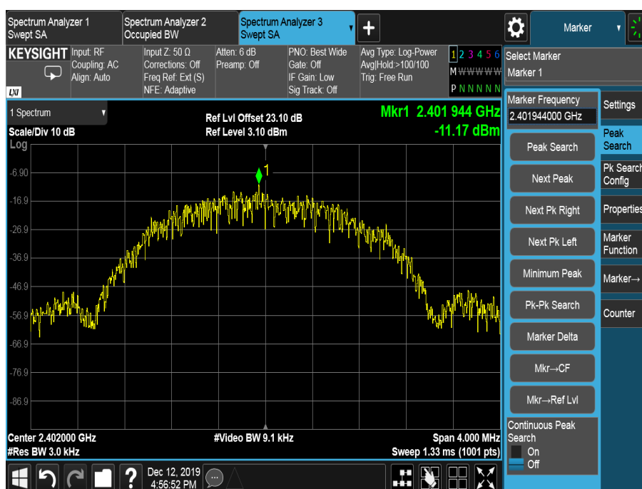
Figure 22 – 2402 MHz
