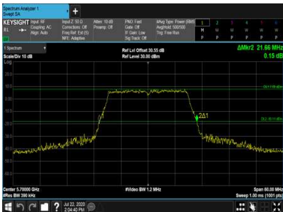
Figure 604 - 5700 MHz - 26 dB Emission Bandwidth
