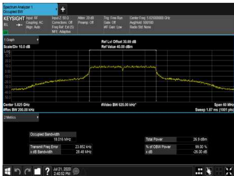
Figure 751 - 5825 MHz - 99% Occupied Bandwidth
