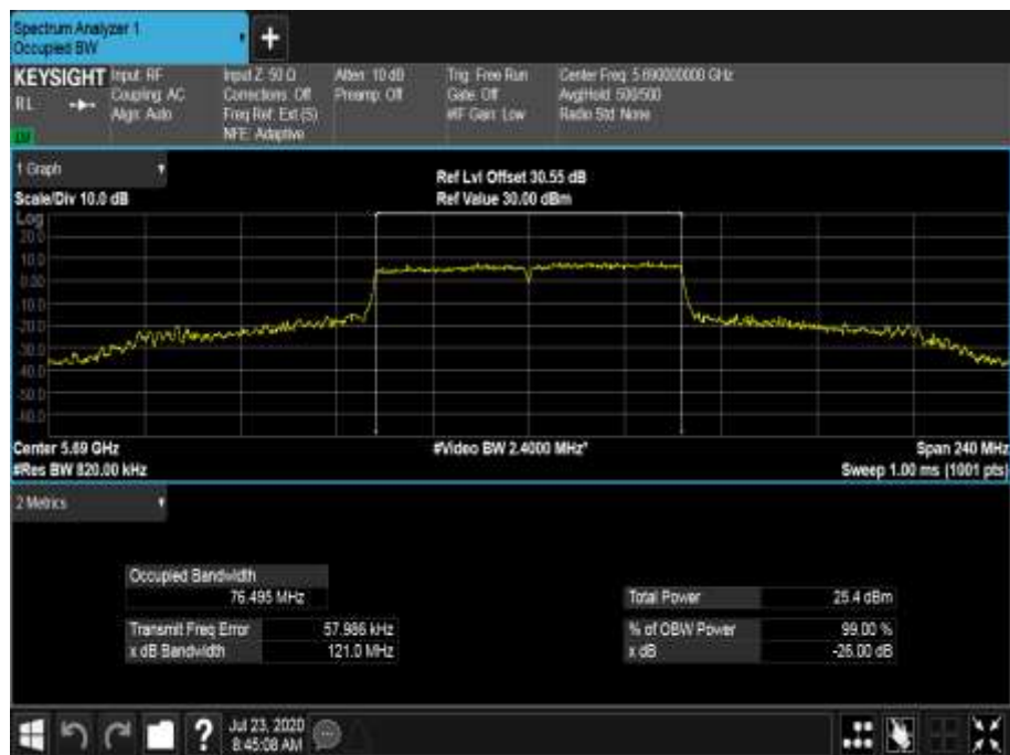
Figure 685 - 5690 MHz - 99% Occupied Bandwidth
