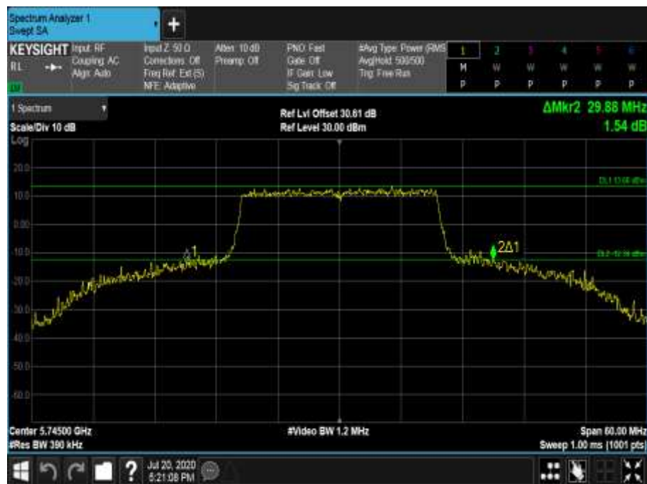
Figure 756 - 5745 MHz - 26 dB Emission Bandwidth
