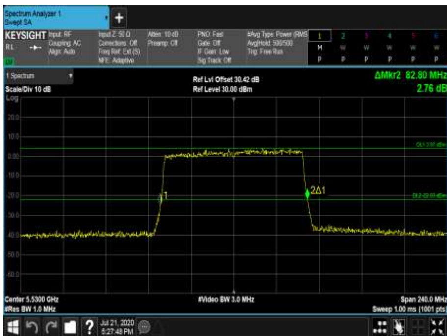
Figure 704 - 5530 MHz - 26 dB Emission Bandwidth
