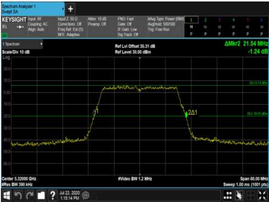
Figure 514 - 5320 MHz - 26 dB Emission Bandwidth
