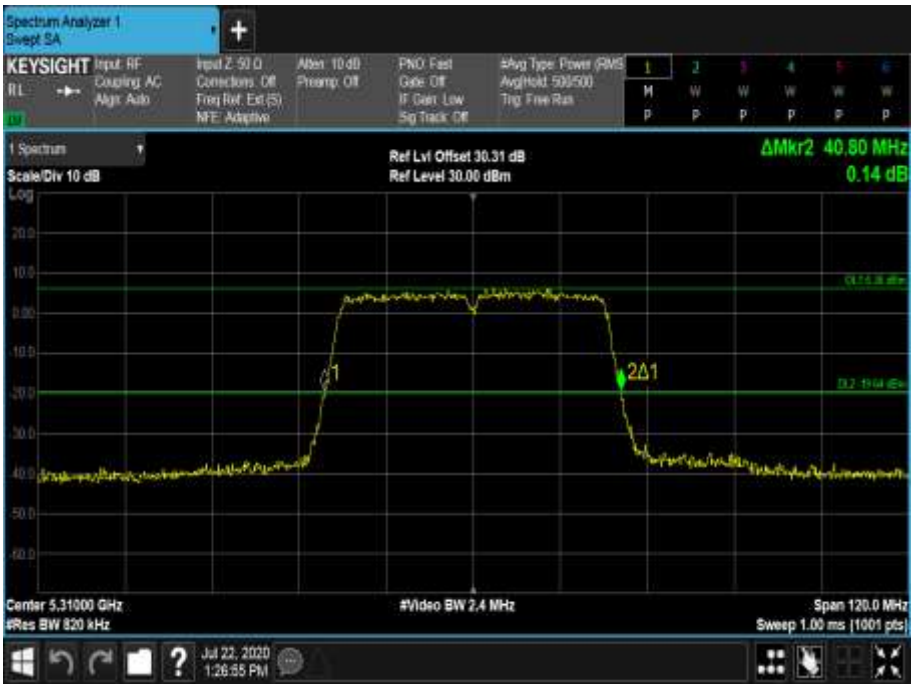
Figure 546 - 5310 MHz - 26 dB Emission Bandwidth
