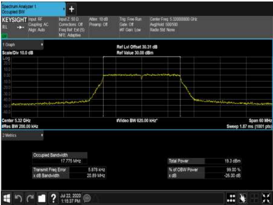
Figure 515 - 5320 MHz - 99% Occupied Bandwidth
