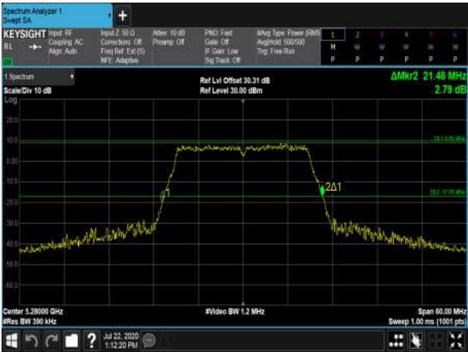
Figure 518 - 5280 MHz - 26 dB Emission Bandwidth
