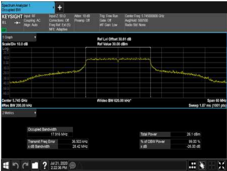
Figure 733 - 5745 MHz - 99% Occupied Bandwidth
