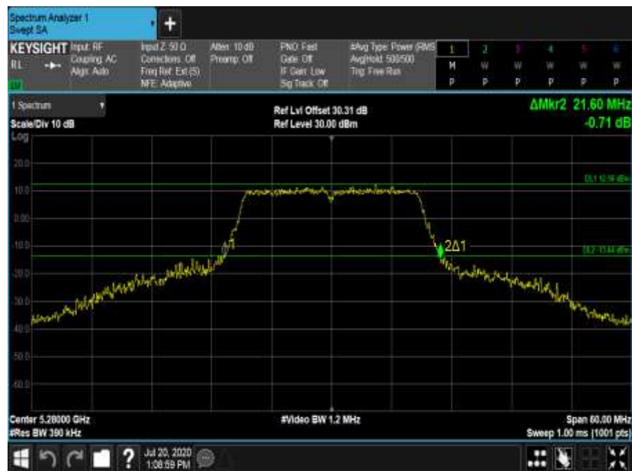
Figure 506 - 5280 MHz - 26 dB Emission Bandwidth
