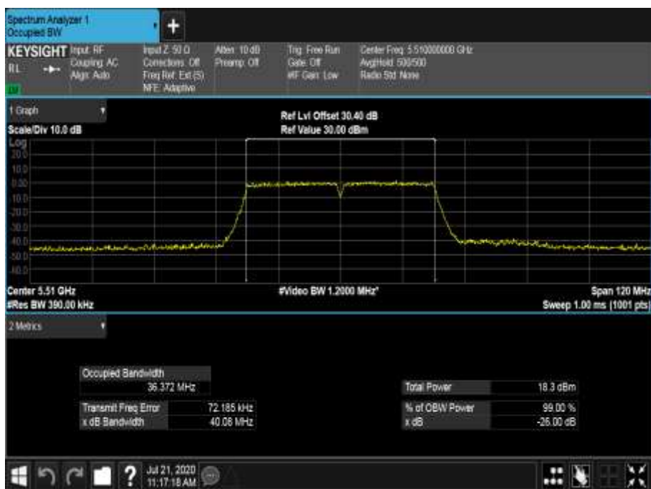
Figure 649 - 5510 MHz - 99% Occupied Bandwidth
