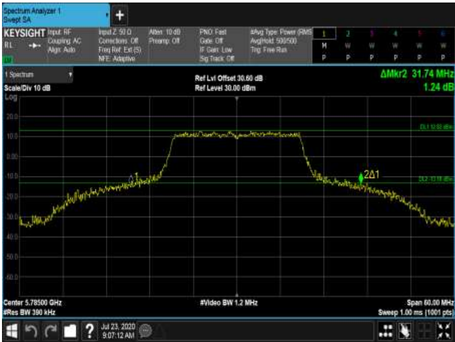
Figure 735 - 5785 MHz - 26 dB Emission Bandwidth
