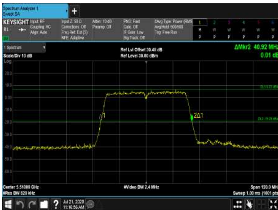
Figure 648 - 5510 MHz - 26 dB Emission Bandwidth
