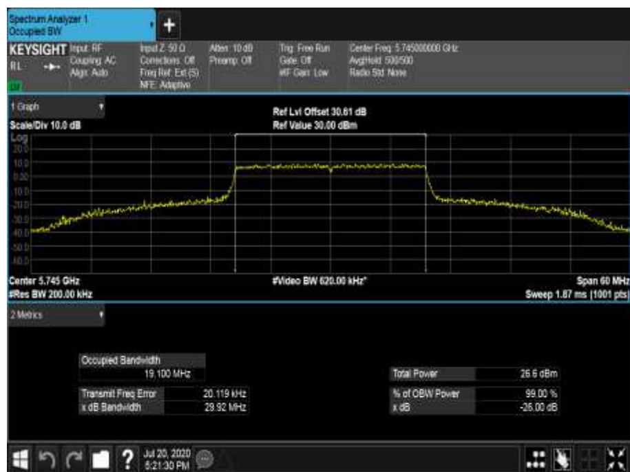
Figure 757 - 5745 MHz - 99% Occupied Bandwidth
