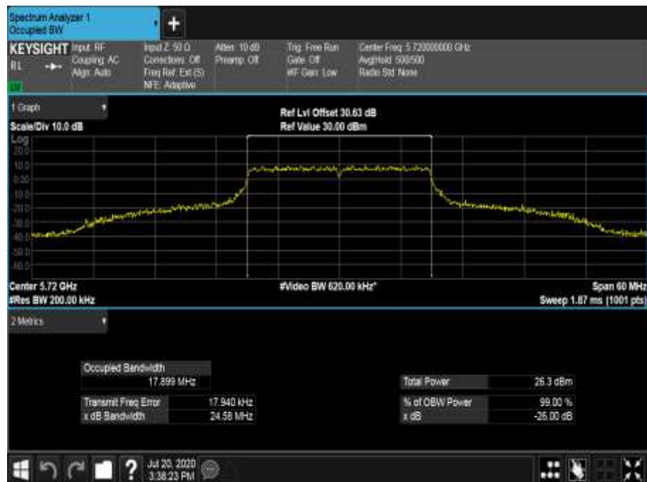
Figure 718 - 5720 MHz - 99% Occupied Bandwidth
