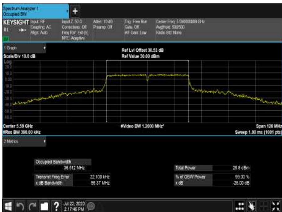
Figure 635 - 5590 MHz - 99% Occupied Bandwidth
