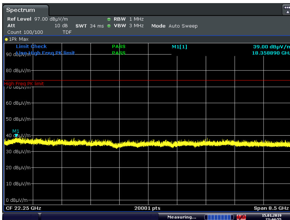
Plot 7-76. Radiated Spurious Plot above 18GHz (GFSK ePA – Ch. 78, Pol. V)
