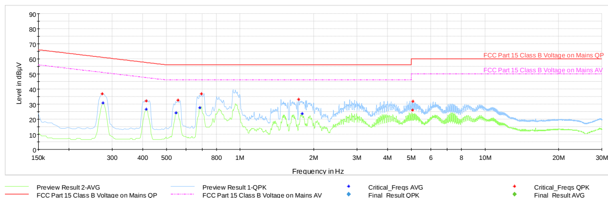
Plot 7-280. Line Conducted Plot with 802.11n UNII Band 1 Ch 36 (L1), with AC/DC Adapter
