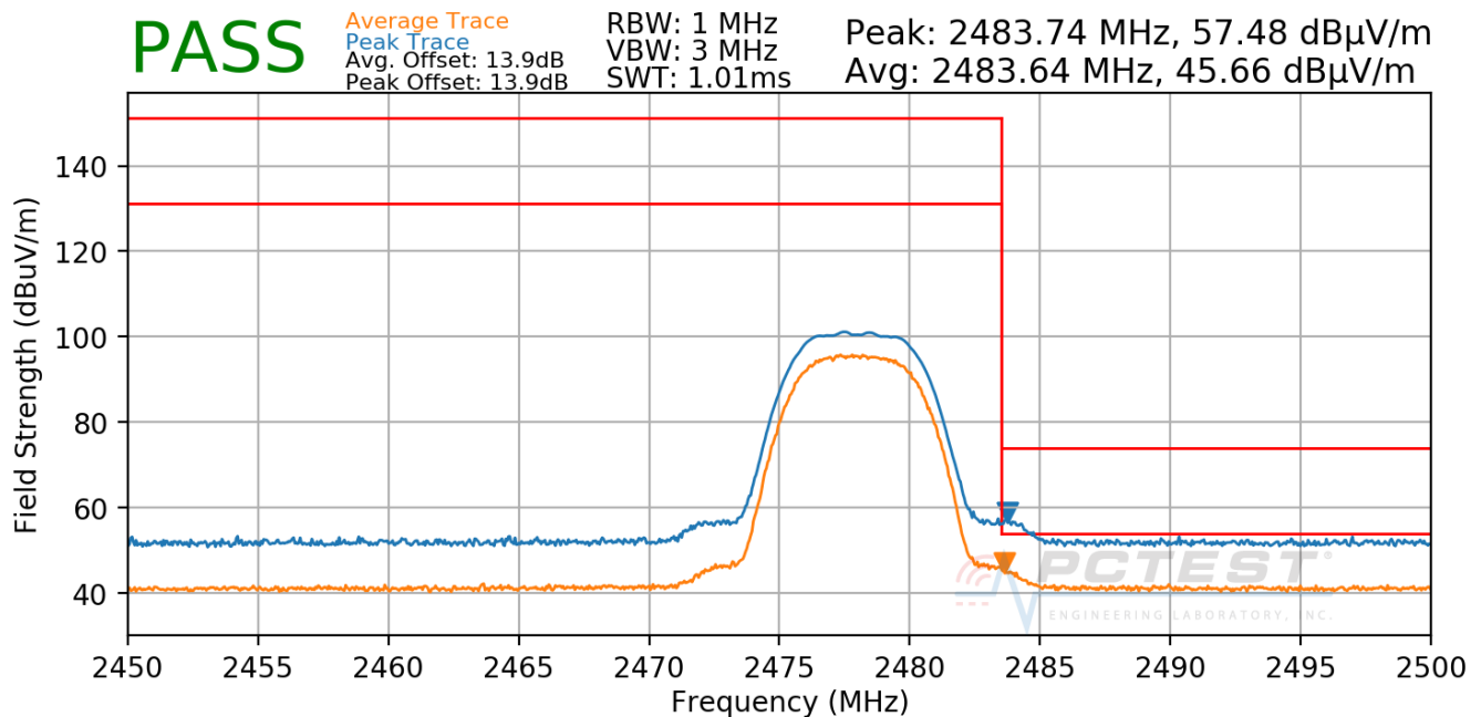
Plot 7-72. Radiated Restricted Upper Band Edge Measurement Ant-1 (Average & Peak)
