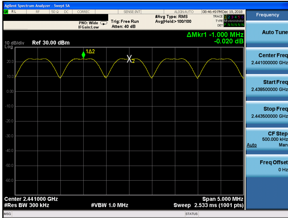
Plot 7-29. Channel Spacing Plot ANT 0 (Bluetooth, GFSK, ePA)
