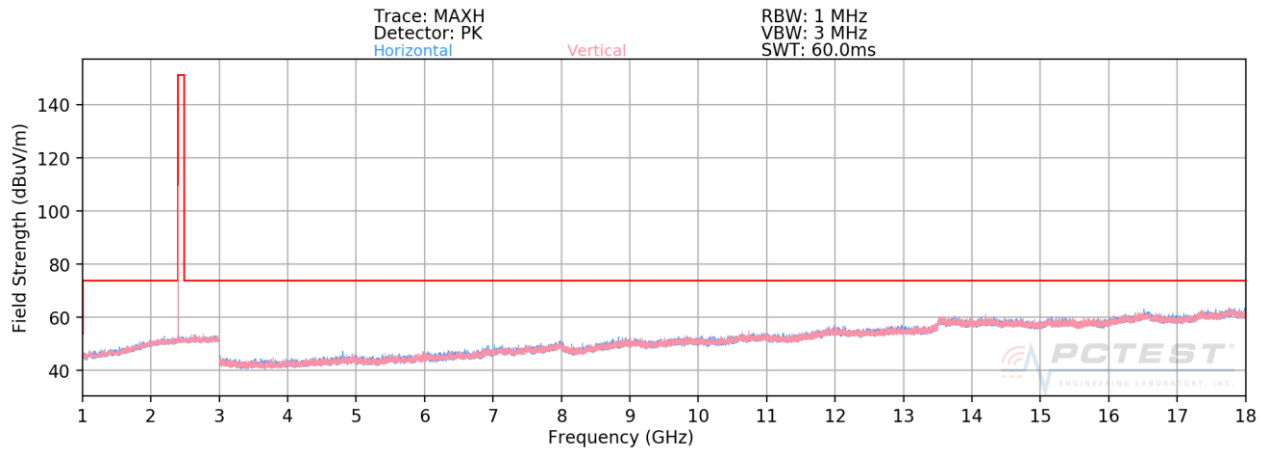
Plot 7-69. Radiated Spurious Plot above 1GHz ANT 0 (BT GFSK ePA – Ch. 0)
