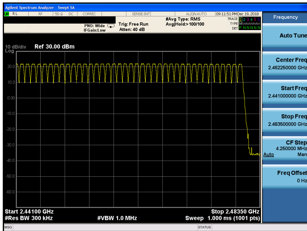
Plot 7-42. High End Spectrum Channel Hopping Plot ANT 1 (Bluetooth, GFSK, ePA)
