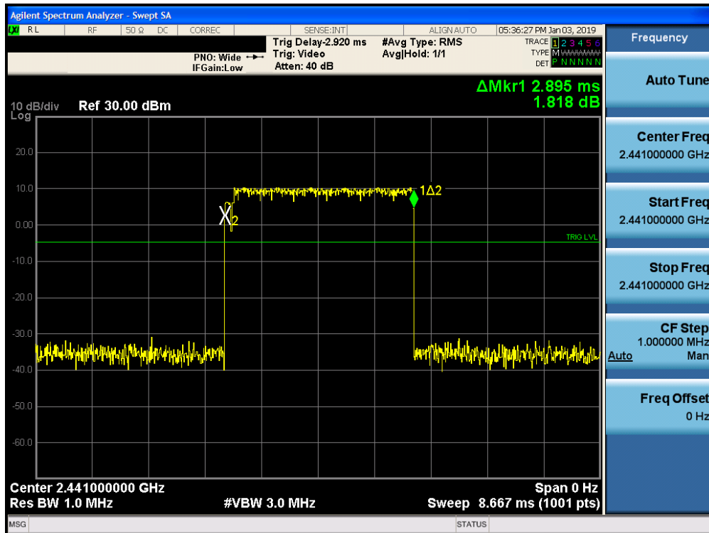
Plot 7-34. Time of Occupancy Plot ANT 0 (Bluetooth, 8DPSK, ePA)
