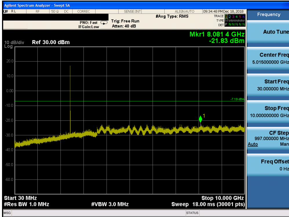
Plot 7-53. Conducted Spurious Plot ANT 0 (Bluetooth, 8DPSK, ePA – Ch. 39)
