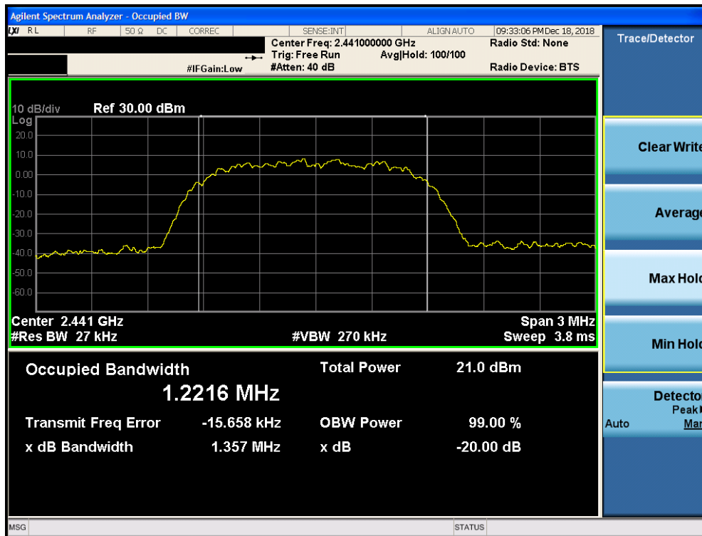
Plot 7-5. 20dB Bandwidth Plot ANT 0 (Bluetooth, 8DPSK, ePA – Ch. 39)
