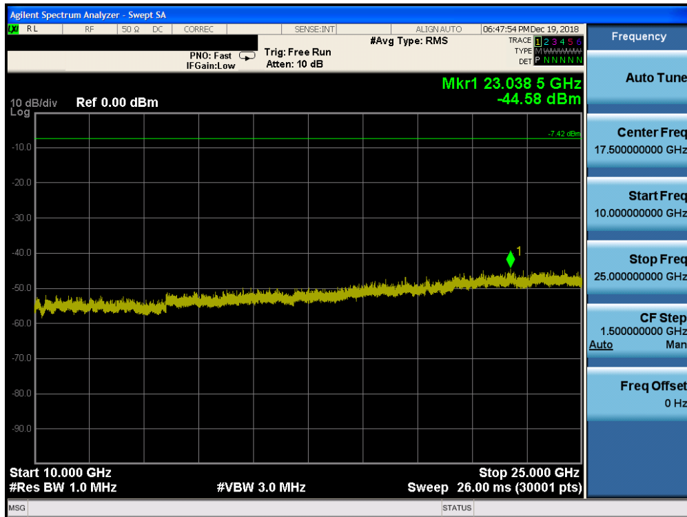
Plot 7-64. Conducted Spurious Plot ANT 1 (Bluetooth, 8DPSK, ePA – Ch. 0)
