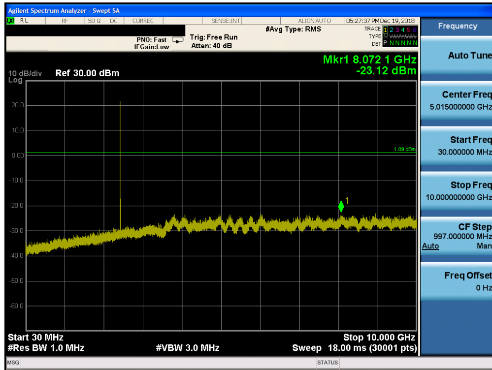
Plot 7-59. Conducted Spurious Plot ANT 1 (Bluetooth, GFSK, ePA – Ch. 39)
