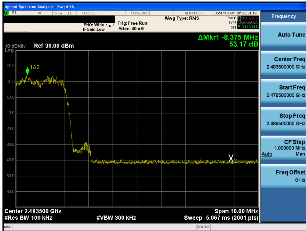
Plot 7-20. Band Edge Plot ANT 0 (Bluetooth with Hopping Enabled, 8DPSK, ePA)
