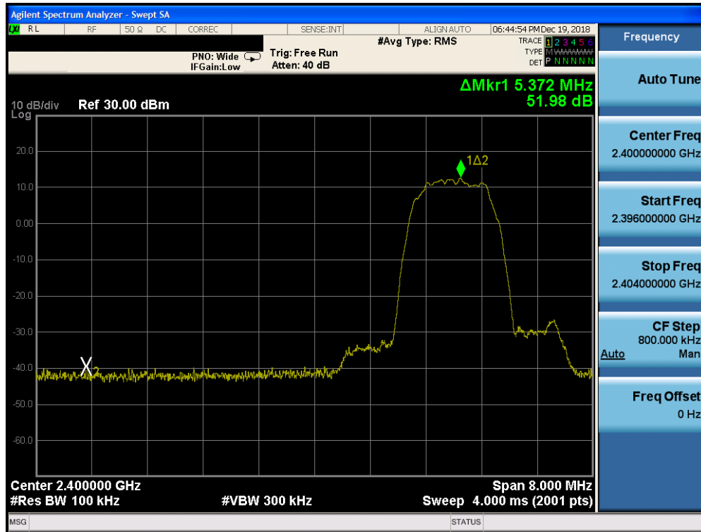
Plot 7-25. Band Edge Plot ANT 1 (Bluetooth with Hopping Disabled, 8DPSK, ePA – Ch. 0)
