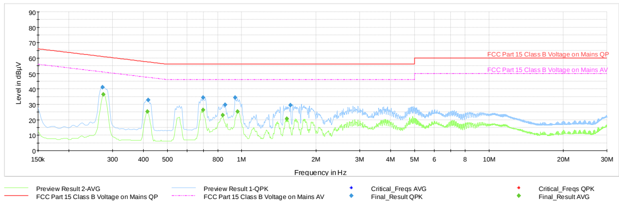
Plot 7-91. AC Line-Conducted Test Plot – GFSK ePA Ch.0 (N, with AC/DC Adapter)
