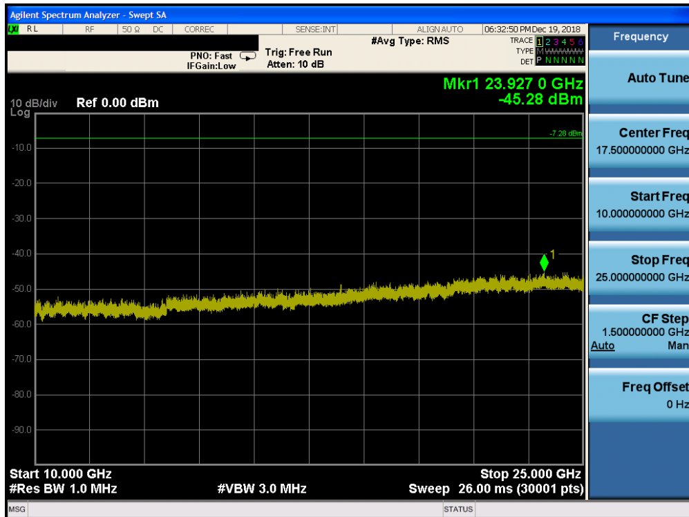
Plot 7-66. Conducted Spurious Plot ANT 1 (Bluetooth, 8DPSK, ePA Ch. 39)
