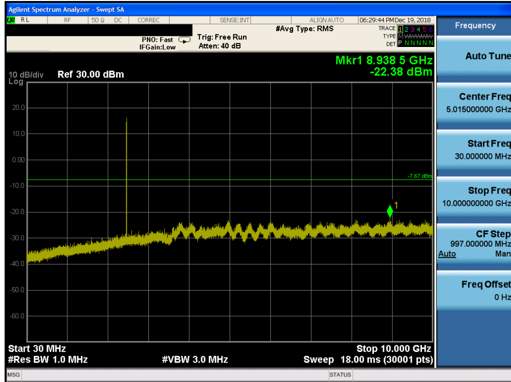
Plot 7-67. Conducted Spurious Plot ANT 1 (Bluetooth, 8DPSK, ePA – Ch. 78)
