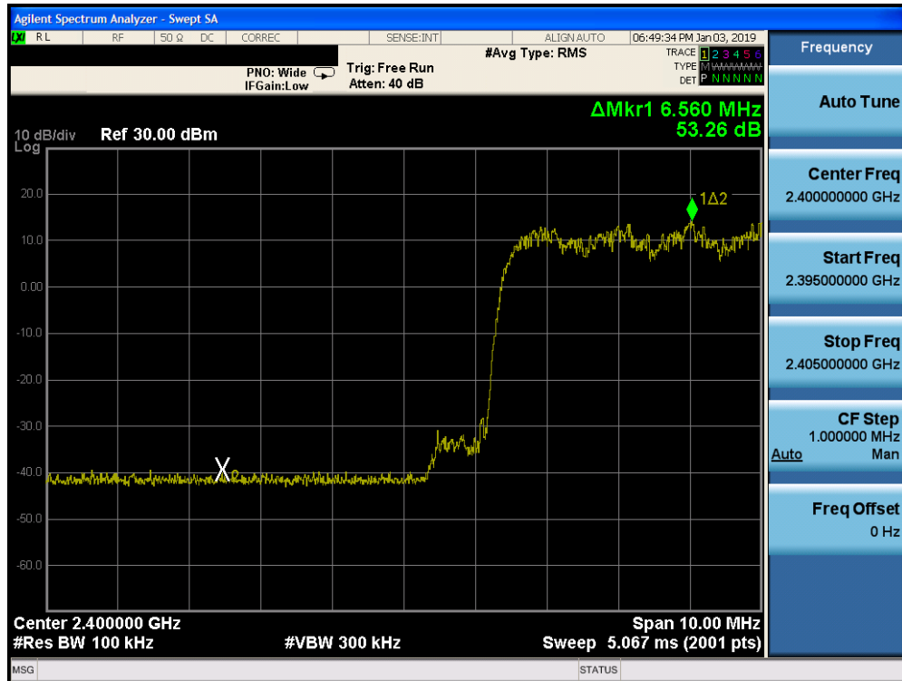
Plot 7-19. Band Edge Plot ANT 0 (Bluetooth with Hopping Enabled, 8DPSK, ePA)
