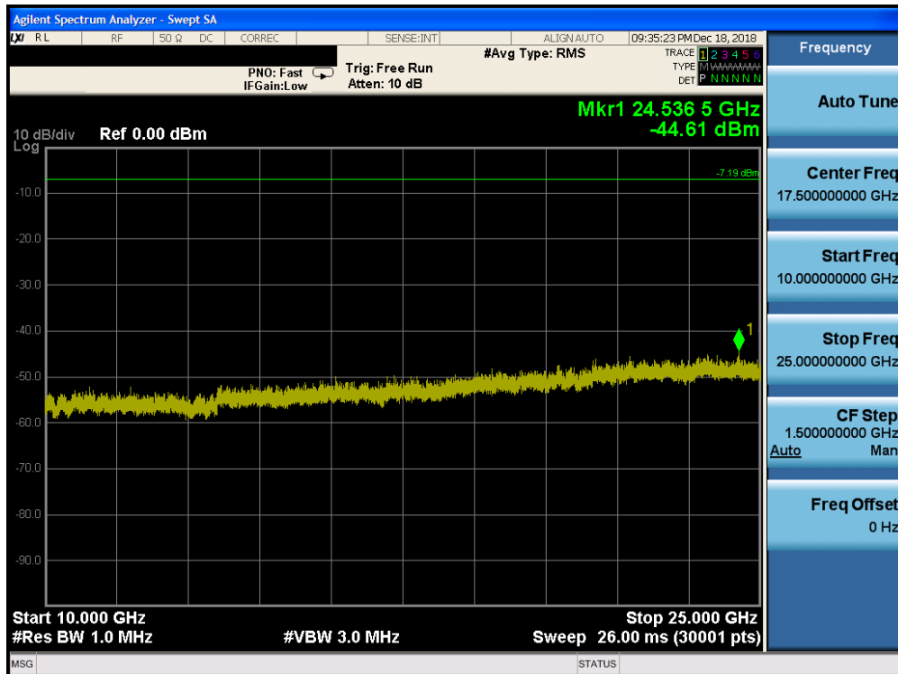
Plot 7-54. Conducted Spurious Plot ANT 0 (Bluetooth, 8DPSK, ePA Ch. 39)
