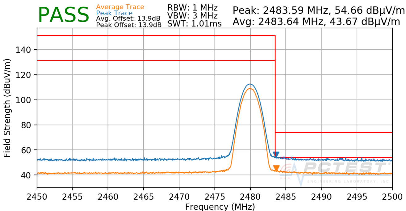
Plot 7-83. Radiated Restricted Upper Band Edge Measurement ANT 0
