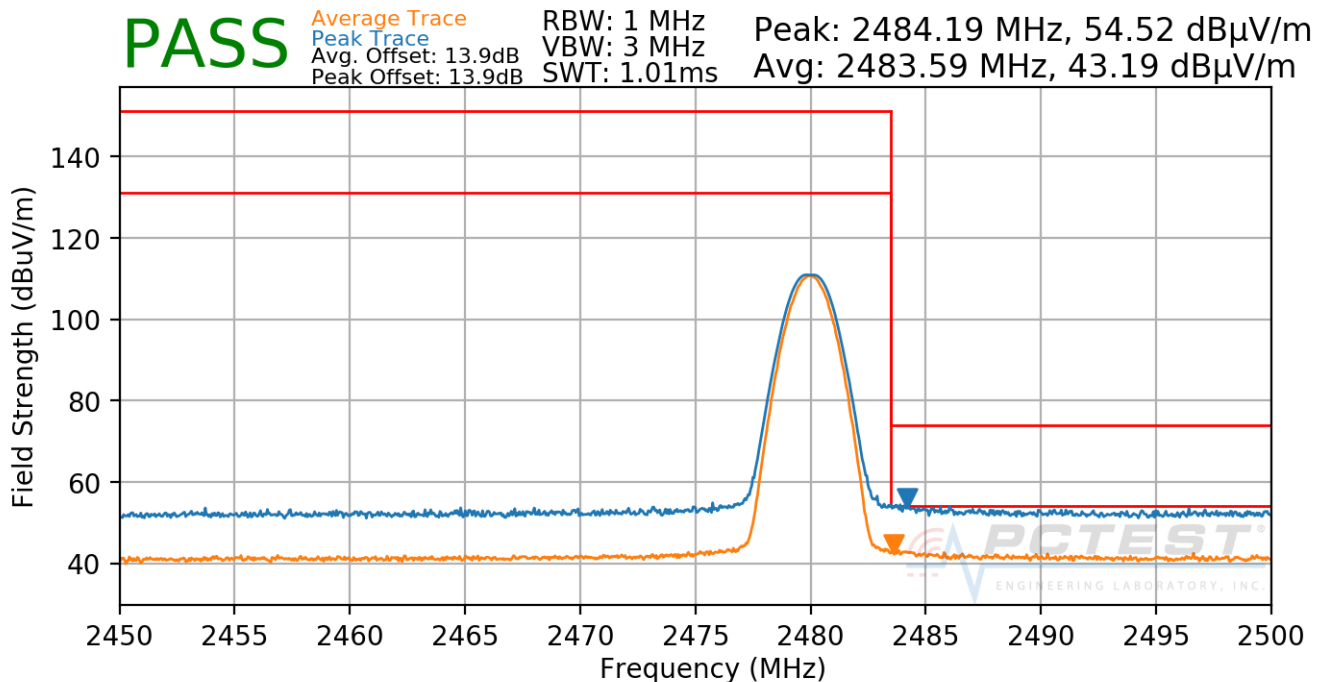
Plot 7-82. Radiated Restricted Upper Band Edge Measurement ANT 0
