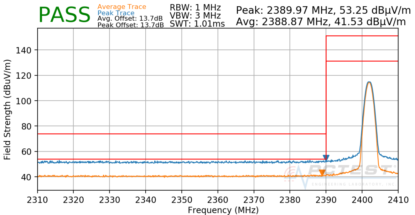
Plot 7-84. Radiated Restricted Lower Band Edge Measurement ANT 1
