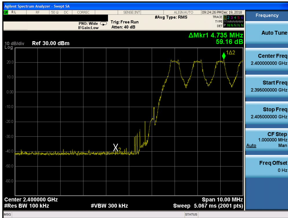
Plot 7-23. Band Edge Plot ANT 1 (Bluetooth with Hopping Enabled, GFSK, ePA)
