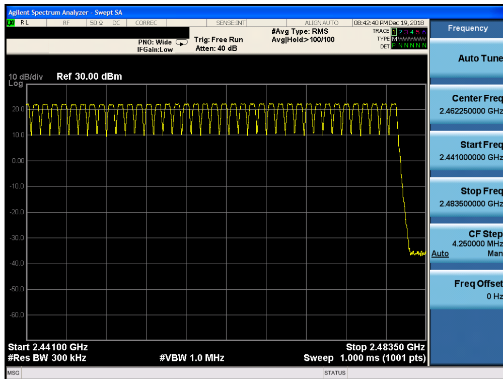
Plot 7-38. High End Spectrum Channel Hopping Plot ANT 0 (Bluetooth, GFSK, ePA)
