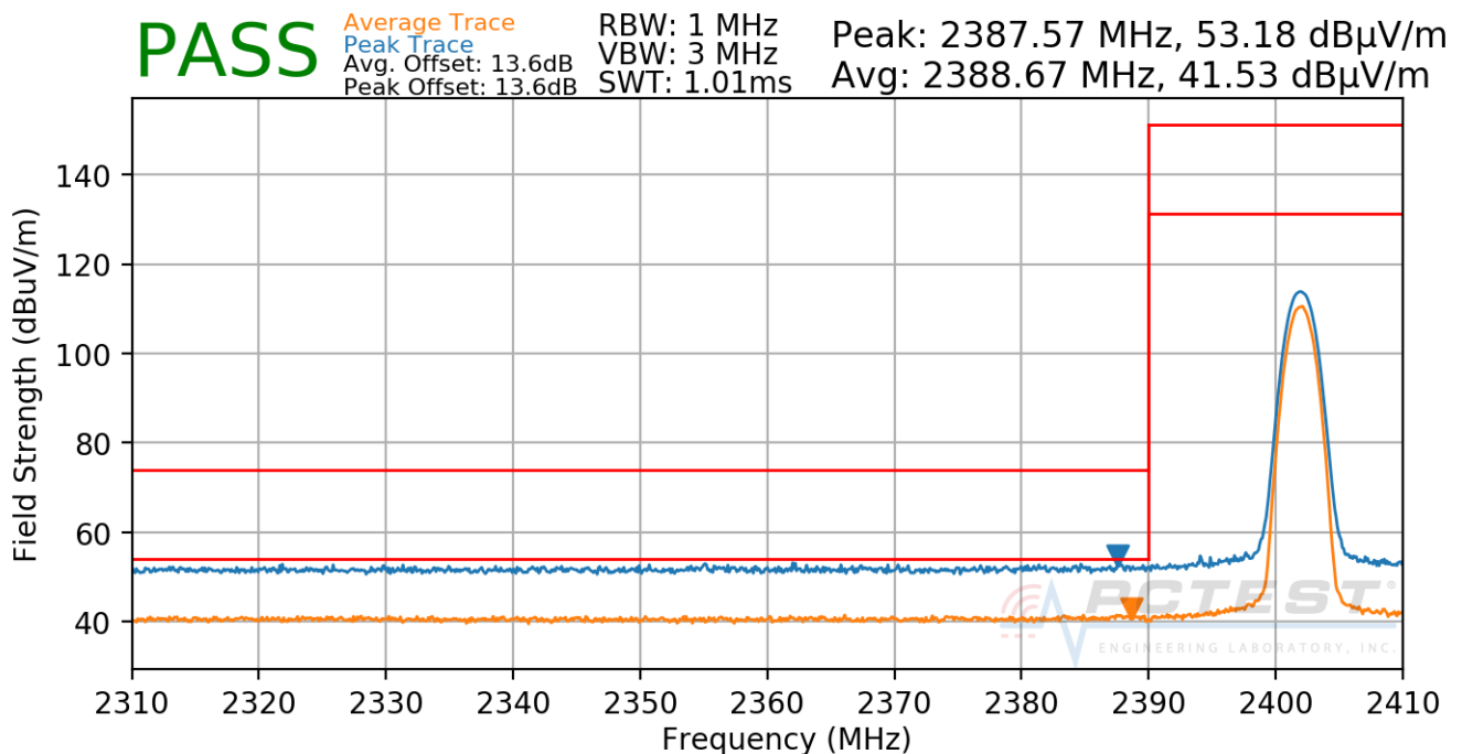
Plot 7-81. Radiated Restricted Lower Band Edge Measurement ANT 0
