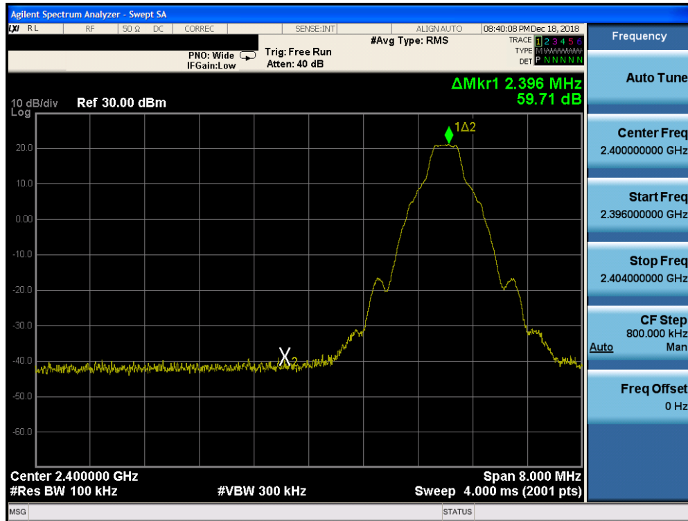
Plot 7-13. Band Edge Plot ANT 0 (Bluetooth with Hopping Disabled, GFSK, ePA – Ch. 0)
