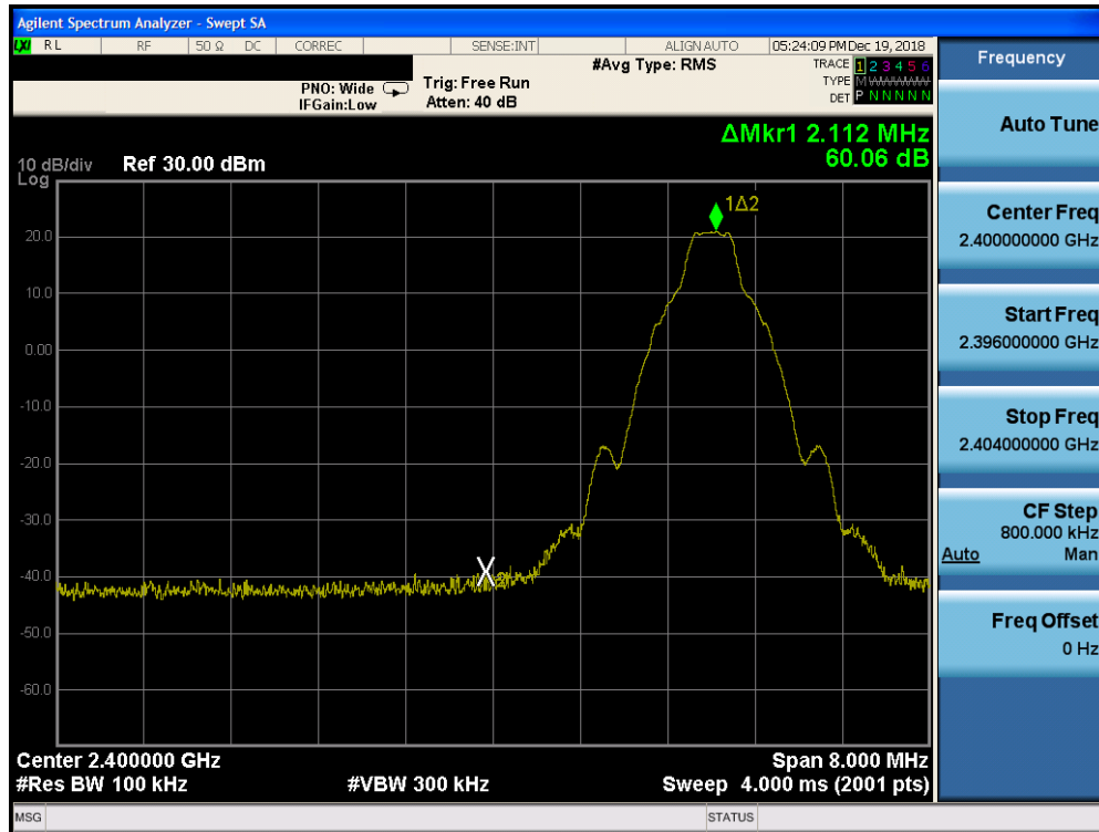
Plot 7-21. Band Edge Plot ANT 1 (Bluetooth with Hopping Disabled, GFSK, ePA – Ch. 0)
