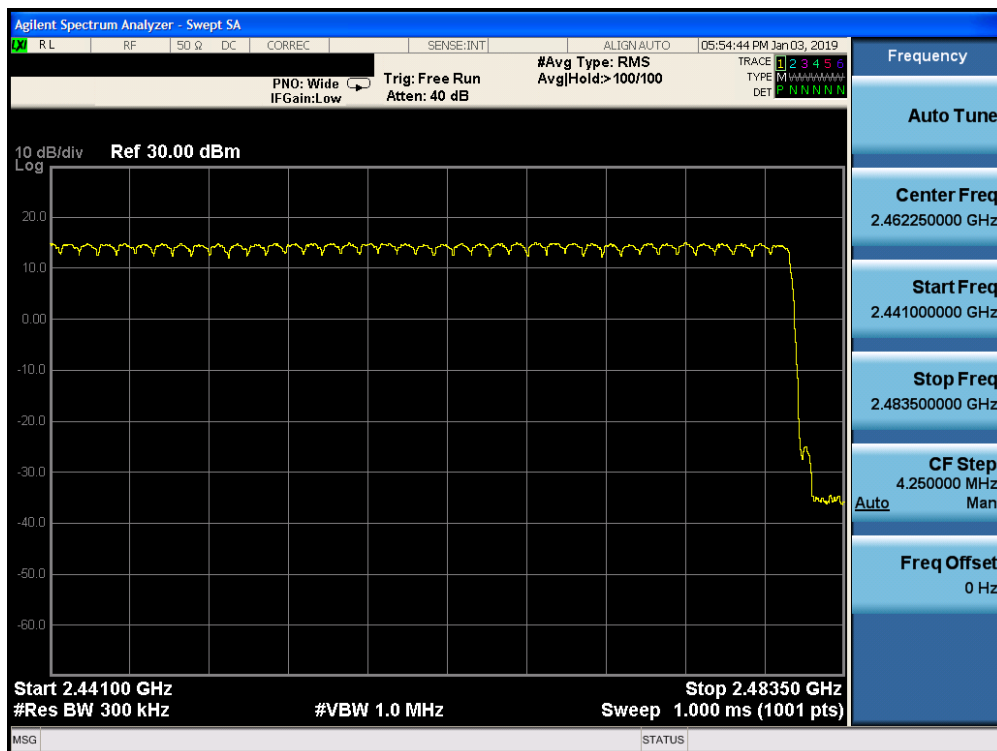
Plot 7-44. High End Spectrum Channel Hopping Plot ANT 1 (Bluetooth, 8DPSK, ePA)
