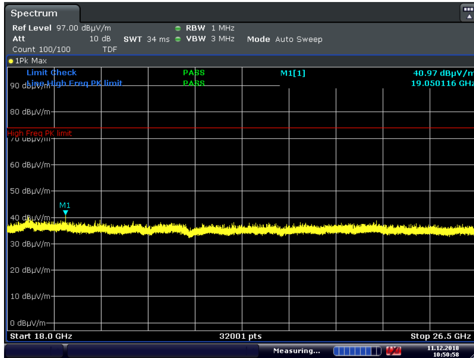
Plot 7-75. Radiated Spurious Plot above 18GHz ANT1 (GFSK ePA – Ch. 78, Pol. H)
