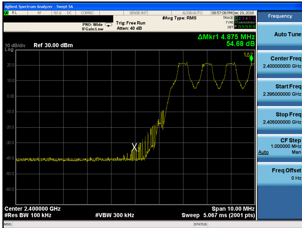
Plot 7-15. Band Edge Plot ANT 0 (Bluetooth with Hopping Enabled, GFSK, ePA)
