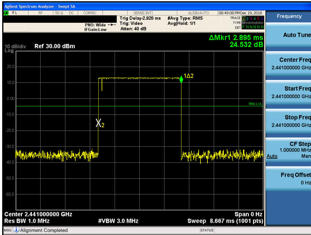
Plot 7-33. Time of Occupancy Plot ANT 0 (Bluetooth, GFSK, ePA)
