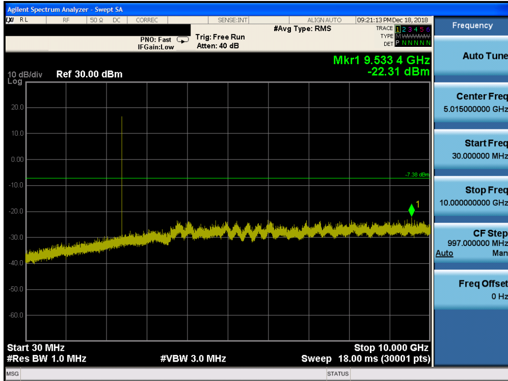
Plot 7-51. Conducted Spurious Plot ANT 0 (Bluetooth, 8DPSK, ePA – Ch. 0)
