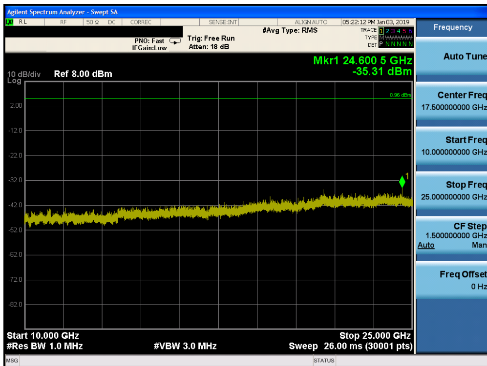
Plot 7-46. Conducted Spurious Plot ANT 0 (Bluetooth, GFSK, ePA – Ch. 0)
