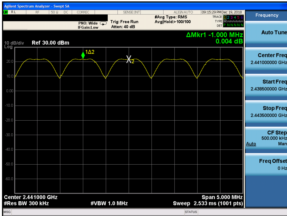
Plot 7-31. Channel Spacing Plot ANT 1 (Bluetooth, GFSK, ePA)
