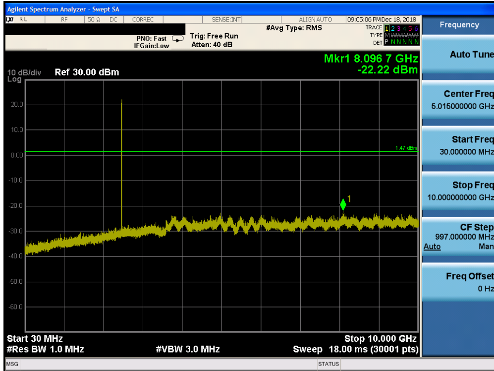
Plot 7-49. Conducted Spurious Plot ANT 0 (Bluetooth, GFSK, ePA – Ch. 78)
