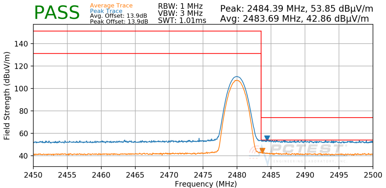
Plot 7-87. Radiated Restricted Upper Band Edge Measurement ANT 1
