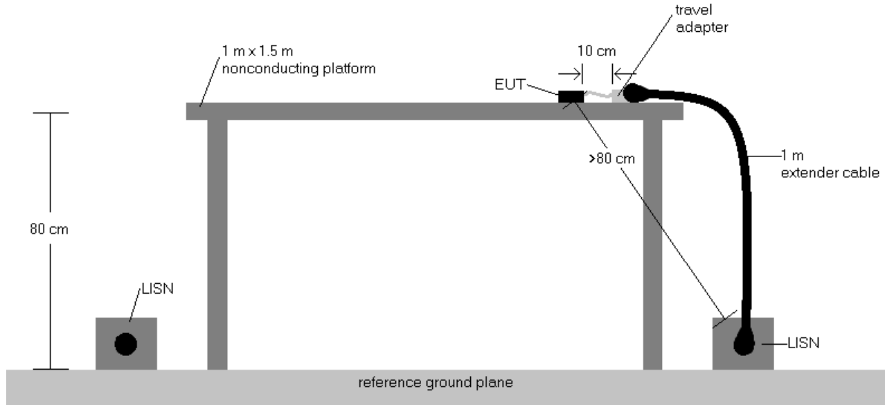
Figure 7-11. Test Instrument & Measurement Setup
