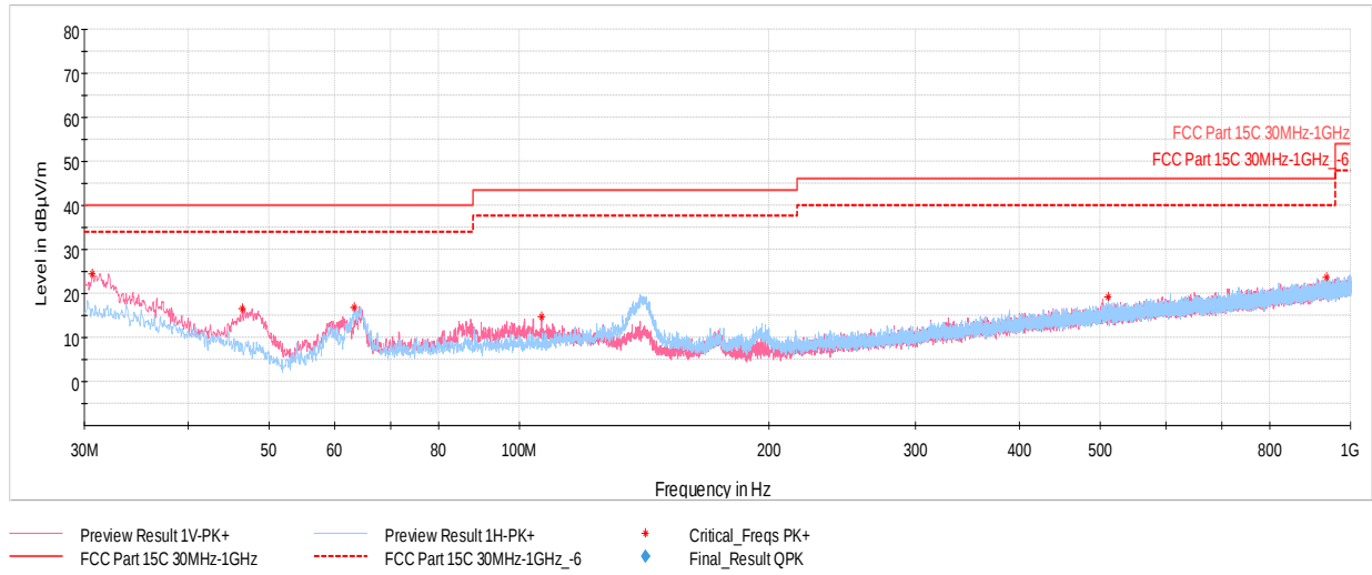
Plot 7-88. Radiated Spurious Plot below 1GHz GFSK ePA ANT 1, with AC/DC Adapter
