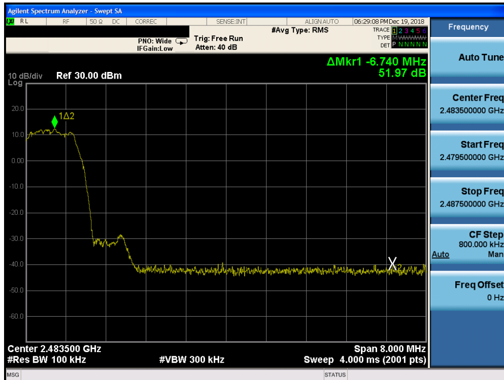
Plot 7-26. Band Edge Plot ANT 1 (Bluetooth with Hopping Disabled, 8DPSK, ePA – Ch. 78)
