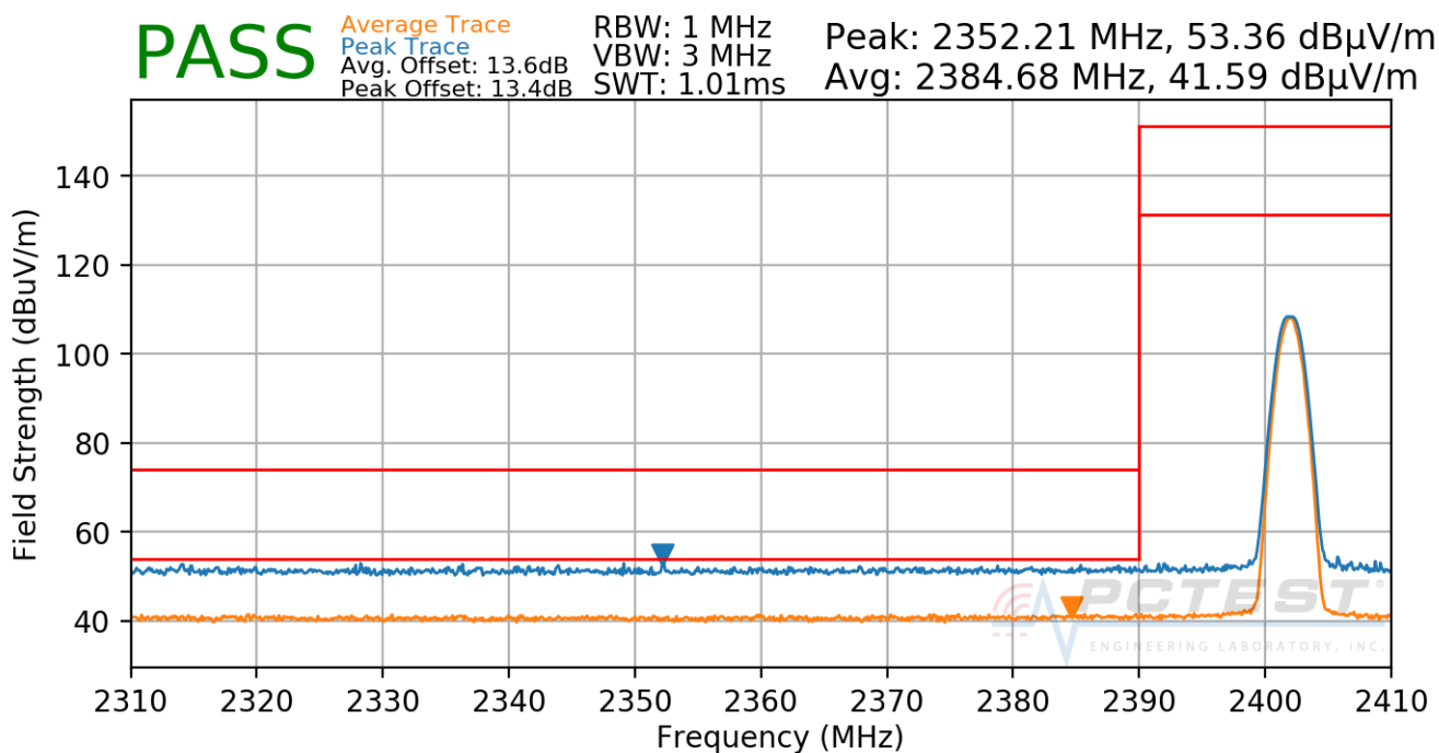
Plot 7-80. Radiated Restricted Lower Band Edge Measurement ANT 0
