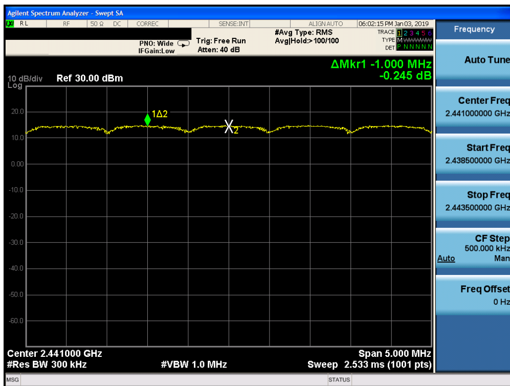
Plot 7-32. Channel Spacing Plot ANT 1 (Bluetooth, 8DPSK, ePA)
