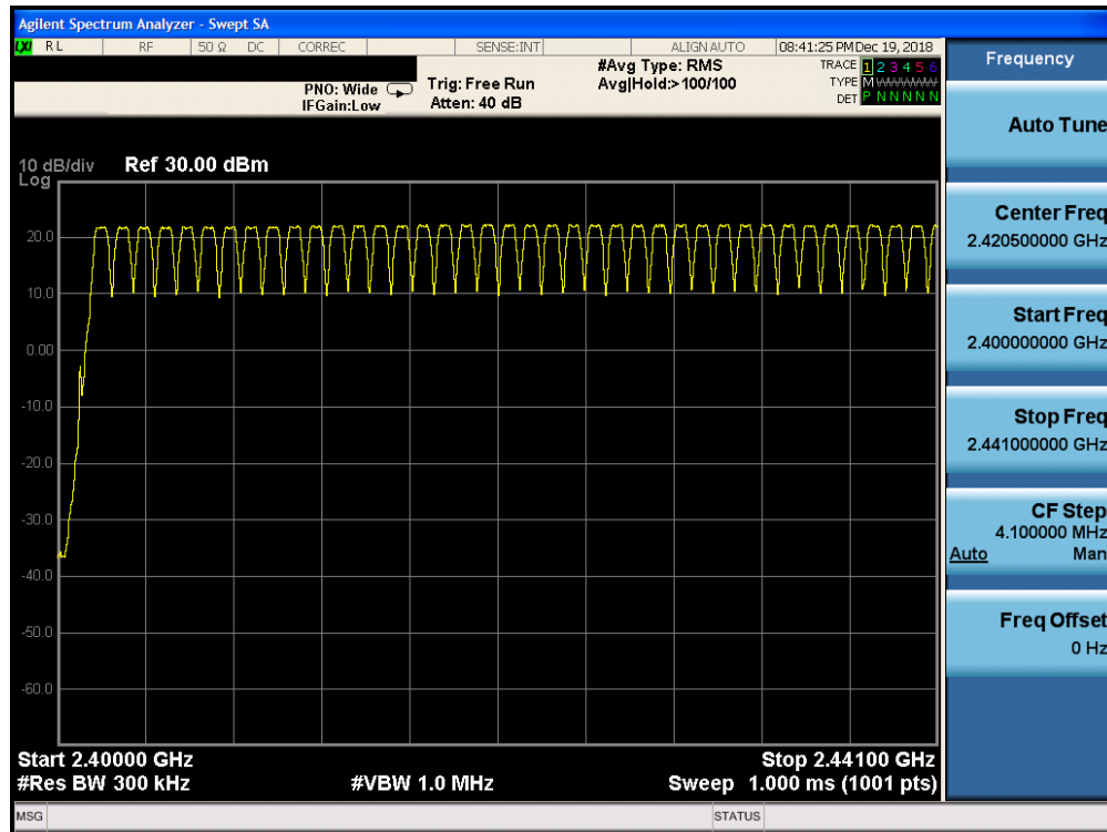
Plot 7-37. Low End Spectrum Channel Hopping Plot ANT 0 (Bluetooth, GFSK, ePA)
