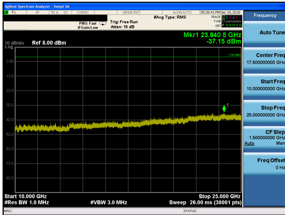
Plot 7-60. Conducted Spurious Plot ANT 1 (Bluetooth, GFSK, ePA Ch. 39)
