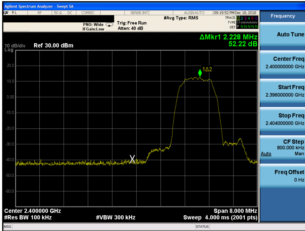
Plot 7-17. Band Edge Plot ANT 0 (Bluetooth with Hopping Disabled, 8DPSK, ePA – Ch. 0)
