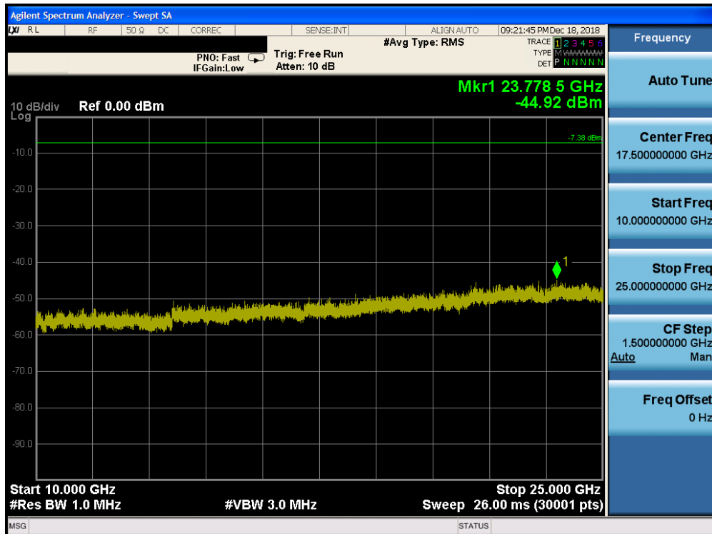
Plot 7-52. Conducted Spurious Plot ANT 0 (Bluetooth, 8DPSK, ePA – Ch. 0)
