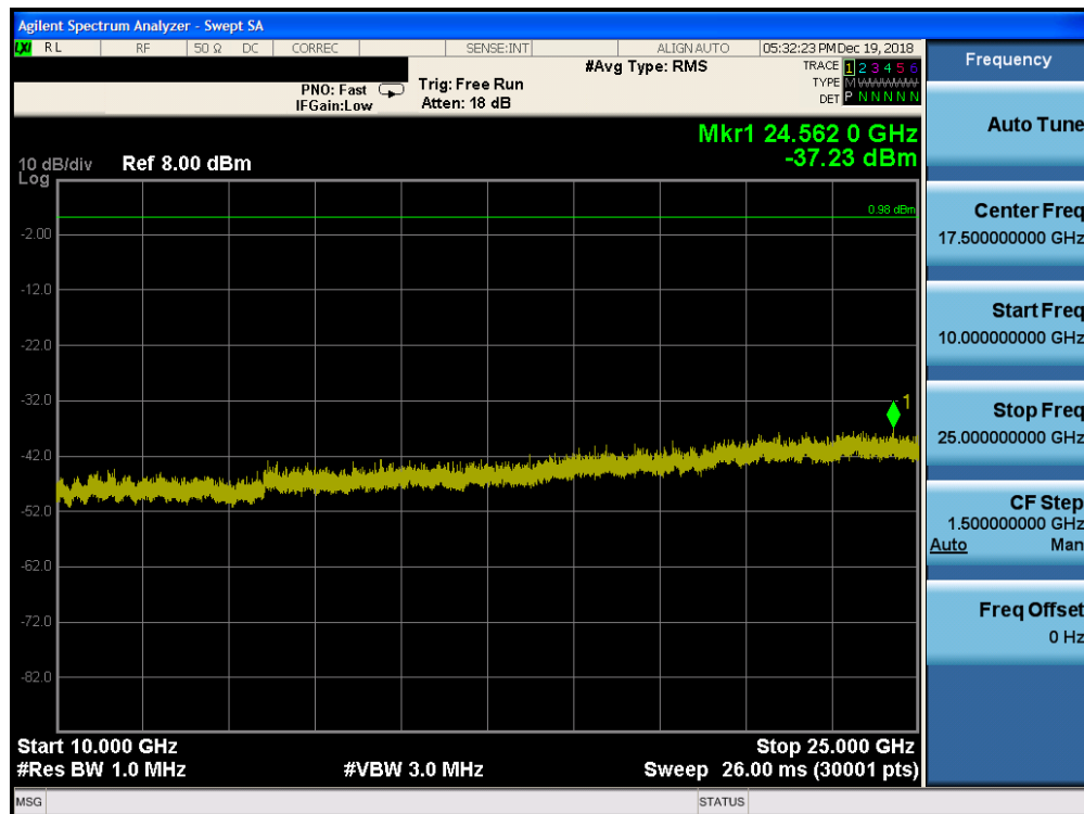
Plot 7-62. Conducted Spurious Plot ANT 1 (Bluetooth, GFSK, ePA – Ch. 78)
