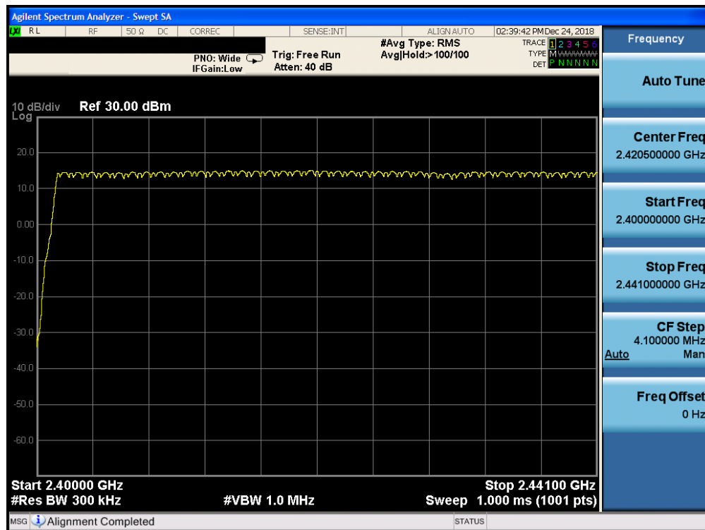
Plot 7-39. Low End Spectrum Channel Hopping Plot ANT 0 (Bluetooth, 8DPSK, ePA)
