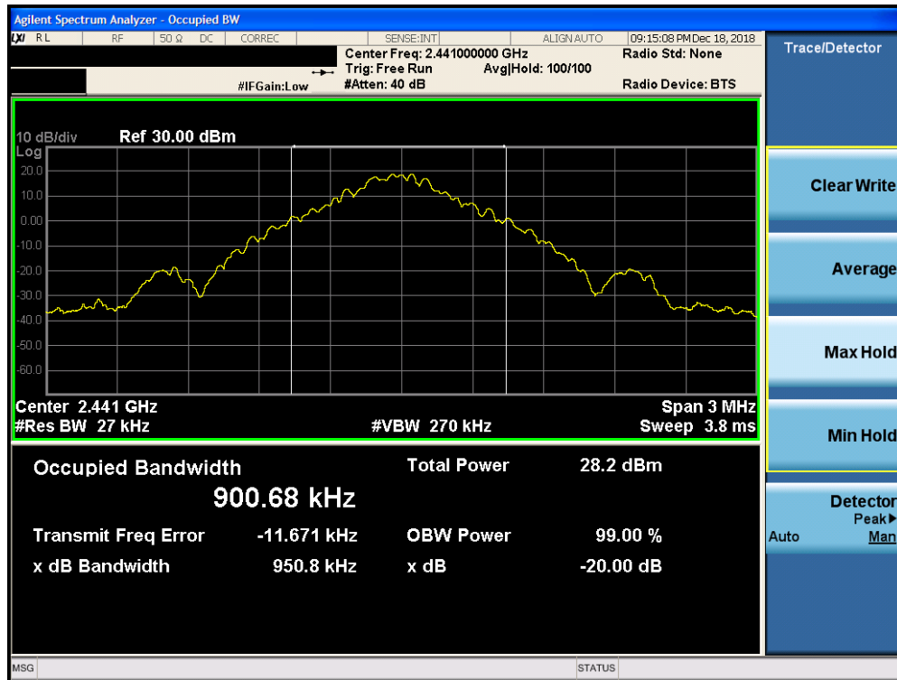
Plot 7-2. 20dB Bandwidth Plot ANT 0 (Bluetooth, GFSK, ePA – Ch. 39)
