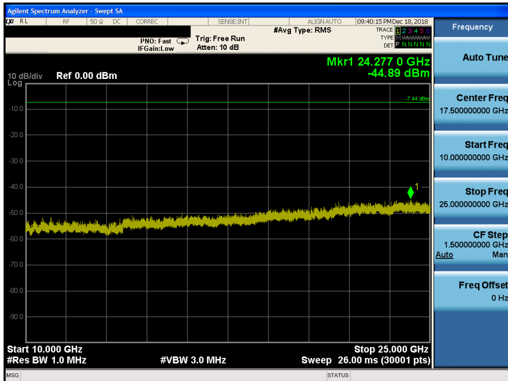
Plot 7-56. Conducted Spurious Plot ANT 0 (Bluetooth, 8DPSK, ePA – Ch. 78)
