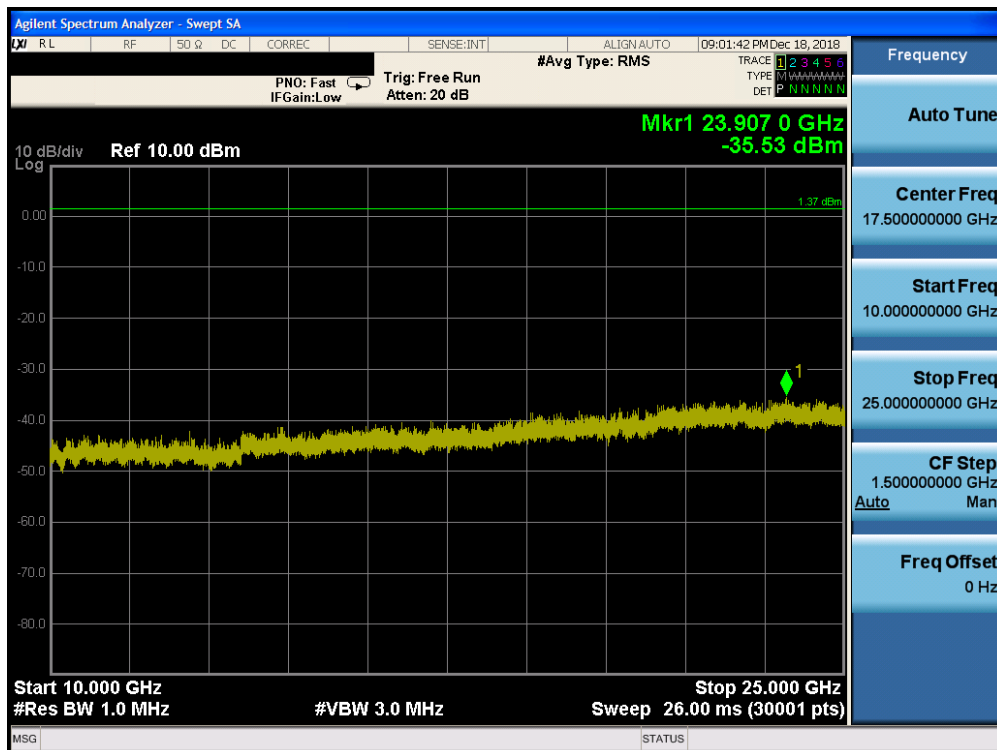
Plot 7-48. Conducted Spurious Plot ANT 0 (Bluetooth, GFSK, ePA Ch. 39)
