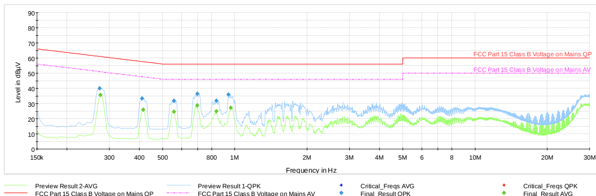
Plot 7-90. AC Line-Conducted Test Plot – GFSK ePA Ch.0 (L1, with AC/DC Adapter)
