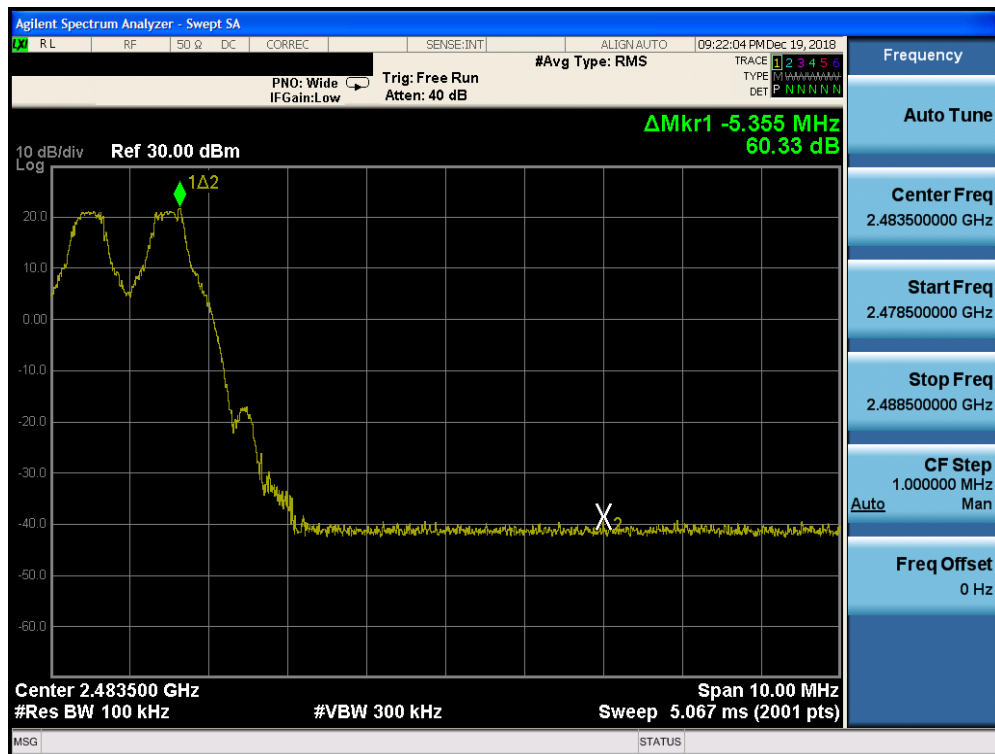
Plot 7-24. Band Edge Plot ANT 1 (Bluetooth with Hopping Enabled, GFSK, ePA)
