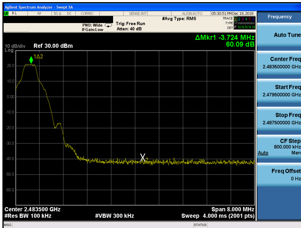
Plot 7-22. Band Edge Plot ANT 1 (Bluetooth with Hopping Disabled, GFSK, ePA – Ch. 78)
