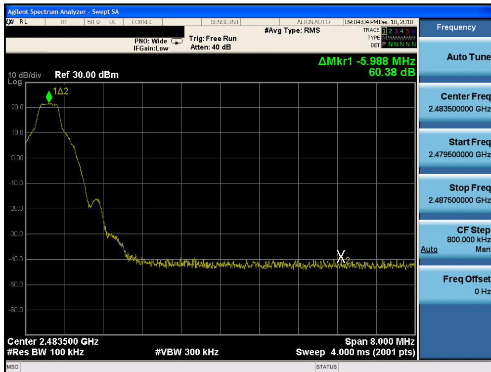
Plot 7-14. Band Edge Plot ANT 0 (Bluetooth with Hopping Disabled, GFSK, ePA – Ch. 78)
