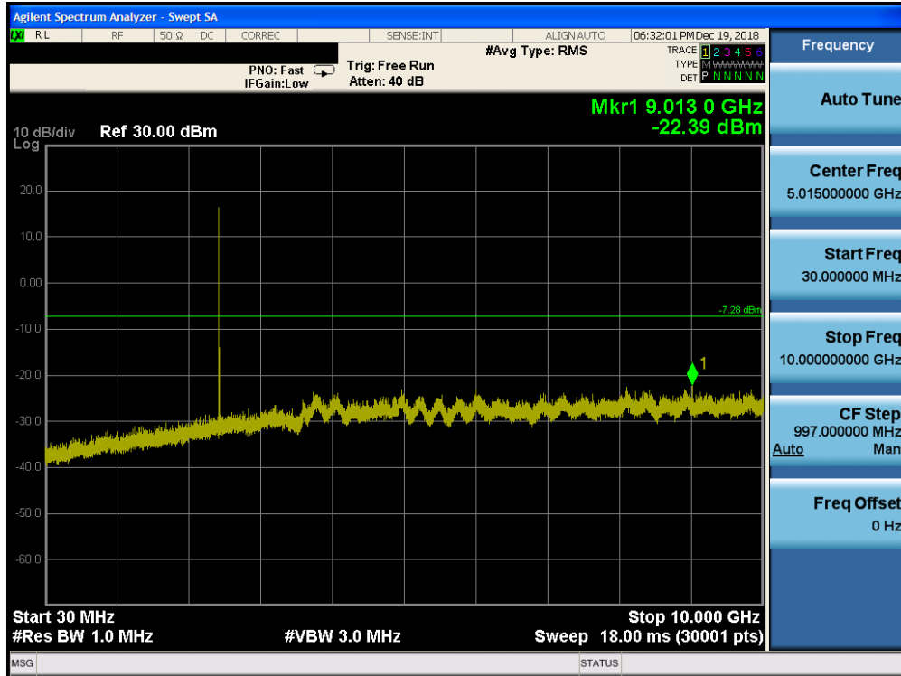
Plot 7-65. Conducted Spurious Plot ANT 1 (Bluetooth, 8DPSK, ePA – Ch. 39)
