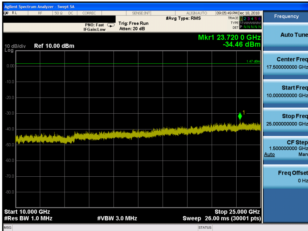
Plot 7-50. Conducted Spurious Plot ANT 0 (Bluetooth, GFSK, ePA – Ch. 78)
