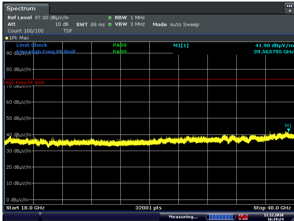
Plot 7-79. Radiated Spurious Plot 18GHz – 40GHz (2.4GHz – 5GHz) Pol. V
