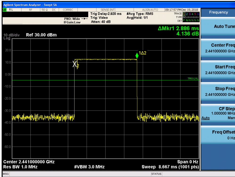
Plot 7-35. Time of Occupancy Plot ANT 1 (Bluetooth, GFSK, ePA)
