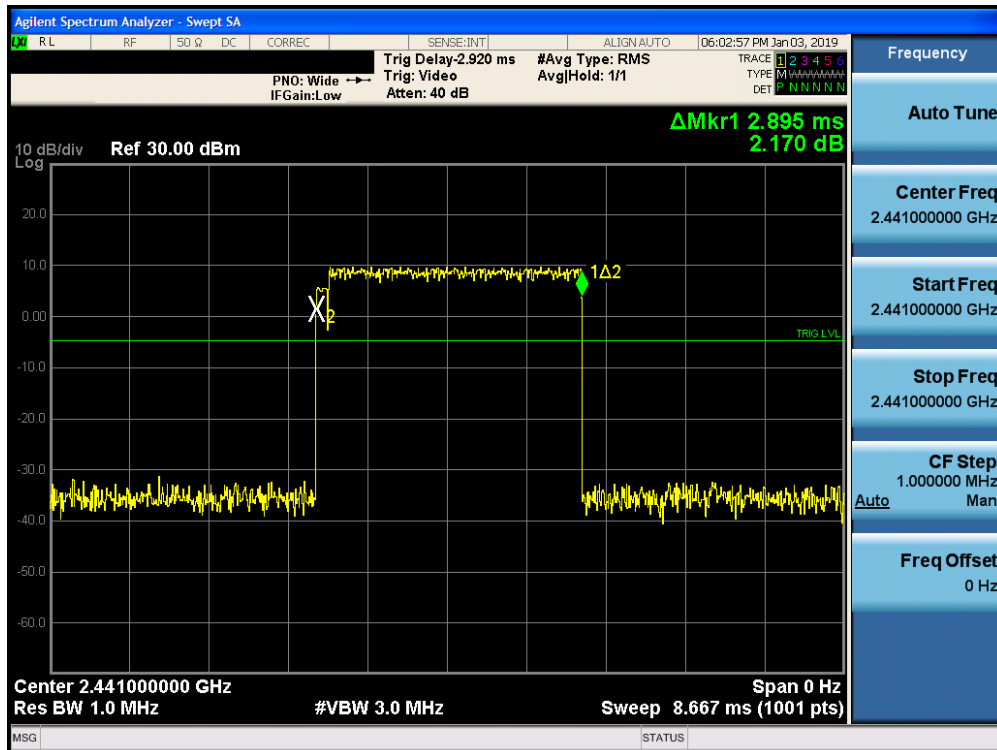
Plot 7-36. Time of Occupancy Plot ANT 1 (Bluetooth, 8DPSK, ePA)
