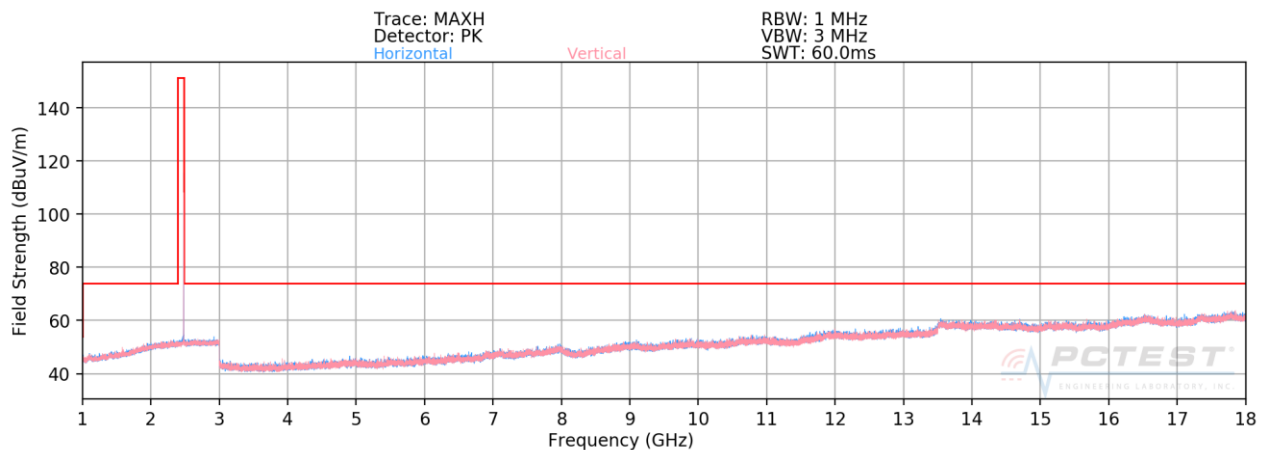
Plot 7-71. Radiated Spurious Plot above 1GHz ANT 0 (BT GFSK ePA – Ch. 78)
