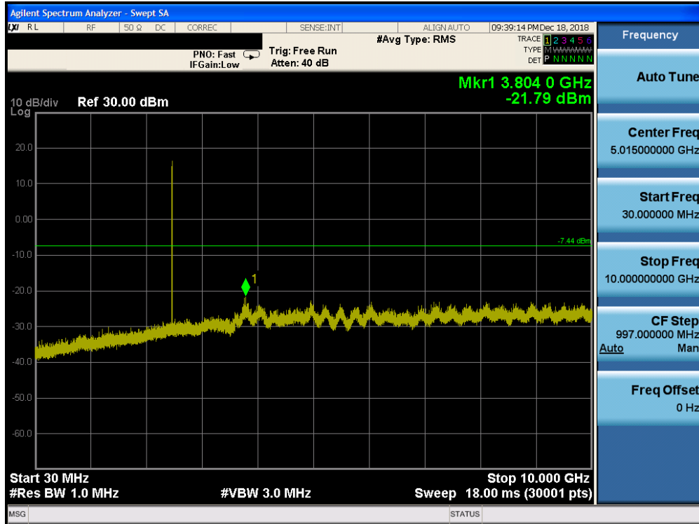
Plot 7-55. Conducted Spurious Plot ANT 0 (Bluetooth, 8DPSK, ePA – Ch. 78)
