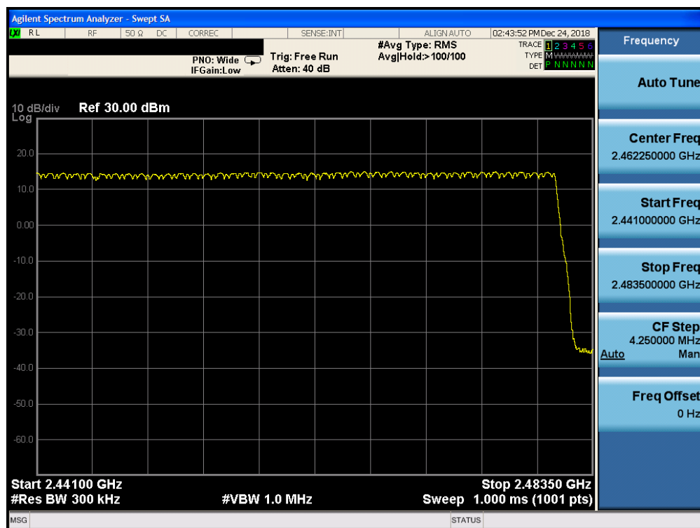
Plot 7-40. High End Spectrum Channel Hopping Plot ANT 0 (Bluetooth, 8DPSK, ePA)
