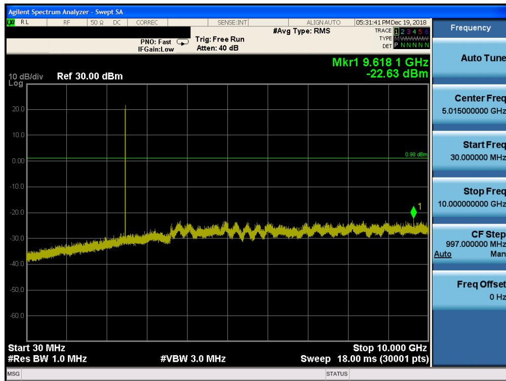
Plot 7-61. Conducted Spurious Plot ANT 1 (Bluetooth, GFSK, ePA – Ch. 78)
