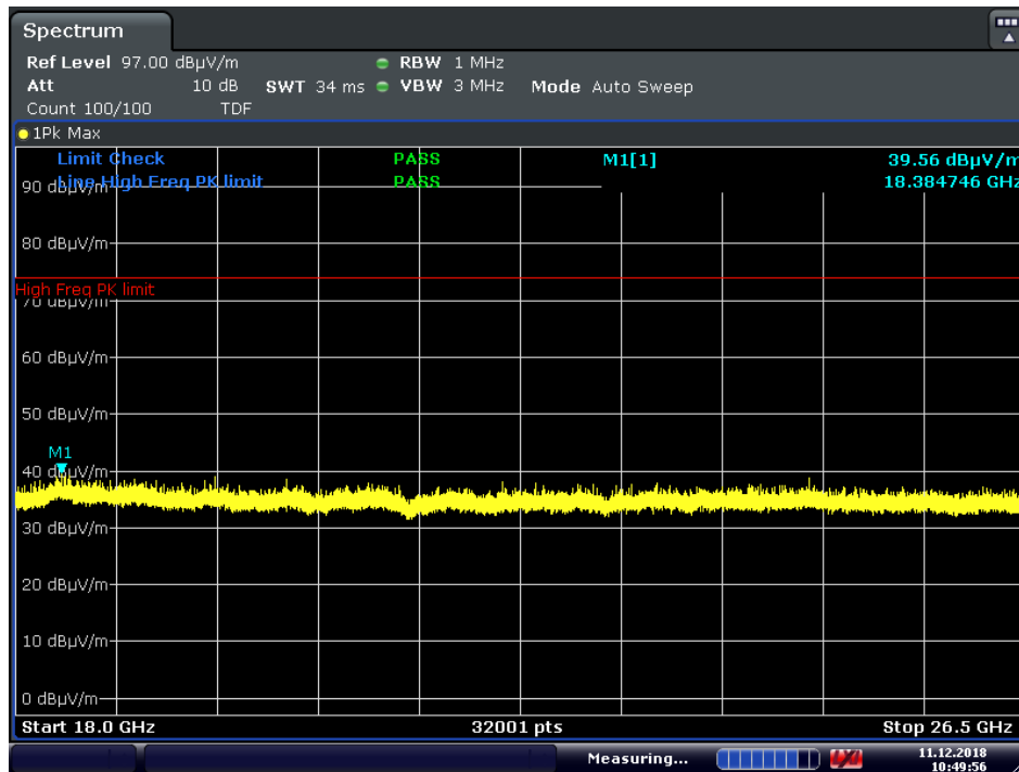
Plot 7-76. Radiated Spurious Plot above 18GHz ANT1 (GFSK ePA – Ch. 78, Pol. V)
