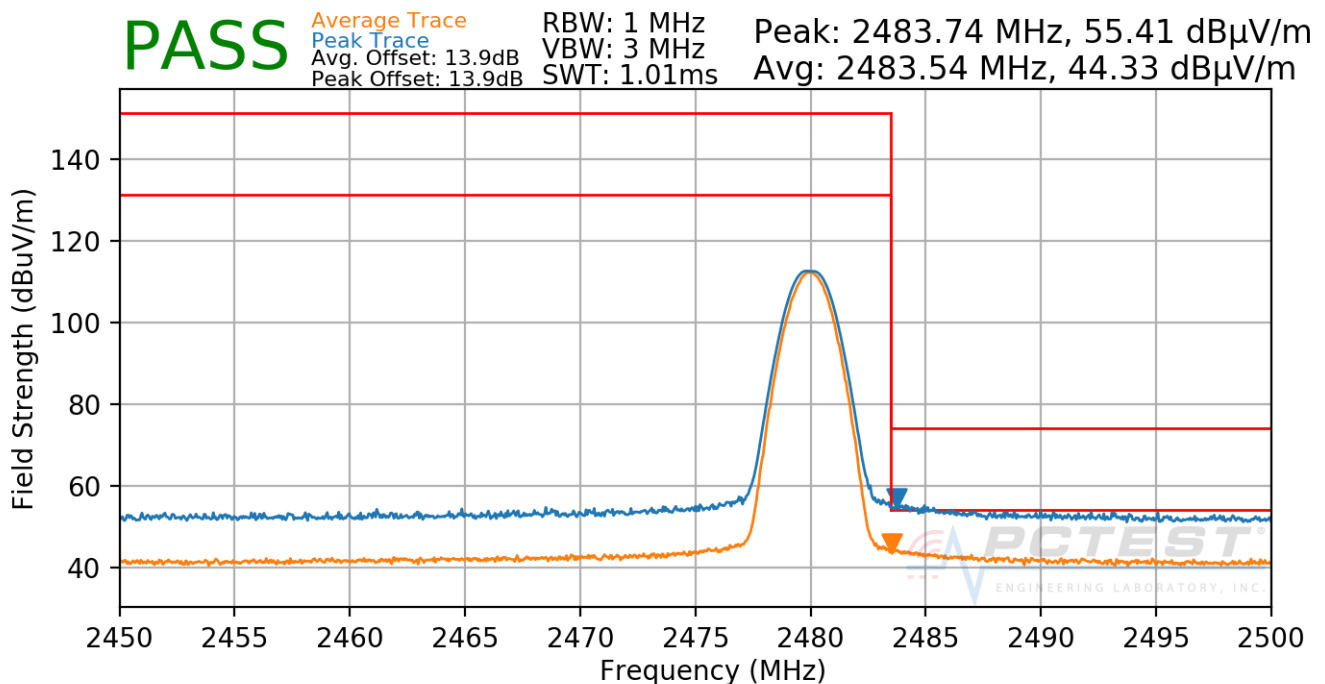
Plot 7-86. Radiated Restricted Upper Band Edge Measurement ANT 1
