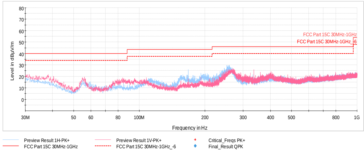
Plot 7-89. Radiated Spurious Plot below 1GHz (2.4GHz – 5GHz), with Laptop
