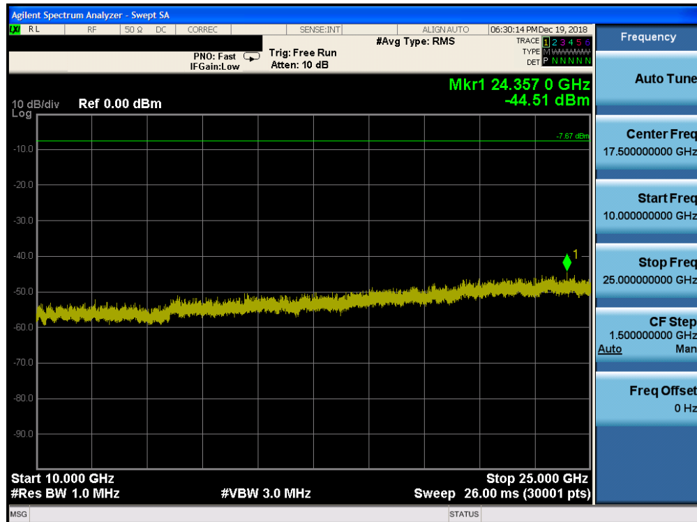
Plot 7-68. Conducted Spurious Plot ANT 1 (Bluetooth, 8DPSK, ePA – Ch. 78)
