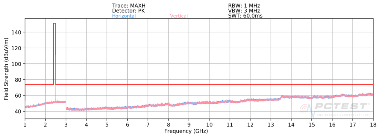
Plot 7-74. Radiated Spurious Plot above 1GHz ANT 1 (BT GFSK ePA – Ch. 78)
