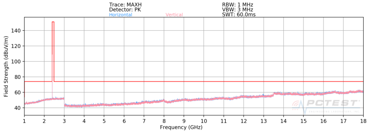
Plot 7-72. Radiated Spurious Plot above 1GHz ANT 1 (BT GFSK ePA – Ch. 0)
