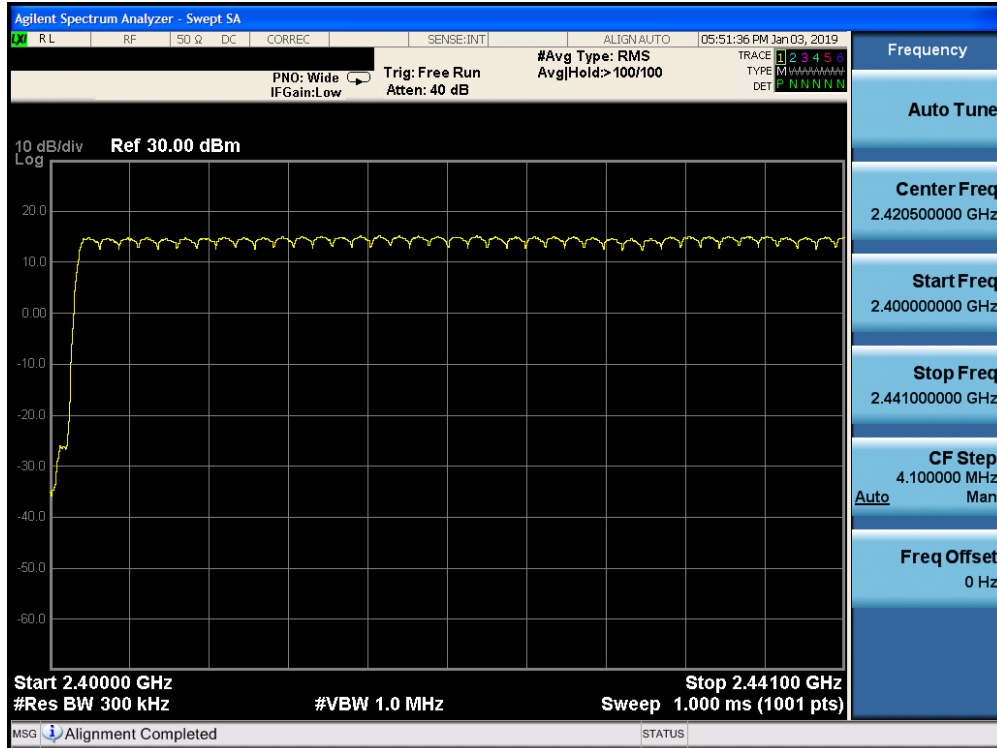
Plot 7-43. Low End Spectrum Channel Hopping Plot ANT 1 (Bluetooth, 8DPSK, ePA)
