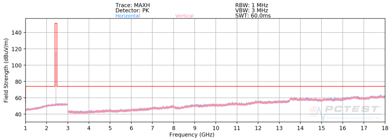
Plot 7-70. Radiated Spurious Plot above 1GHz ANT 0 (BT GFSK ePA – Ch. 39)
