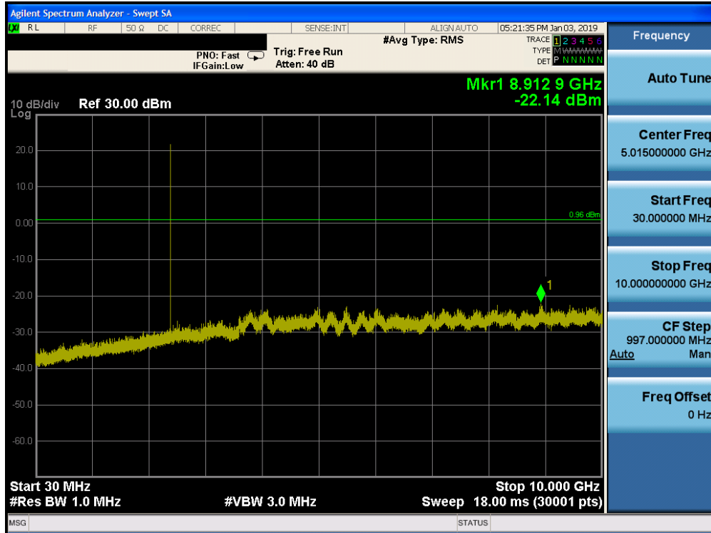
Plot 7-45. Conducted Spurious Plot ANT 0 (Bluetooth, GFSK, ePA – Ch. 0)
