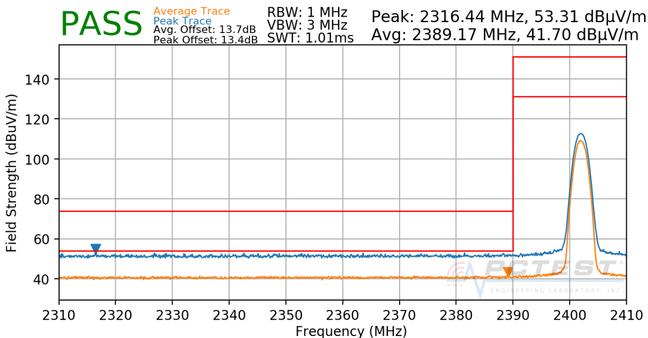
Plot 7-85. Radiated Restricted Lower Band Edge Measurement ANT 1
