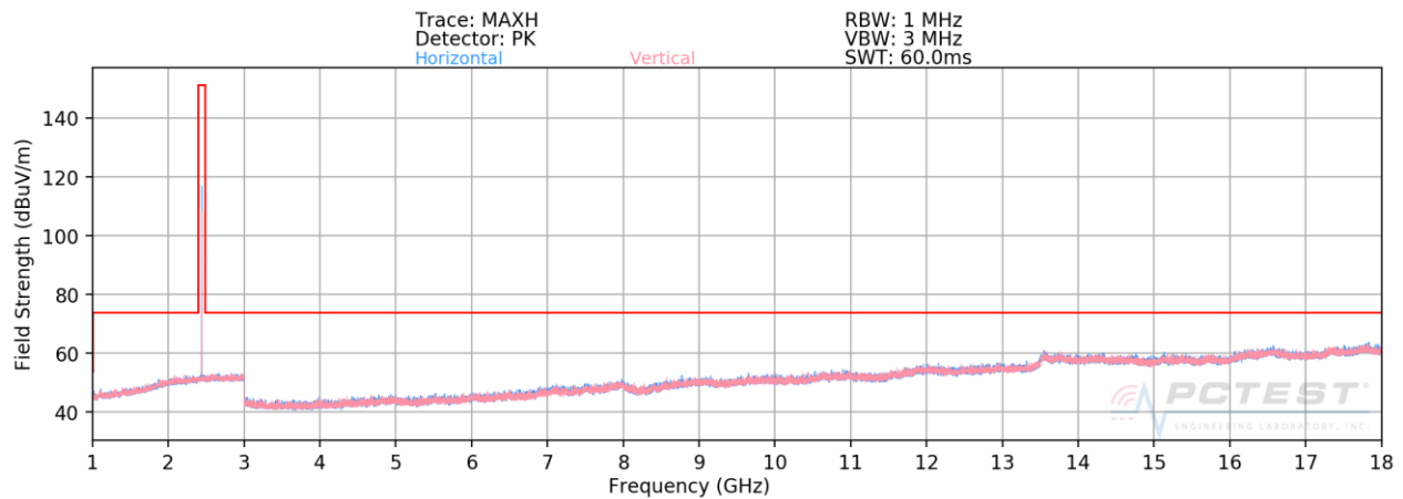
Plot 7-73. Radiated Spurious Plot above 1GHz ANT 1 (BT GFSK ePA – Ch. 39)
