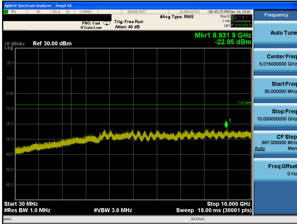
Plot 7-63. Conducted Spurious Plot ANT 1 (Bluetooth, 8DPSK, ePA – Ch. 0)
