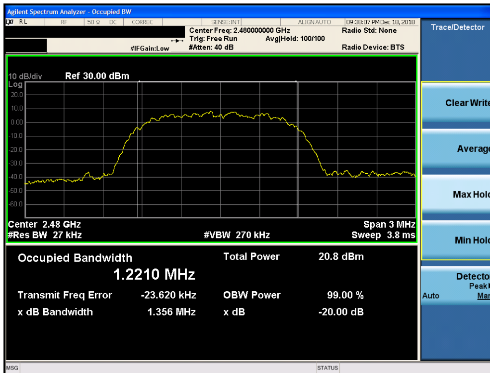
Plot 7-6. 20dB Bandwidth Plot ANT 0 (Bluetooth, 8DPSK, ePA – Ch. 78)
