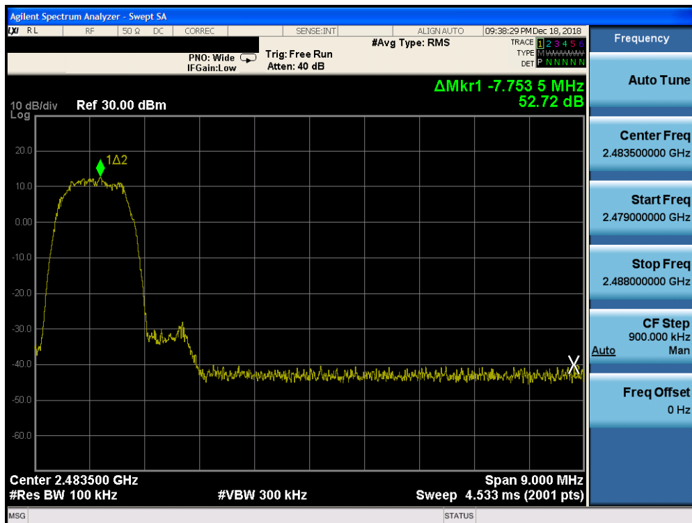
Plot 7-18. Band Edge Plot ANT 0 (Bluetooth with Hopping Disabled, 8DPSK, ePA – Ch. 78)
