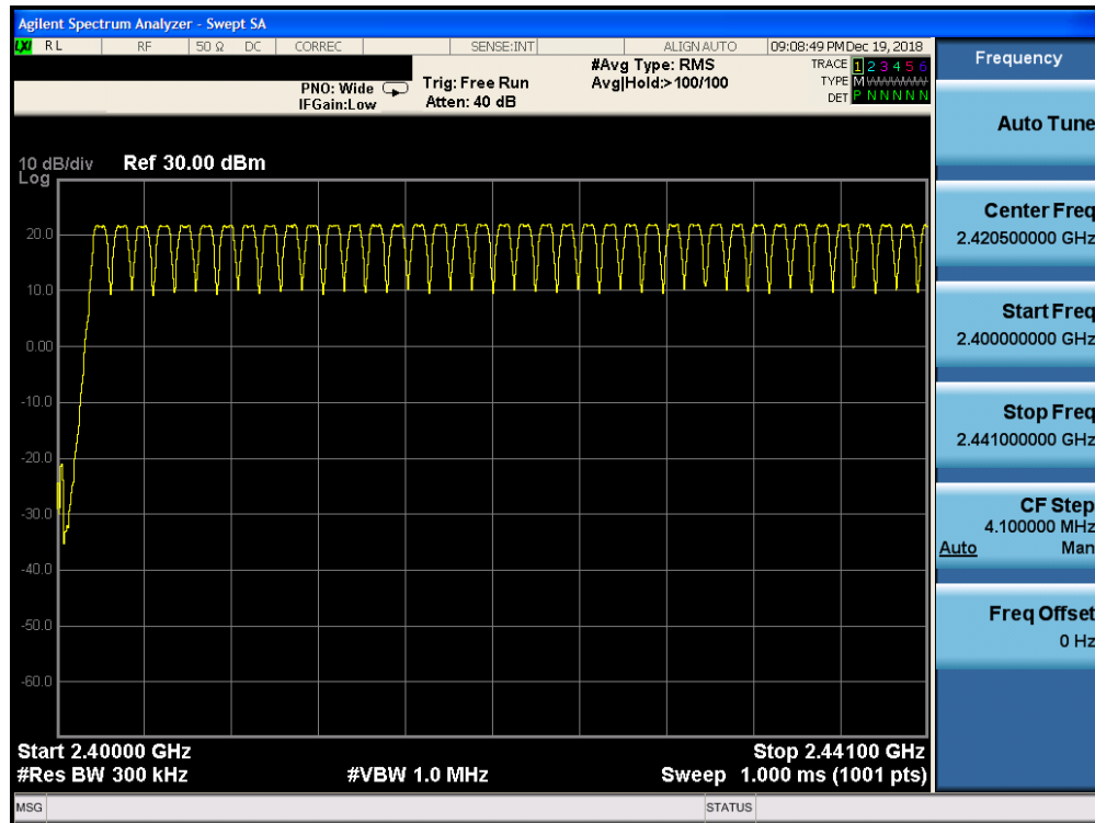
Plot 7-41. Low End Spectrum Channel Hopping Plot ANT 1 (Bluetooth, GFSK, ePA)
