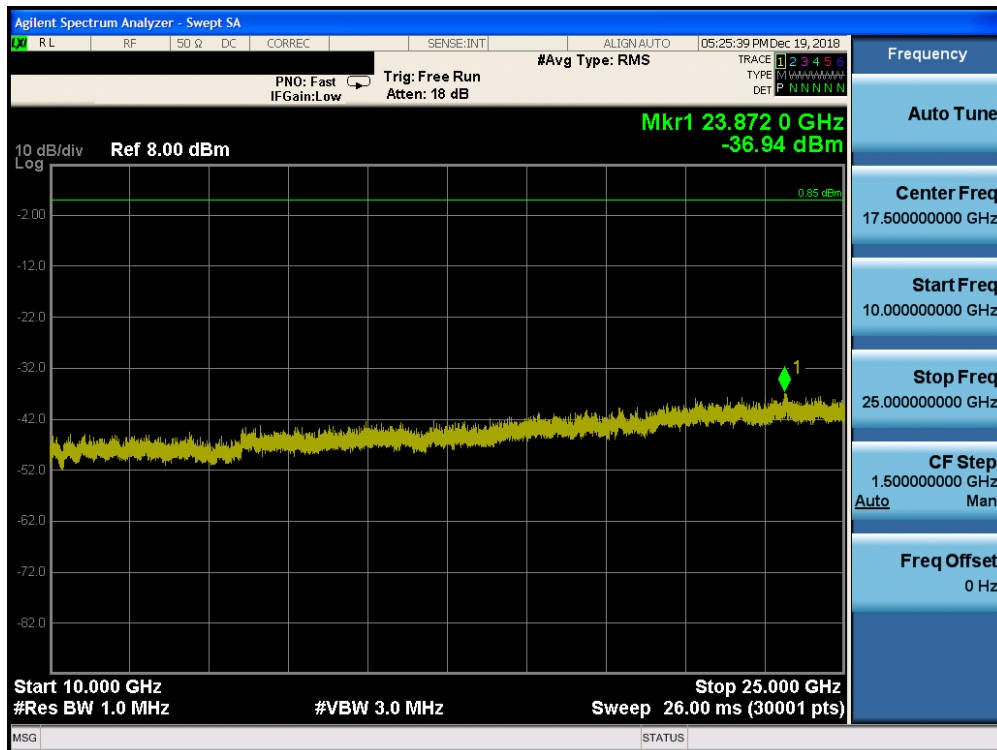
Plot 7-58. Conducted Spurious Plot ANT 1 (Bluetooth, GFSK, ePA – Ch. 0)
