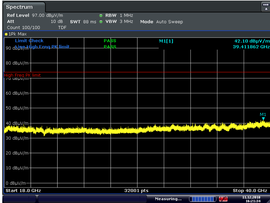
Plot 7-78. Radiated Spurious Plot 18GHz – 40GHz (2.4GHz – 5GHz) Pol. H
