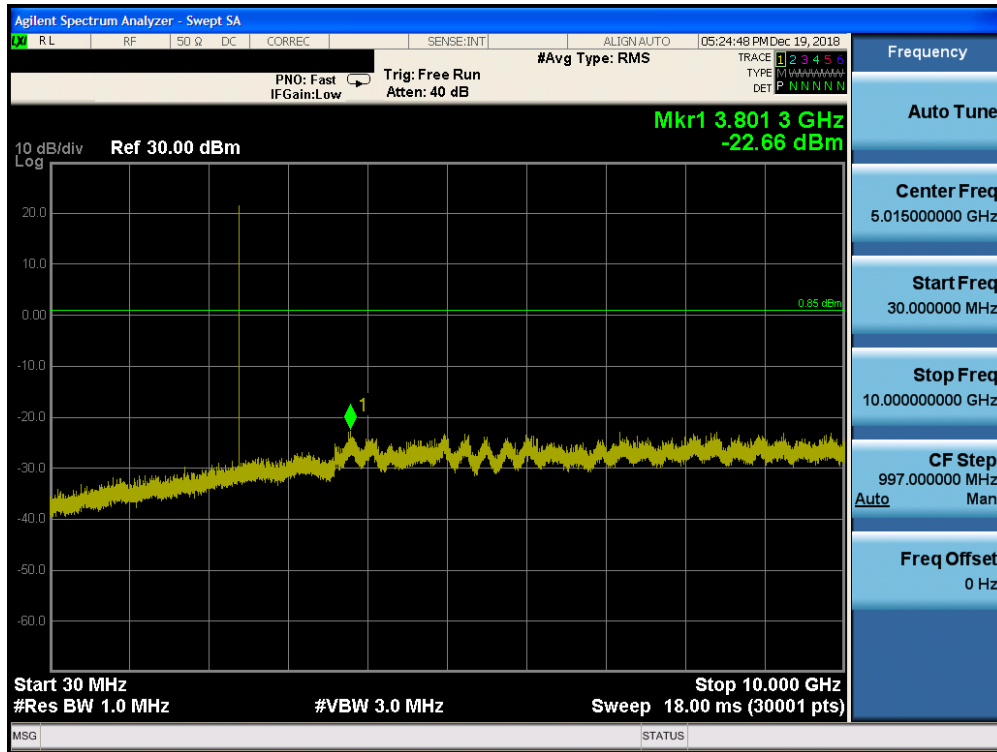
Plot 7-57. Conducted Spurious Plot ANT 1 (Bluetooth, GFSK, ePA – Ch. 0)
