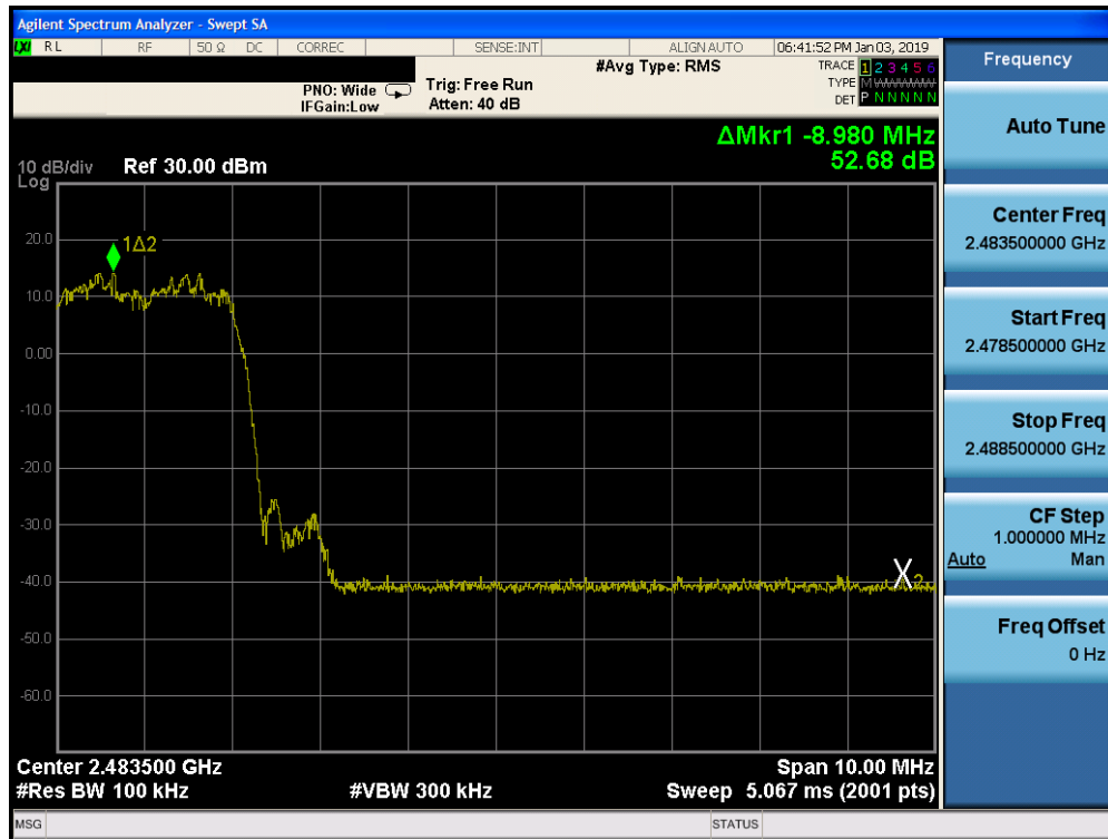
Plot 7-28. Band Edge Plot ANT 1 (Bluetooth with Hopping Enabled, 8DPSK, ePA)
