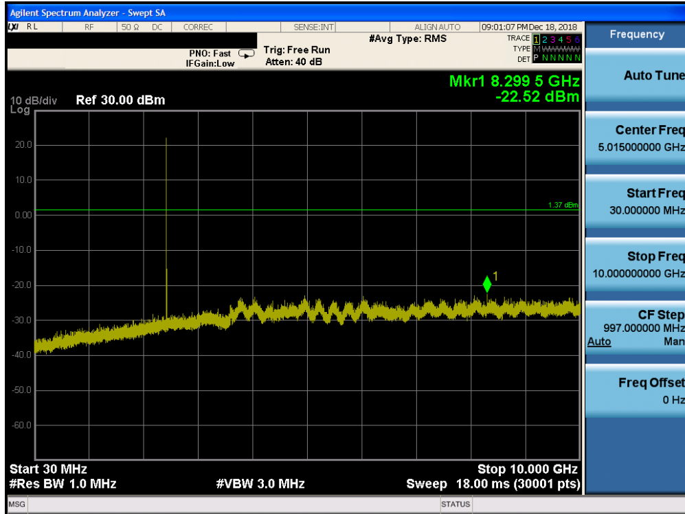
Plot 7-47. Conducted Spurious Plot ANT 0 (Bluetooth, GFSK, ePA – Ch. 39)
