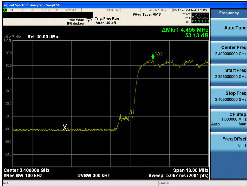
Plot 7-27. Band Edge Plot ANT 1 (Bluetooth with Hopping Enabled, 8DPSK, ePA)
