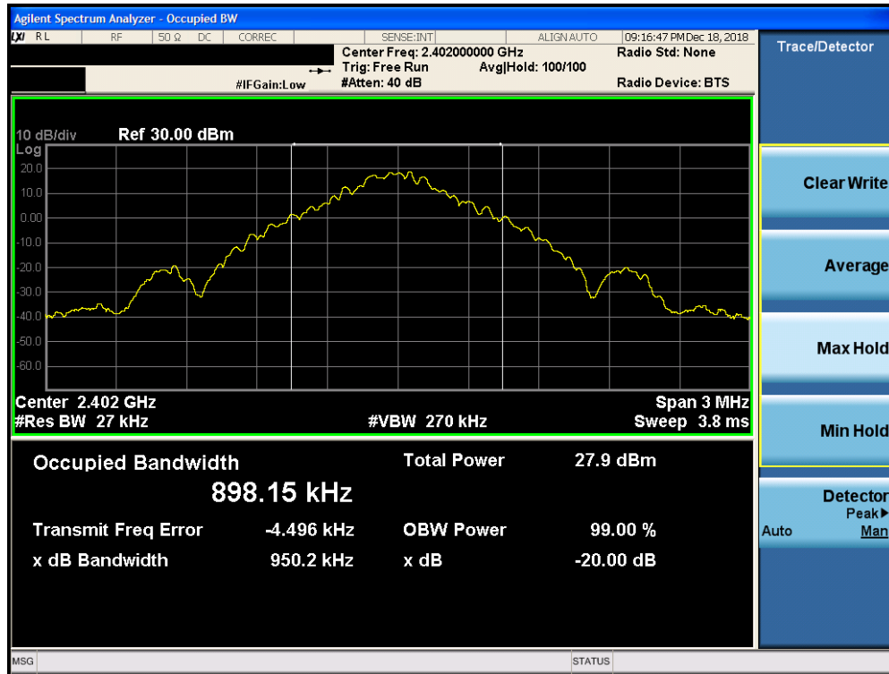
Plot 7-1. 20dB Bandwidth Plot ANT 0 (Bluetooth, GFSK, ePA – Ch. 0)
