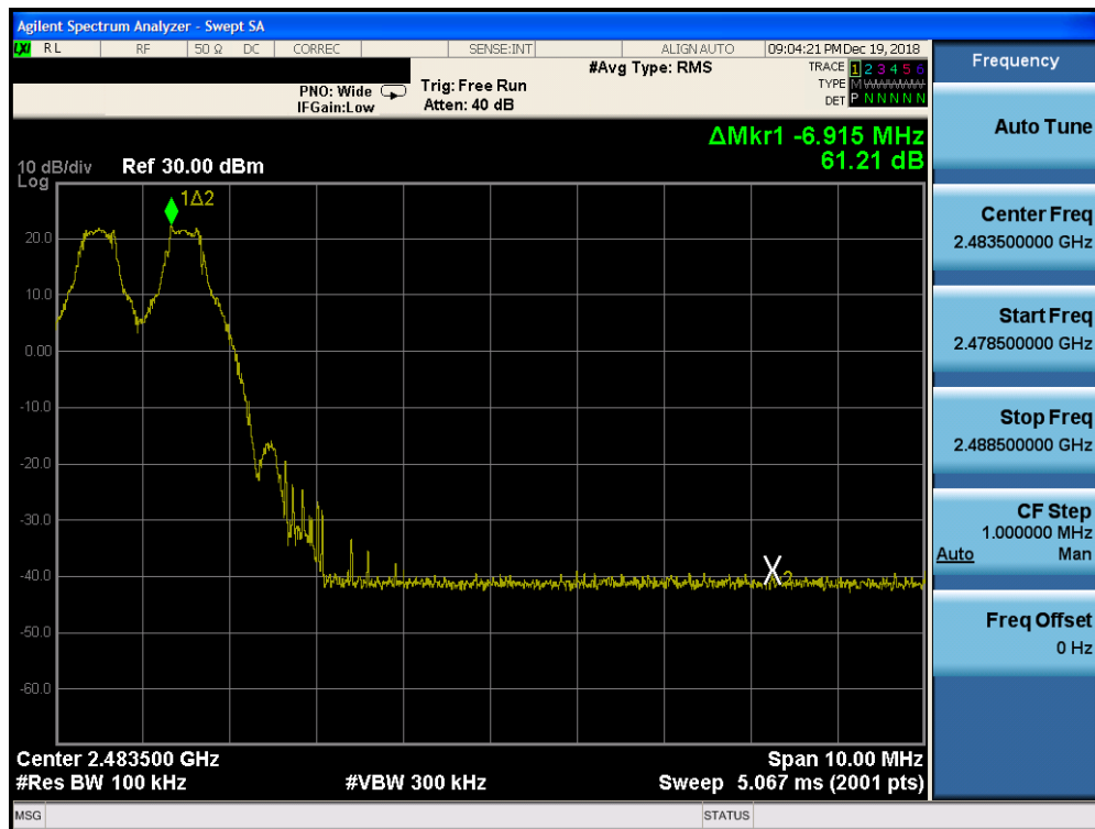
Plot 7-16. Band Edge Plot ANT 0 (Bluetooth with Hopping Enabled, GFSK, ePA)
