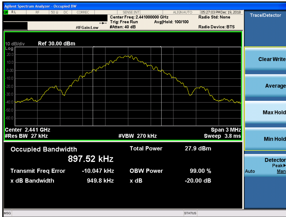
Plot 7-8. 20dB Bandwidth Plot ANT 1 (Bluetooth, GFSK, ePA – Ch. 39)
