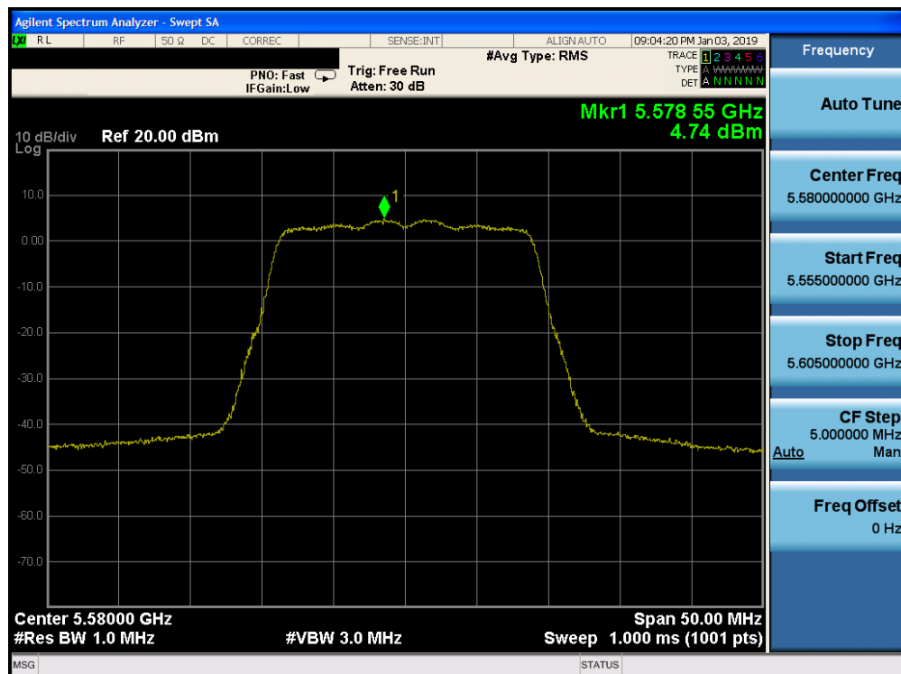
Plot 7-66. Power Spectral Density Plot SISO CORE0 (20MHz BW 802.11n (UNII Band 2C) – Ch. 116)
