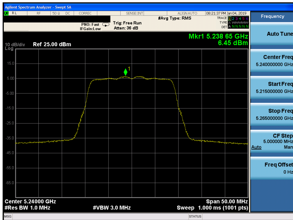
Plot 7-81. Power Spectral Density Plot SISO CORE1 (20MHz BW 802.11n (UNII Band 1) – Ch. 48) - ISED
