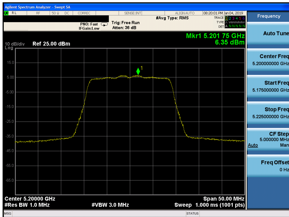
Plot 7-80. Power Spectral Density Plot SISO CORE1 (20MHz BW 802.11n (UNII Band 1) – Ch. 40) - ISED
