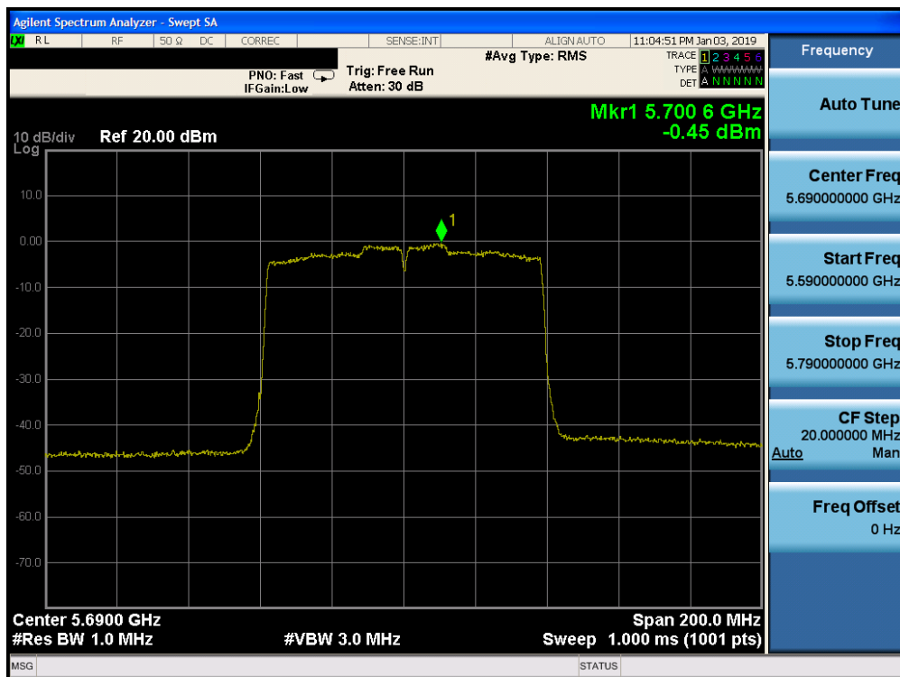
Plot 7-72. Power Spectral Density Plot SISO CORE0 (80MHz BW 802.11ac (UNII Band 2C) – Ch. 138)
