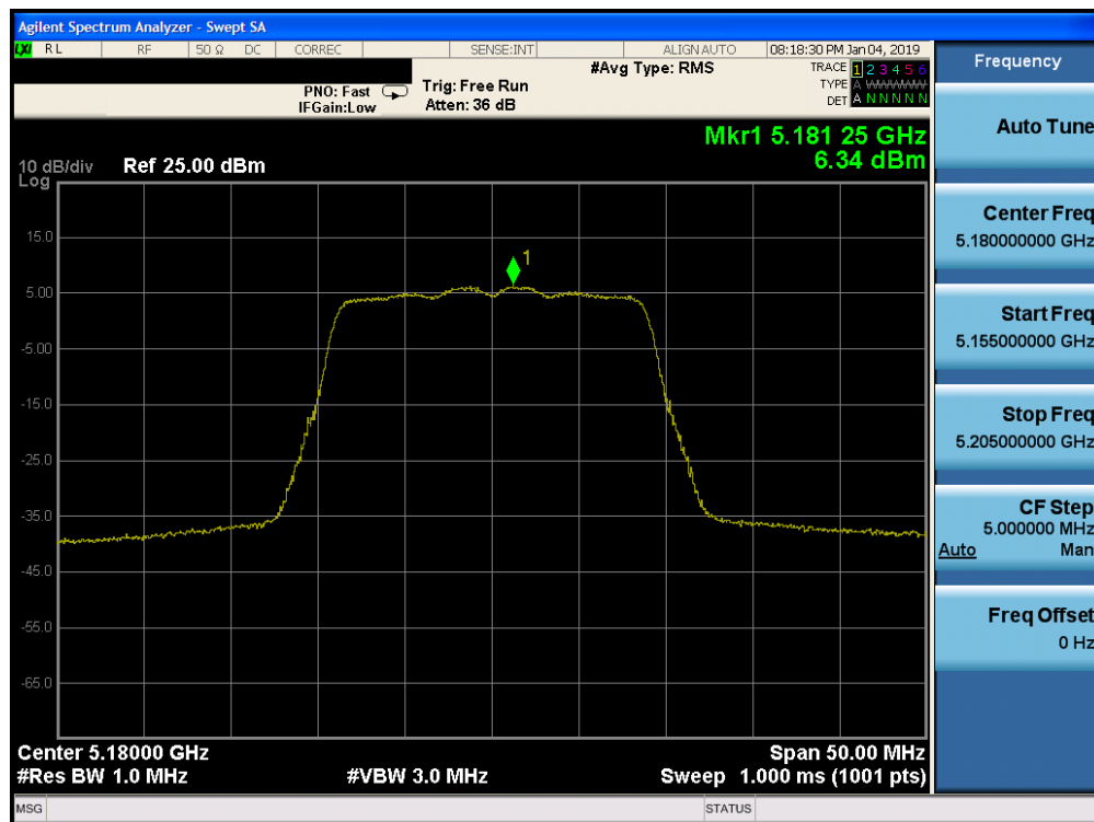
Plot 7-79. Power Spectral Density Plot SISO CORE1 (20MHz BW 802.11n (UNII Band 1) – Ch. 36) - ISED
