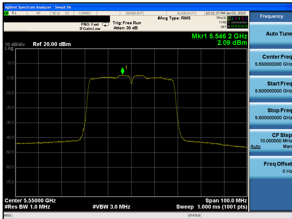
Plot 7-69. Power Spectral Density Plot SISO CORE0 (40MHz BW 802.11n (UNII Band 2C) – Ch. 110)
