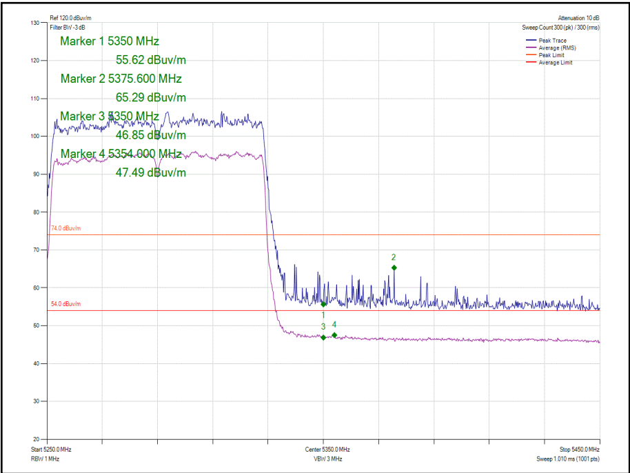
Figure 1122 - 802.11ac VHT80 SDM Cores 0-1 - 5290 MHz Band Edge Frequency 5350 MHz
