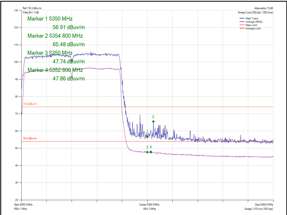
Figure 1123 - 802.11ac VHT80 TxBF Cores 0-1 - 5290 MHz Band Edge Frequency 5350 MHz
