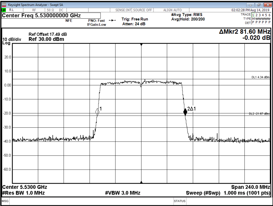
Figure 515 - 5530 MHz - 26 dB Emission Bandwidth
