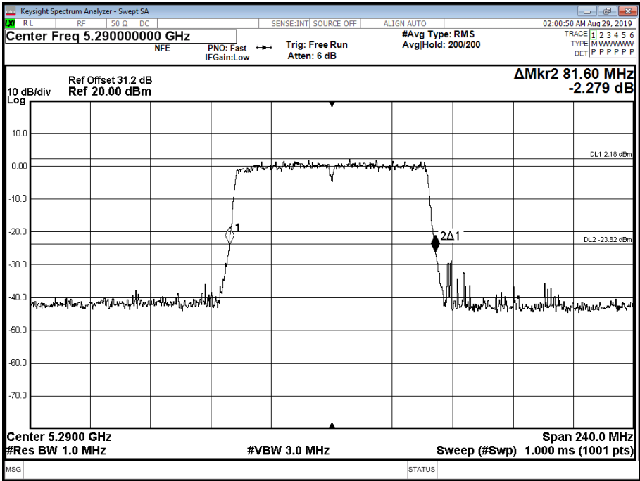
Figure 345 - 5290 MHz - 26 dB Emission Bandwidth
