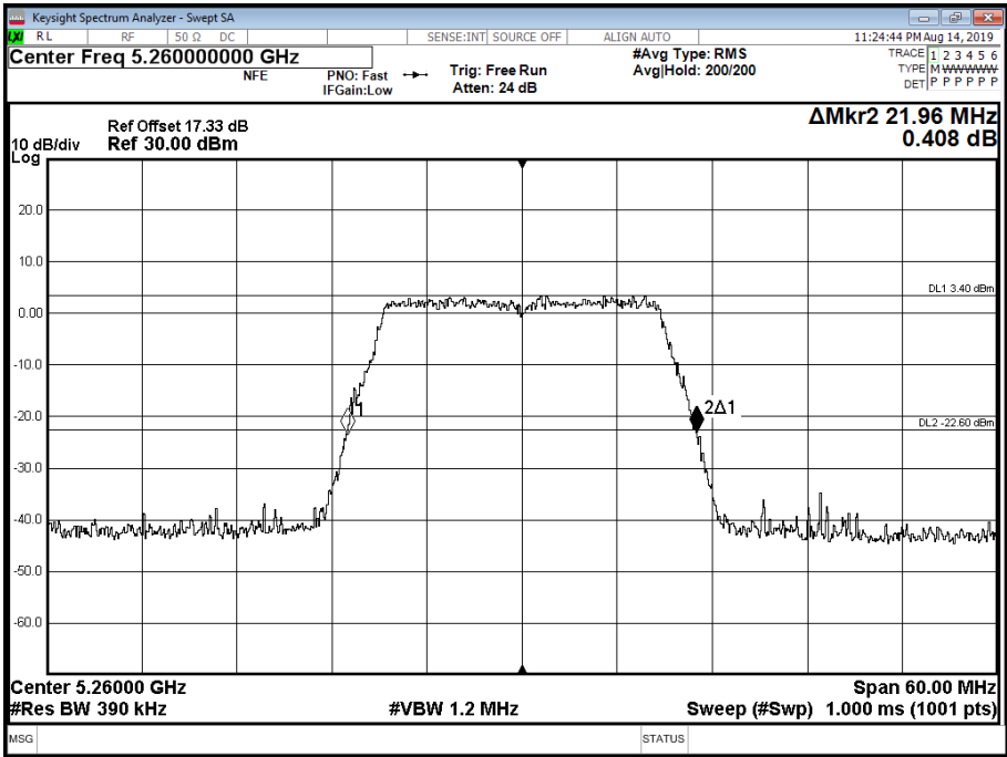
Figure 285 - 5260 MHz - 26 dB Emission Bandwidth
