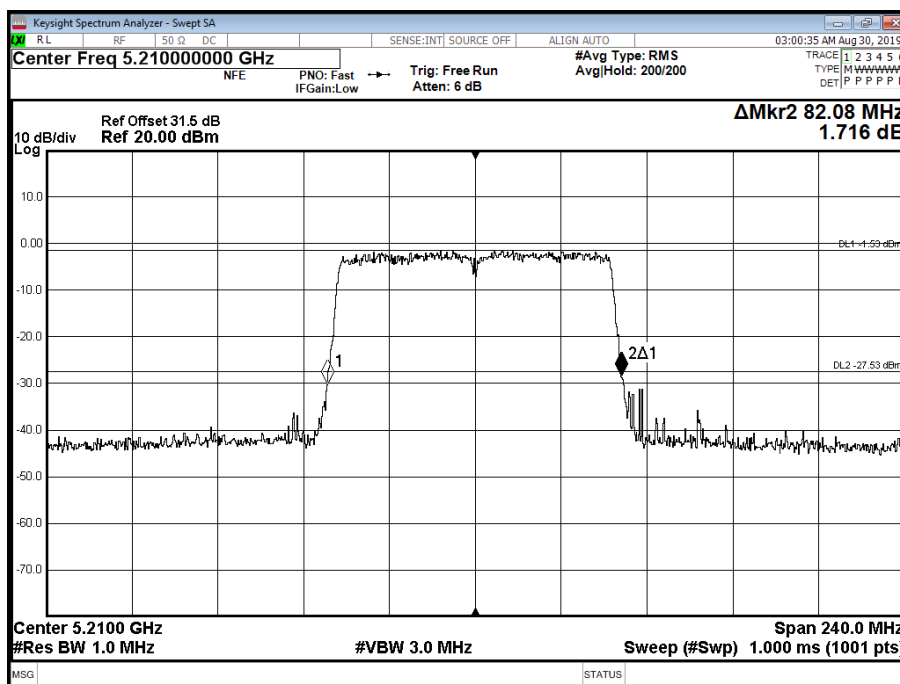
Figure 231 - 5210 MHz - 26 dB Emission Bandwidth
