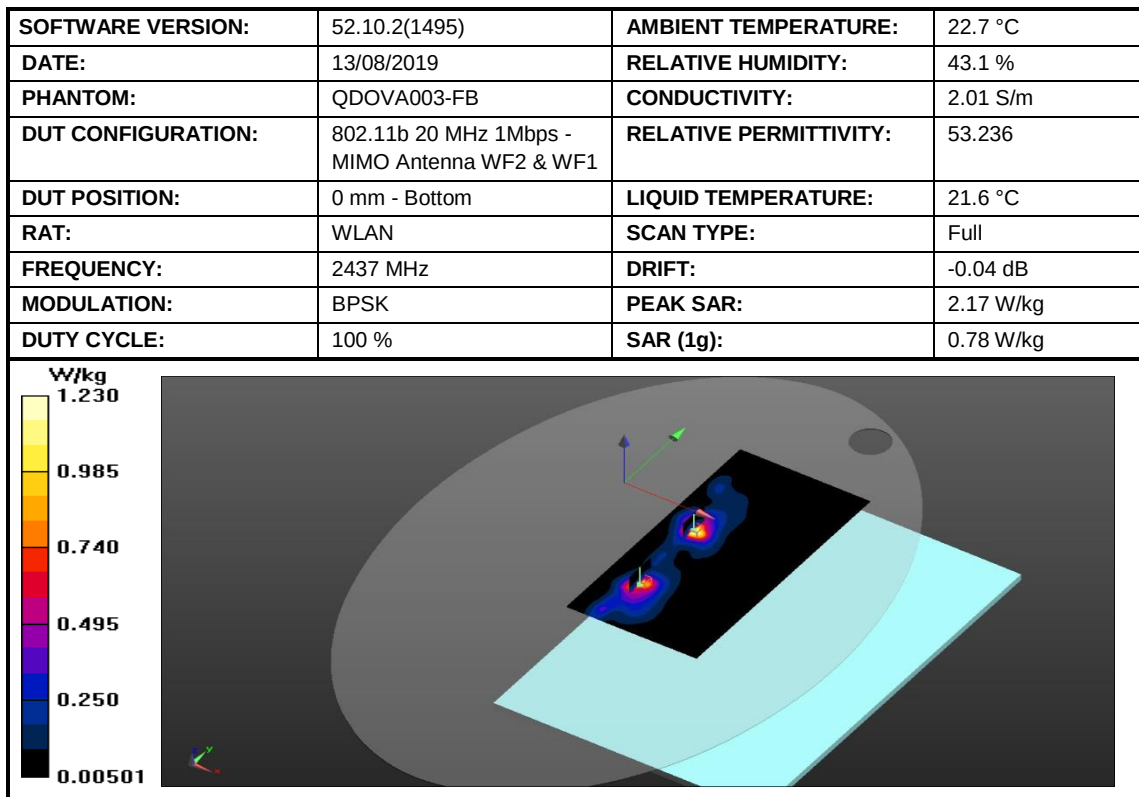
Figure 13: SAR Body Testing Results for the A2141 at 2437 MHz.
