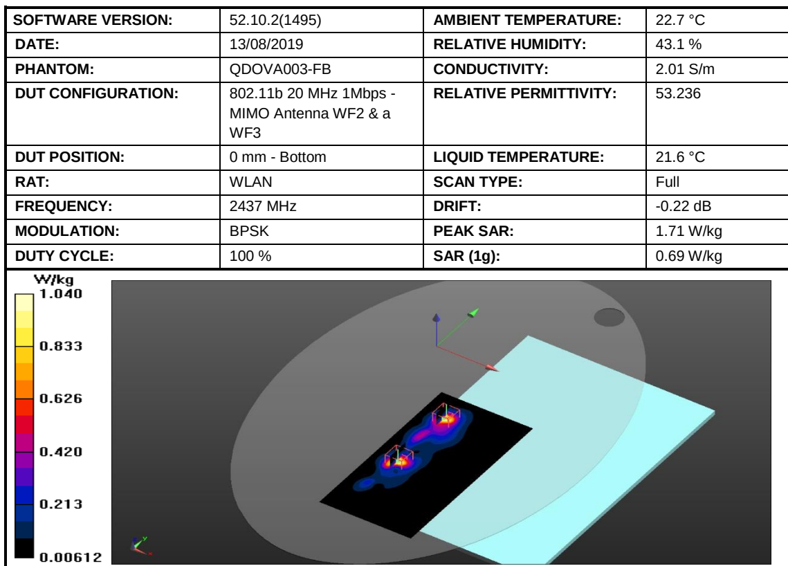
Figure 14: SAR Body Testing Results for the A2141 at 2437 MHz.
