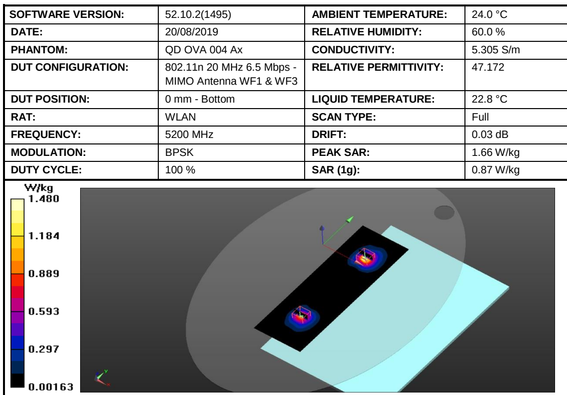
Figure 29: SAR Body Testing Results for the A2141 at 5200 MHz.
