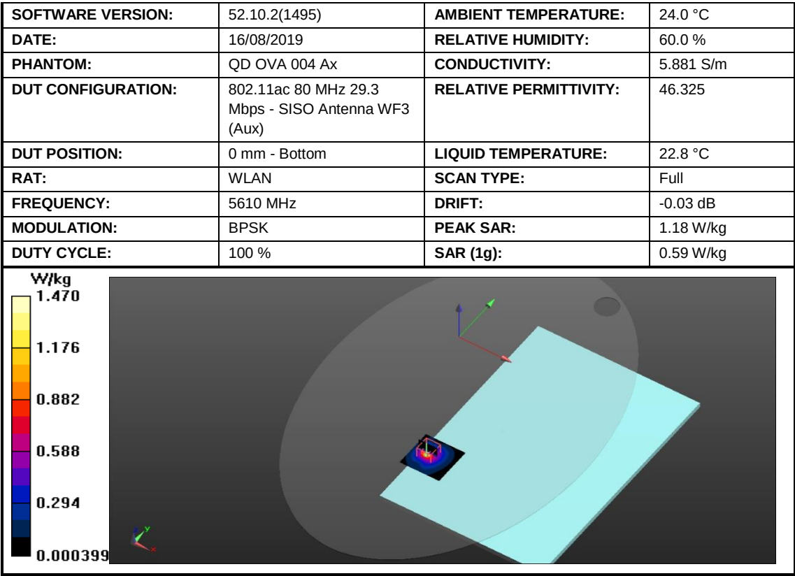
Figure 39: SAR Body Testing Results for the A2141 at 5610 MHz.
