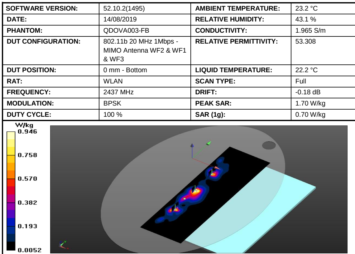
Figure 16: SAR Body Testing Results for the A2141 at 2437 MHz.
