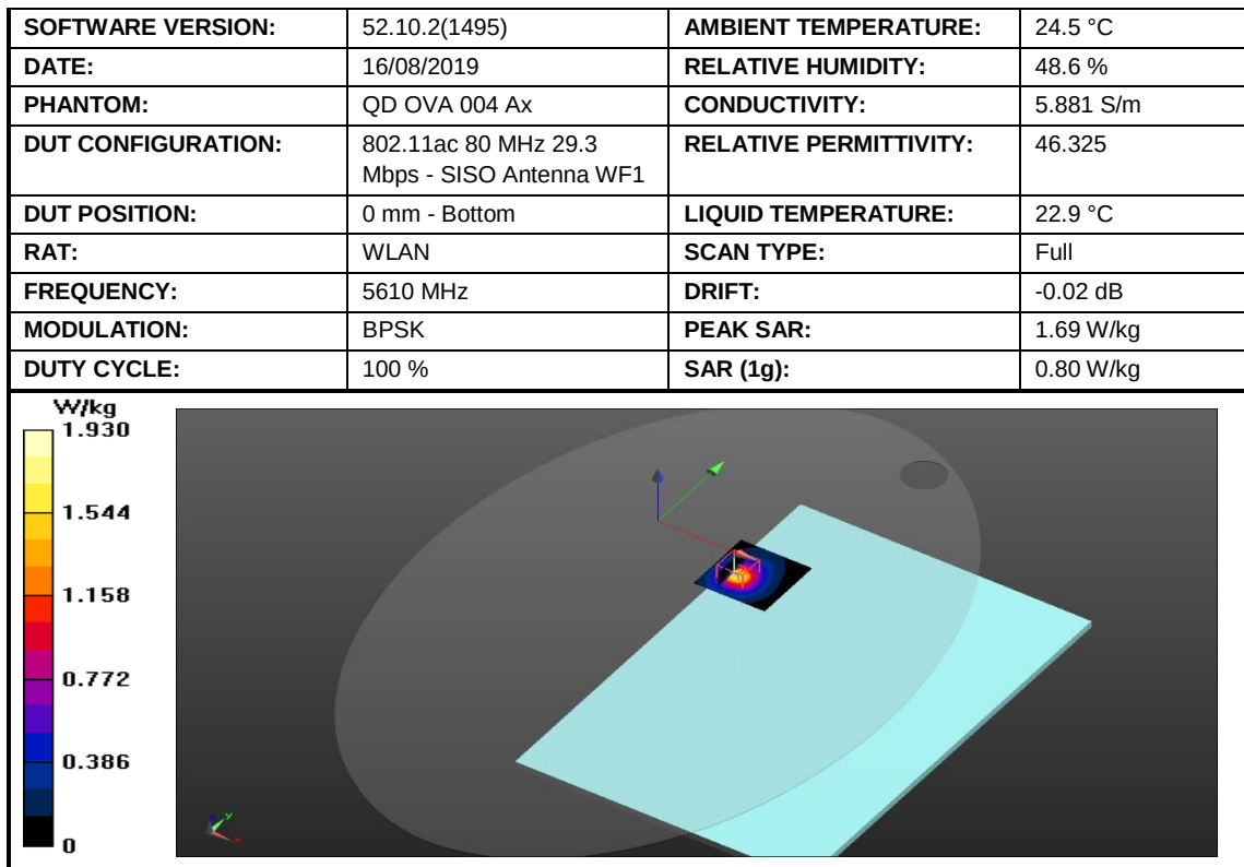
Figure 35: SAR Body Testing Results for the A2141 at 5610 MHz.
