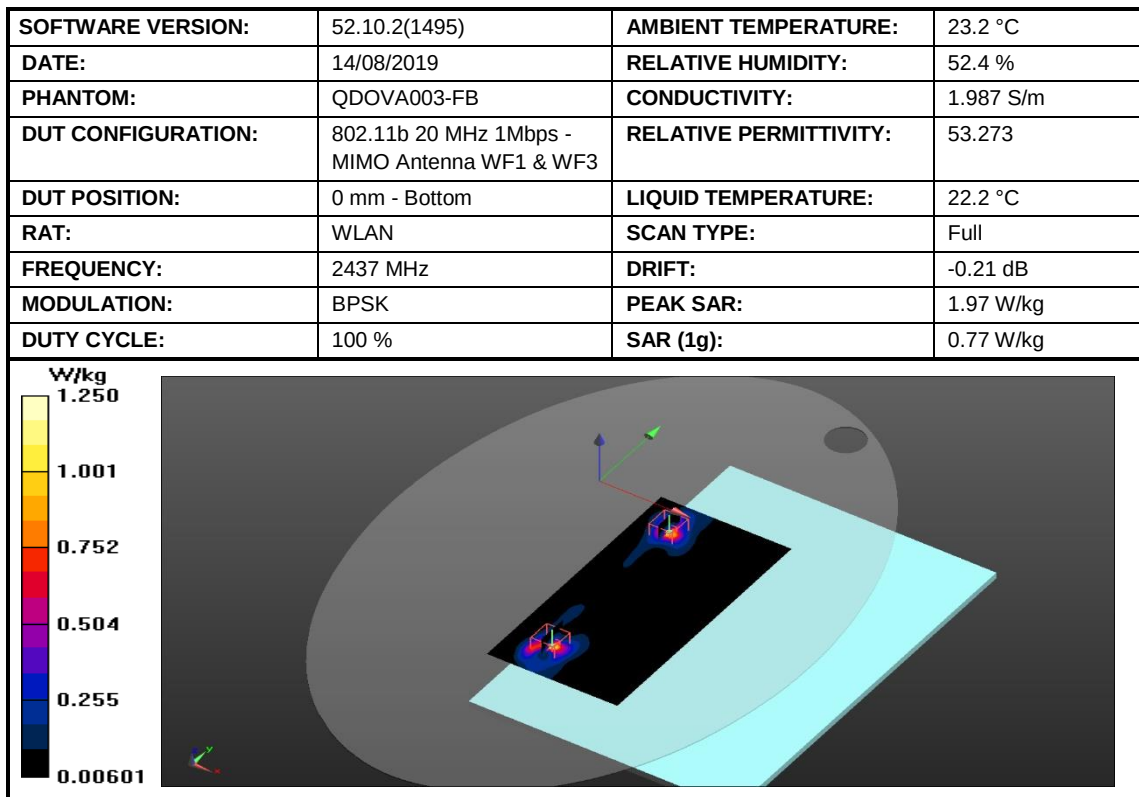
Figure 15: SAR Body Testing Results for the A2141 at 2437 MHz.
