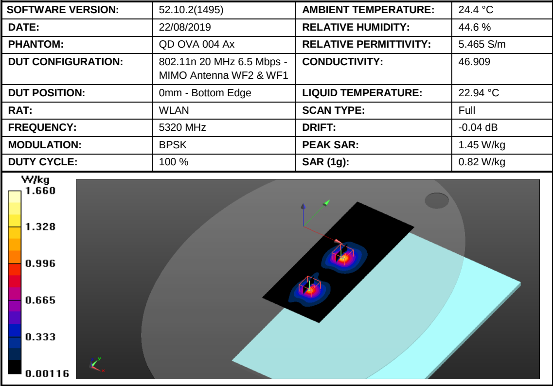
Figure 57: SAR Body Testing Results for the A2141 at 5320 MHz.
