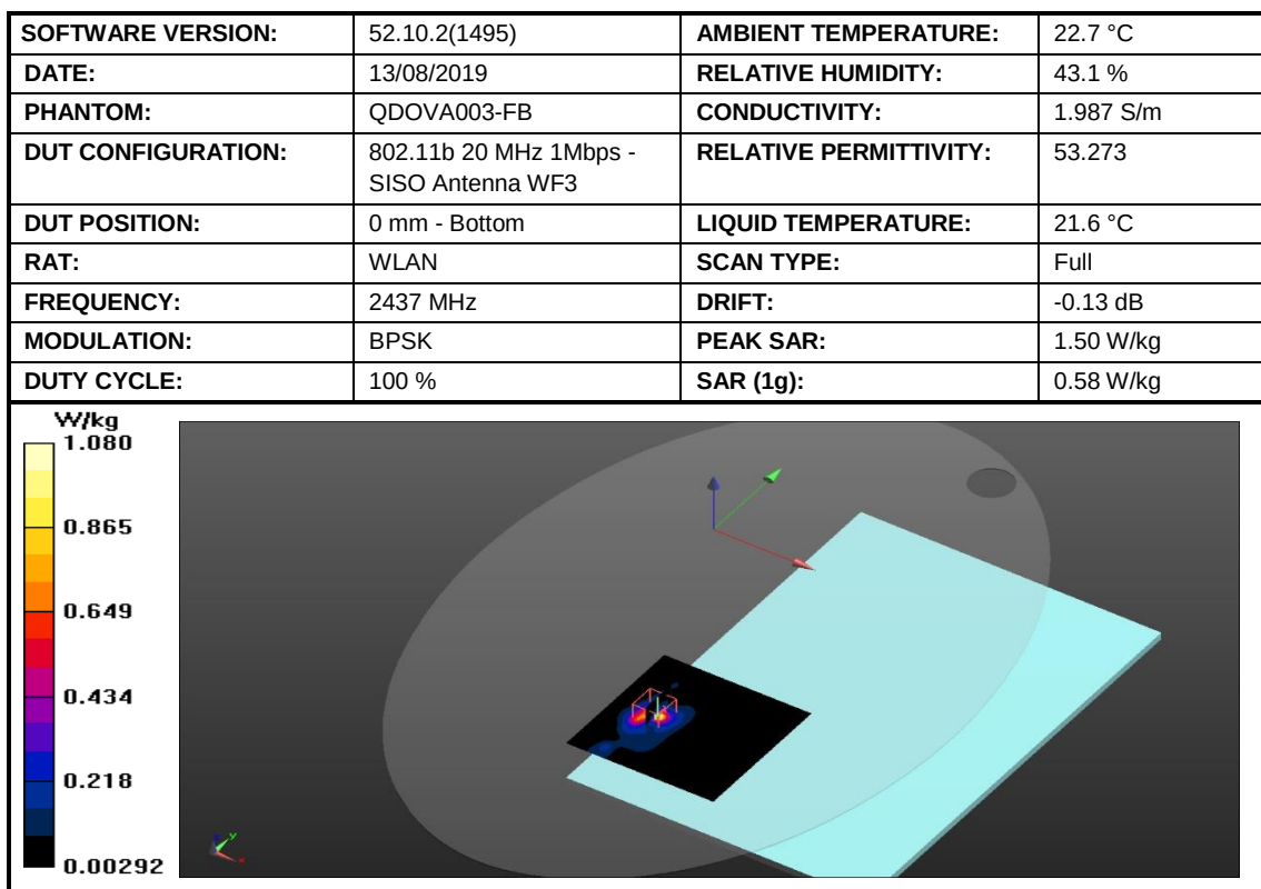
Figure 9: SAR Body Testing Results for the A2141 at 2437 MHz.
