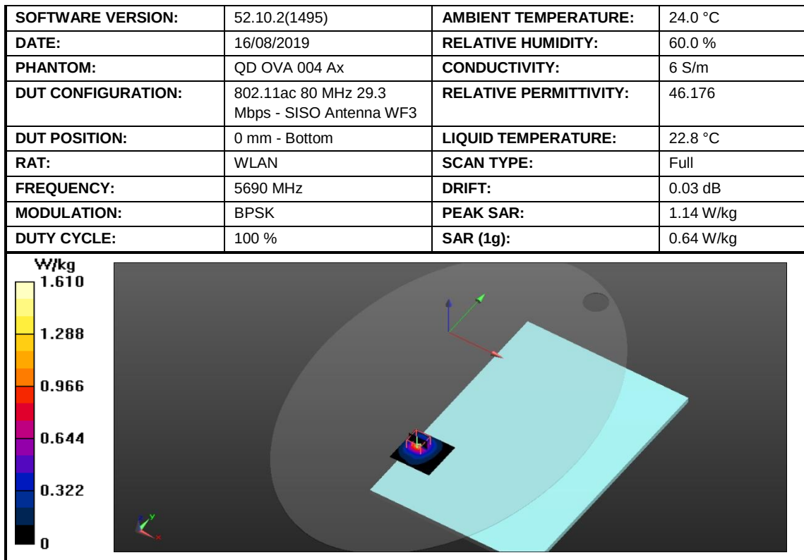
Figure 37: SAR Body Testing Results for the A2141 at 5690 MHz.
