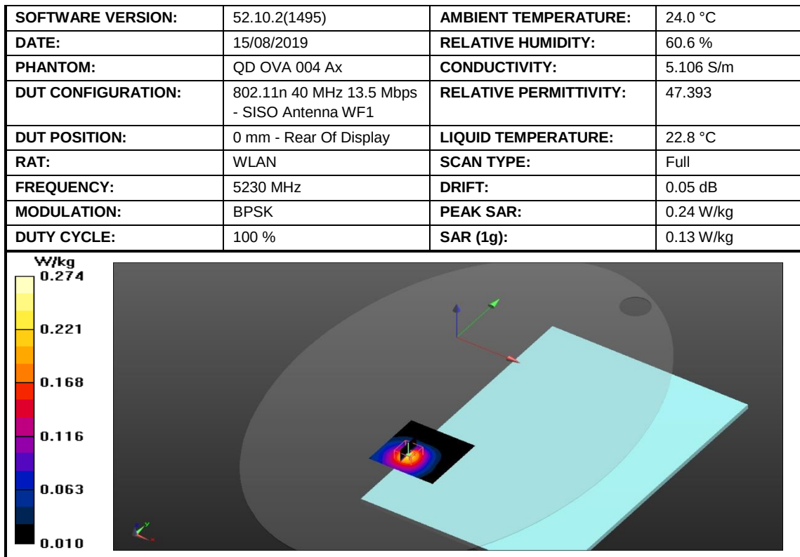
Figure 20: SAR Body Testing Results for the A2141 at 5230 MHz.
