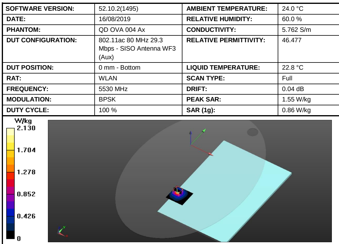
Figure 38: SAR Body Testing Results for the A2141 at 5530 MHz.
