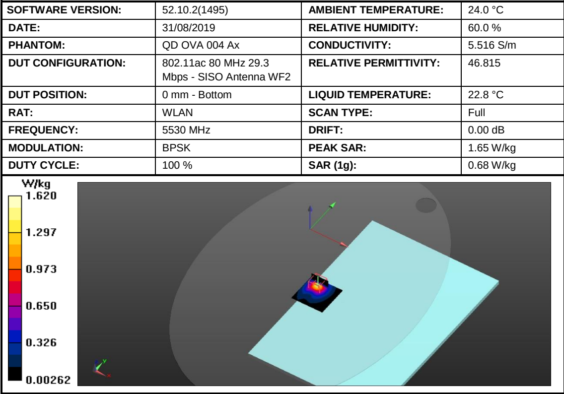
Figure 34: SAR Body Testing Results for the A2141 at 5530 MHz.
