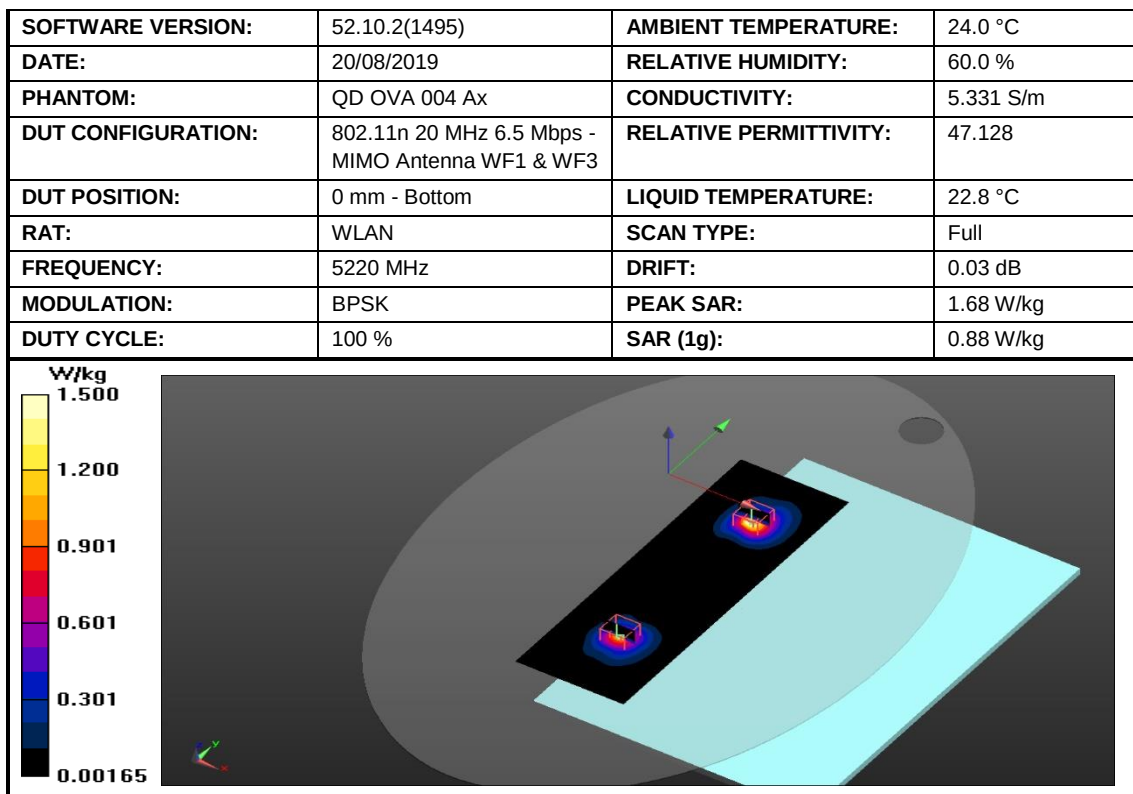
Figure 27: SAR Body Testing Results for the A2141 at 5220 MHz.
