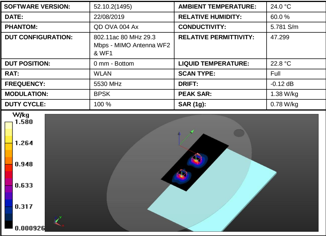
Figure 43: SAR Body Testing Results for the A2141 at 5530 MHz.
