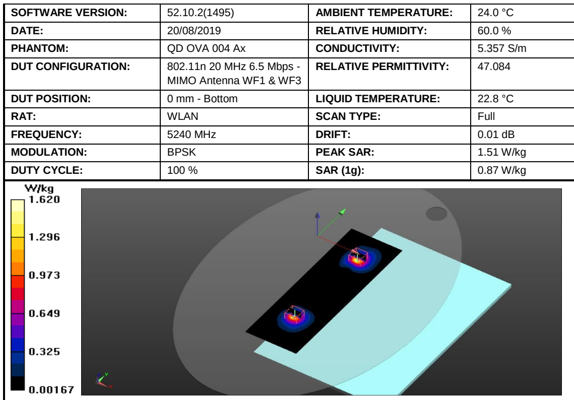
Figure 28: SAR Body Testing Results for the A2141 at 5240 MHz.
