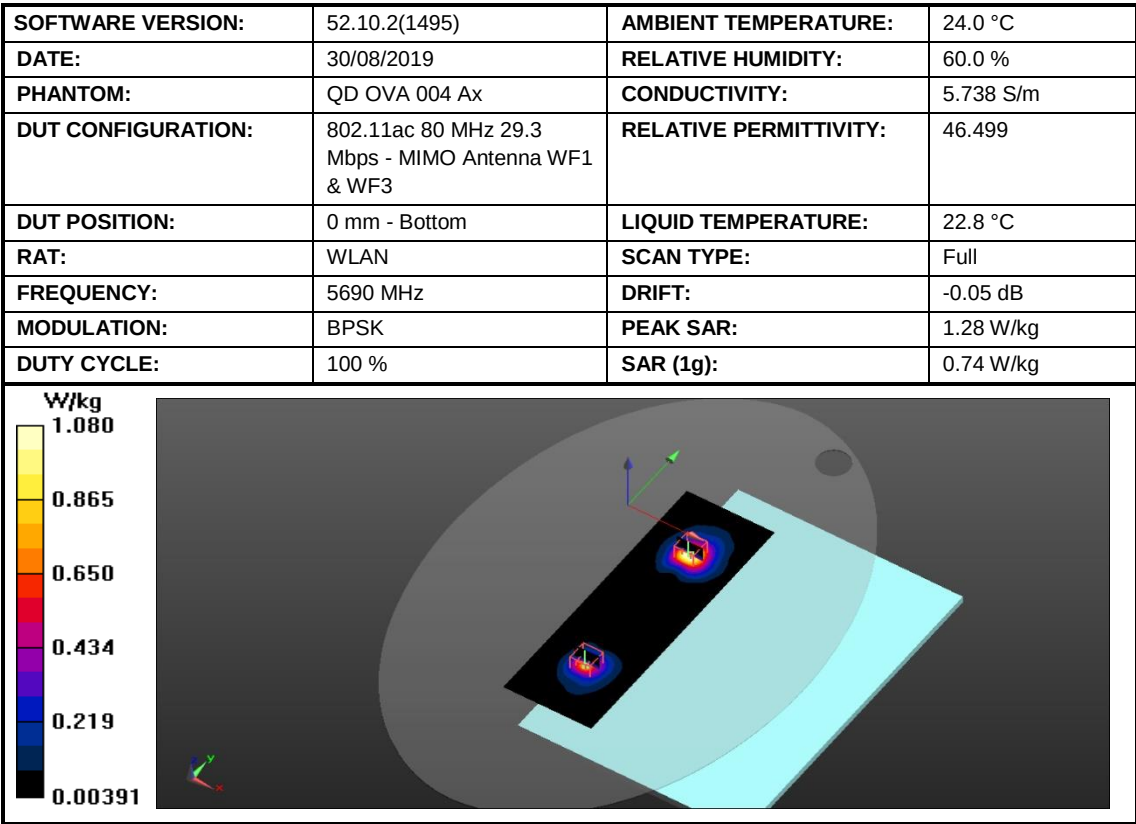
Figure 44: SAR Body Testing Results for the A2141 at 5690 MHz.
