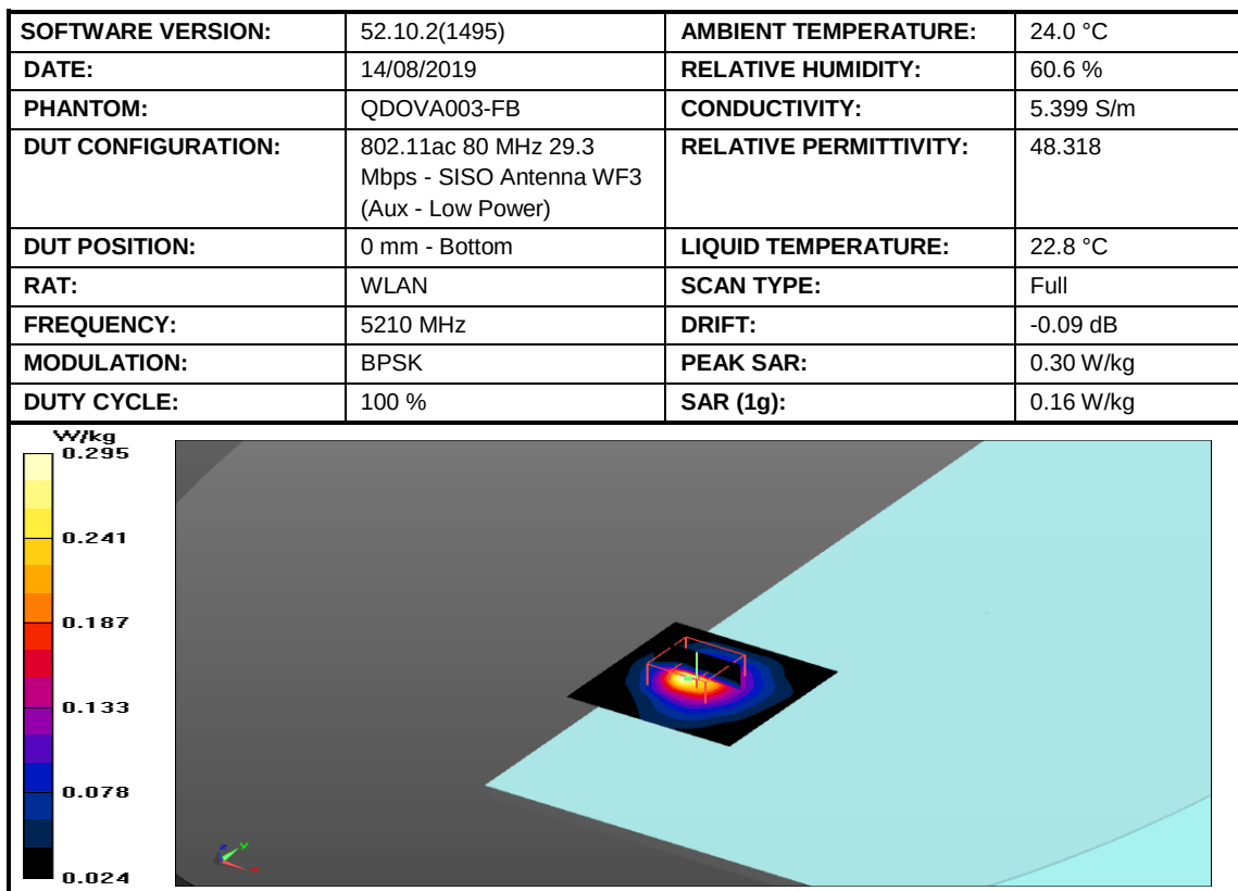
Figure 25: SAR Body Testing Results for the A2141 at 5210 MHz.
