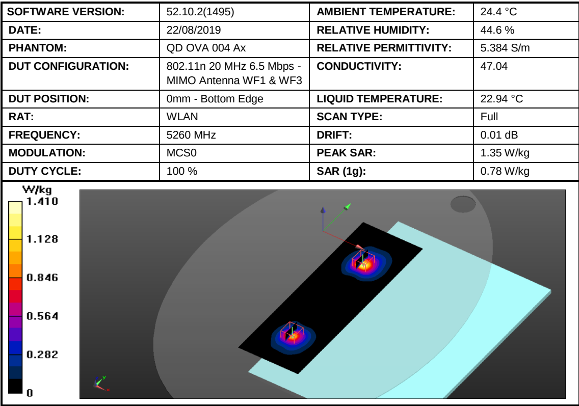
Figure 59: SAR Body Testing Results for the A2141 at 5260 MHz.
