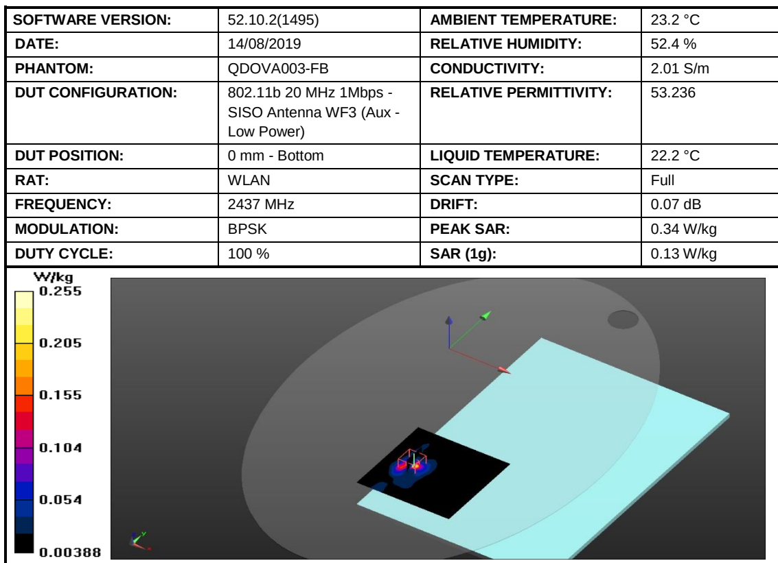
Figure 12: SAR Body Testing Results for the A2141 at 2437 MHz.
