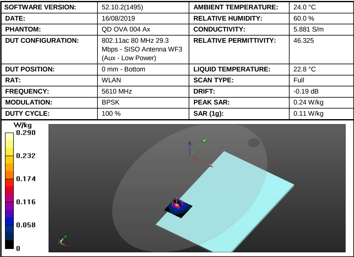
Figure 40: SAR Body Testing Results for the A2141 at 5610 MHz.
