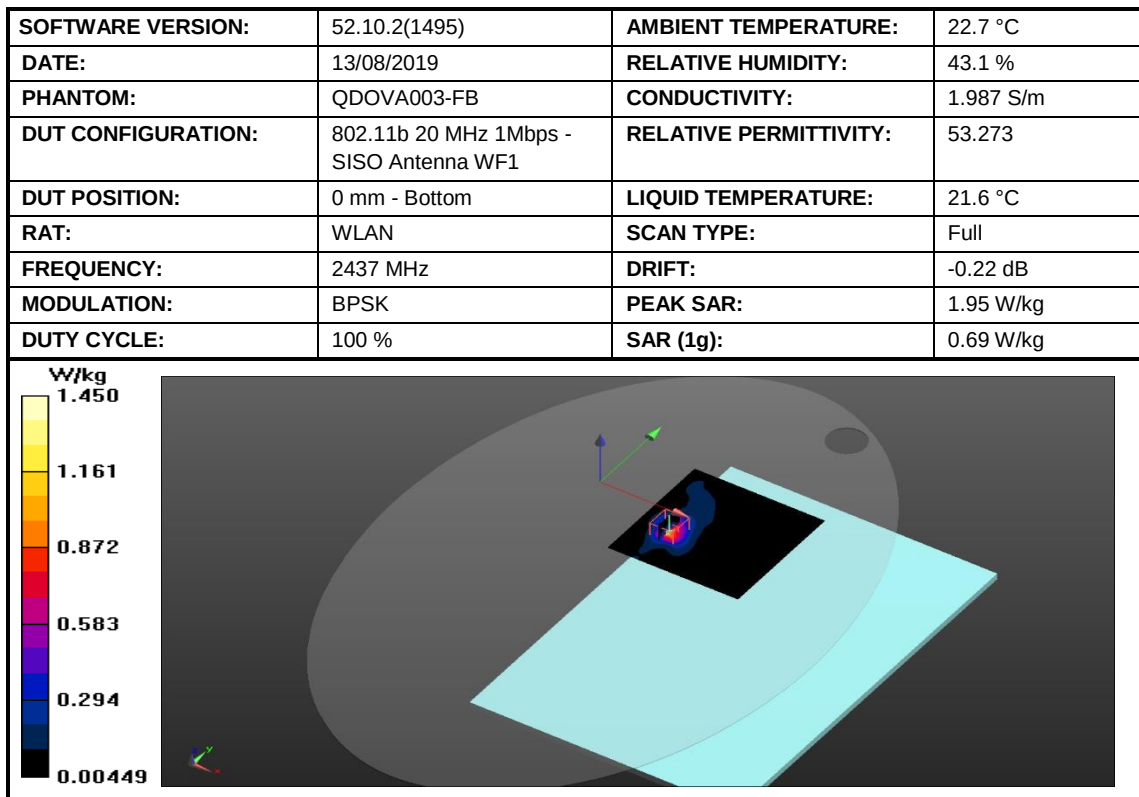
Figure 7: SAR Body Testing Results for the A2141 at 2437 MHz.
