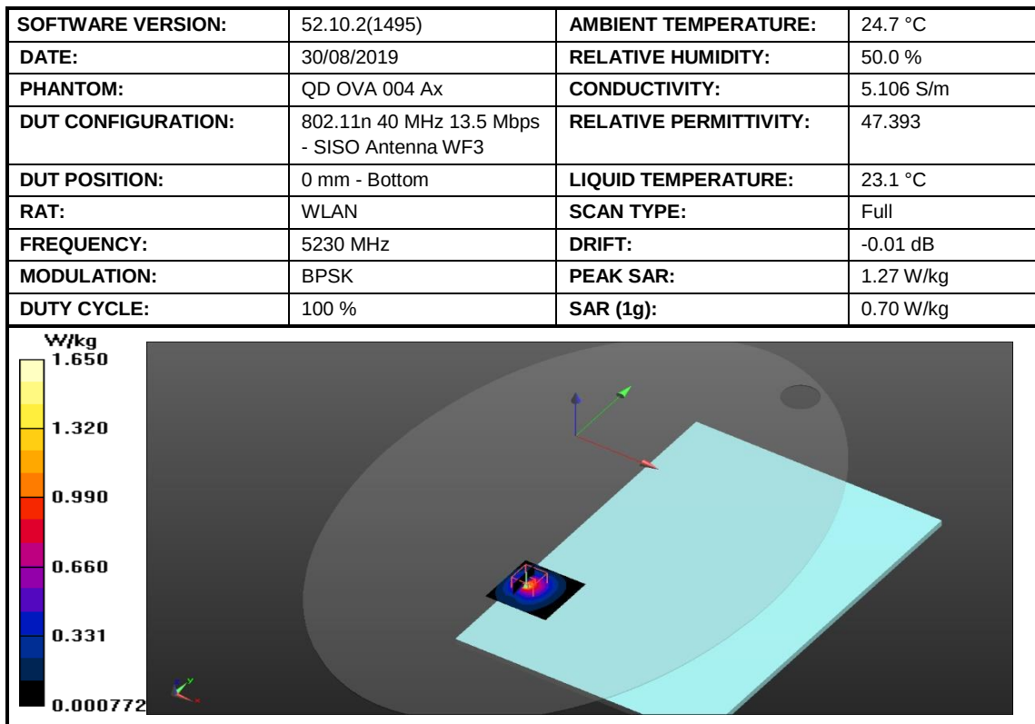
Figure 22: SAR Body Testing Results for the A2141 at 5230 MHz.
