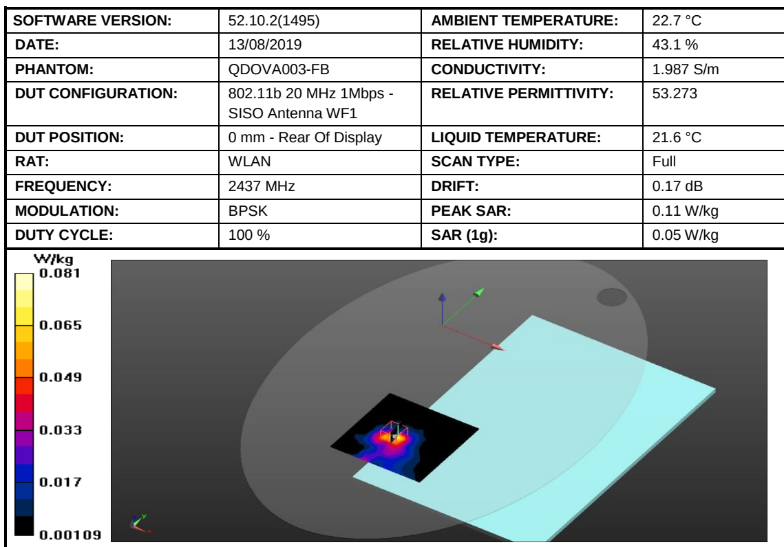
Figure 8: SAR Body Testing Results for the A2141 at 2437 MHz.
