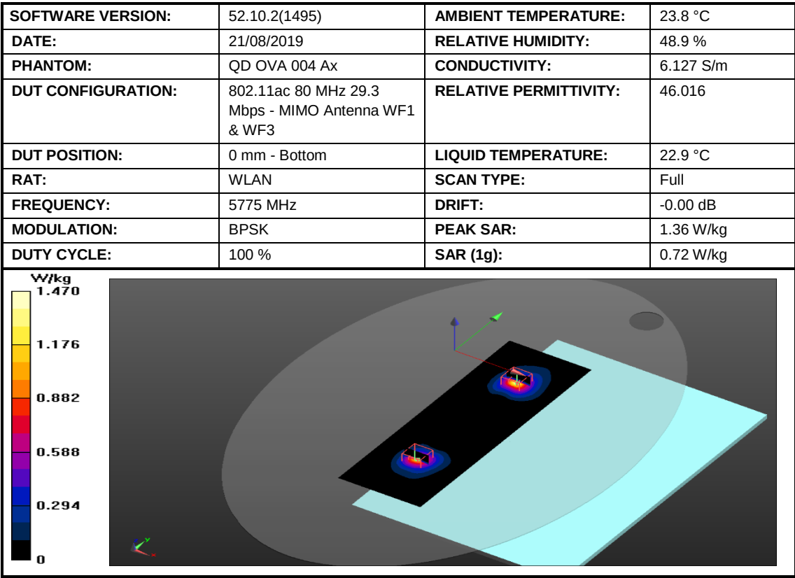
Figure 54: SAR Body Testing Results for the A2141 at 5775 MHz.
