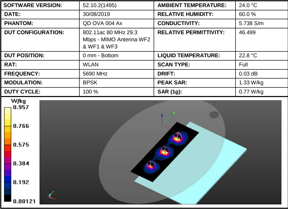
Figure 47: SAR Body Testing Results for the A2141 at 5690 MHz.
