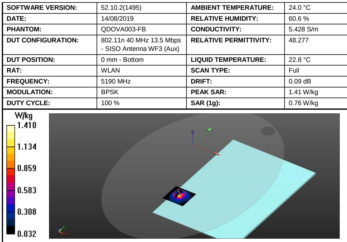
Figure 24: SAR Body Testing Results for the A2141 at 5190 MHz.
