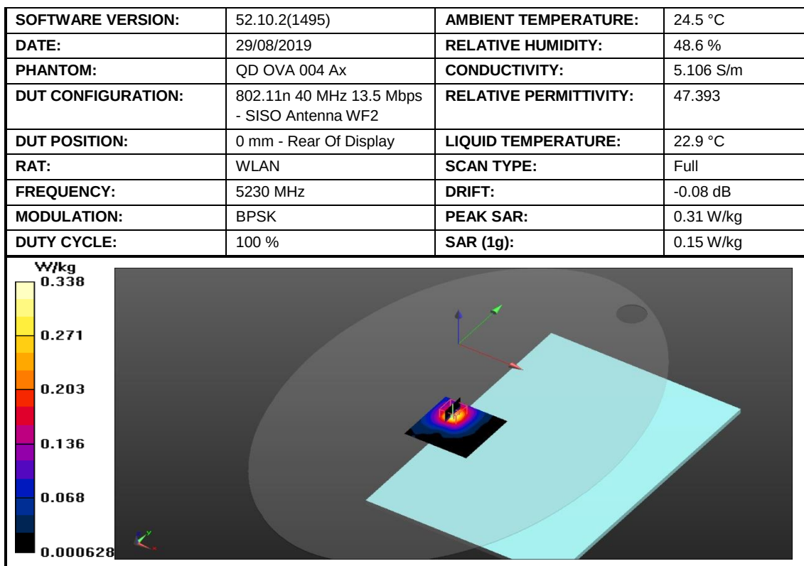
Figure 18: SAR Body Testing Results for the A2141 at 5230 MHz.
