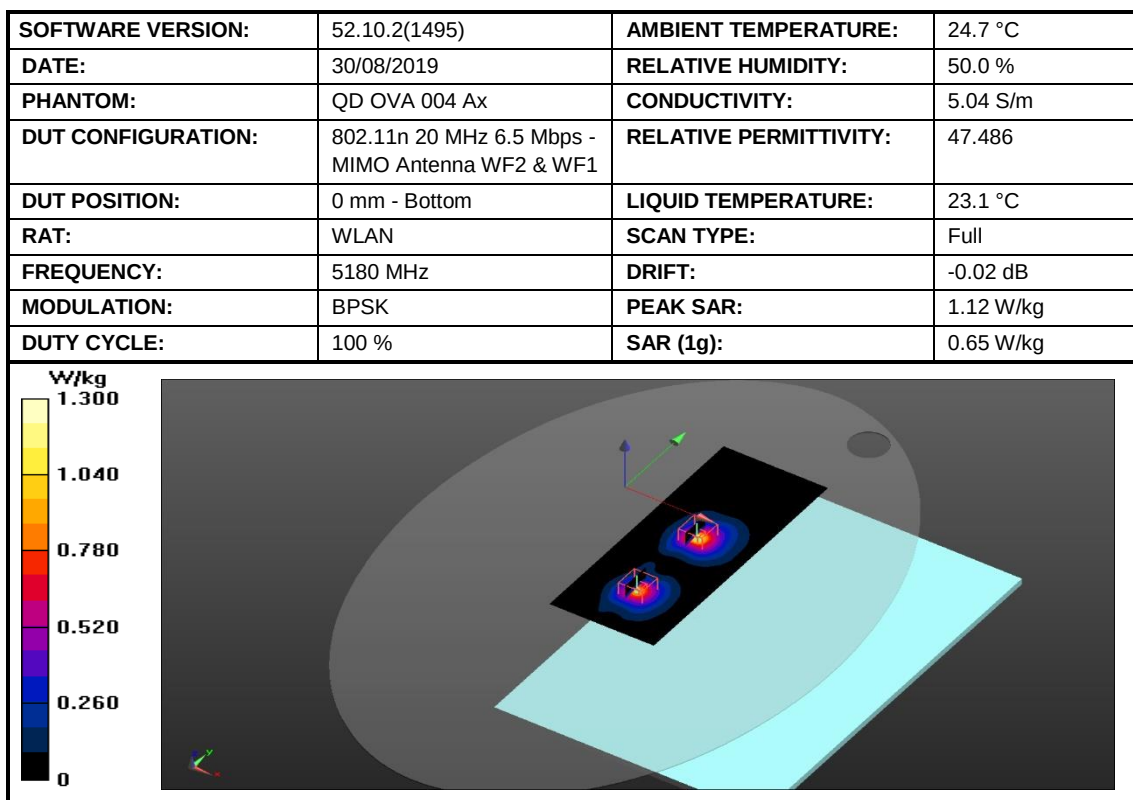
Figure 26: SAR Body Testing Results for the A2141 at 5180 MHz.
