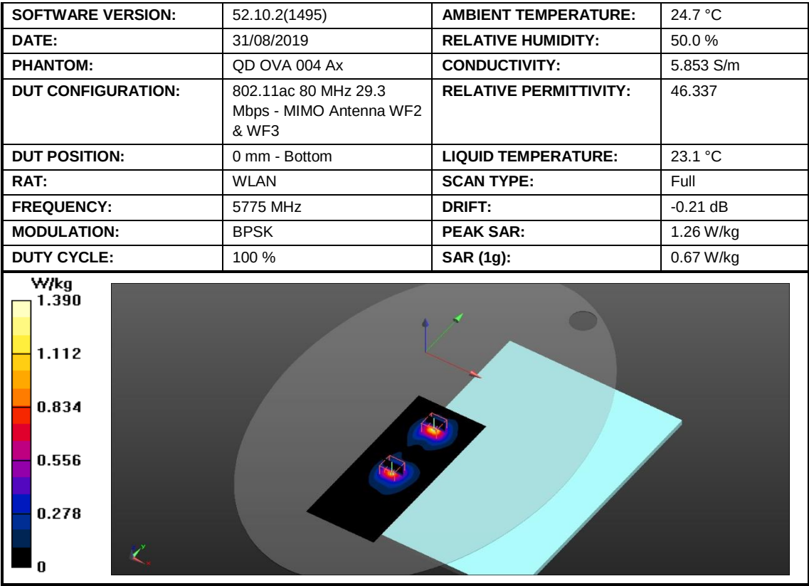
Figure 55: SAR Body Testing Results for the A2141 at 5775 MHz.
