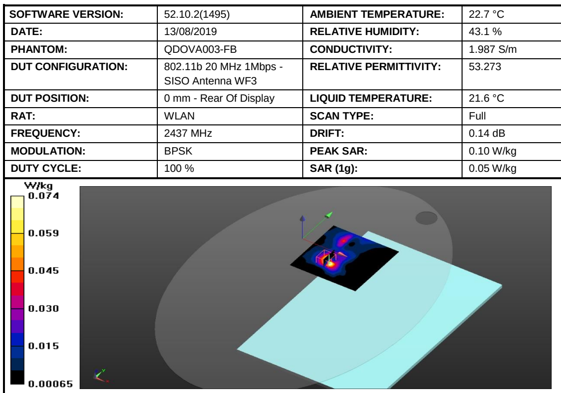
Figure 10: SAR Body Testing Results for the A2141 at 2437 MHz.
