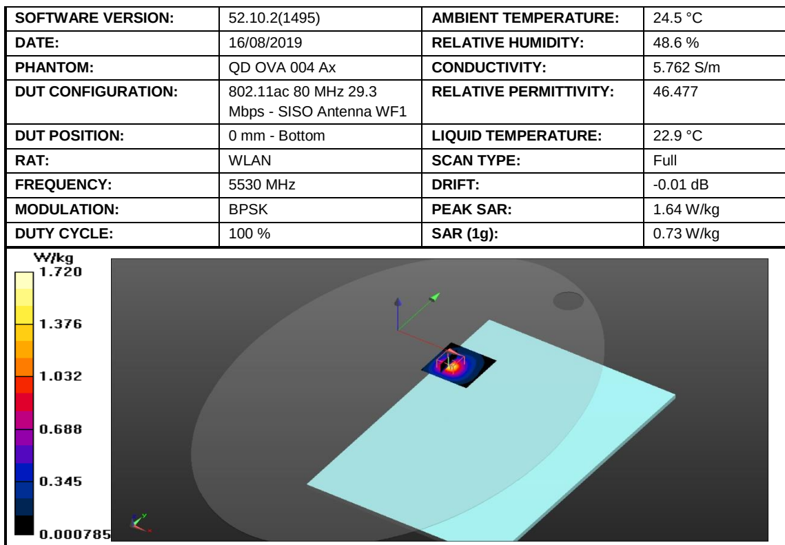
Figure 36: SAR Body Testing Results for the A2141 at 5530 MHz.
