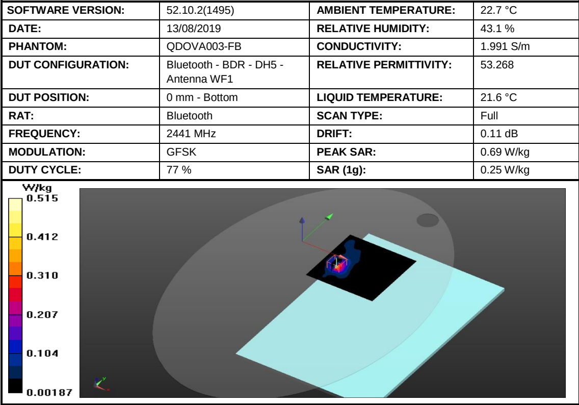
Figure 3: SAR Body Testing Results for the A2141 at 2441 MHz.
