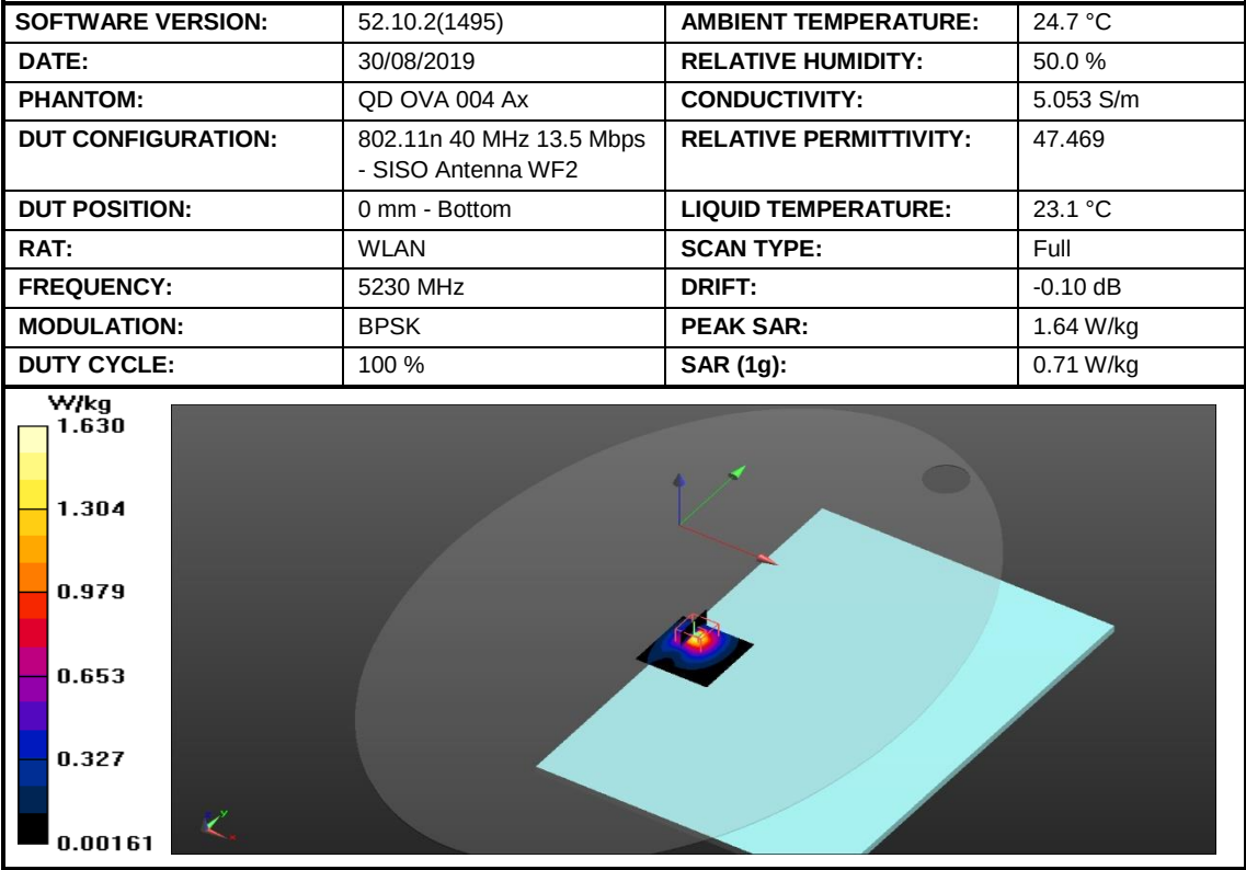
Figure 17: SAR Body Testing Results for the A2141 at 5230 MHz.
