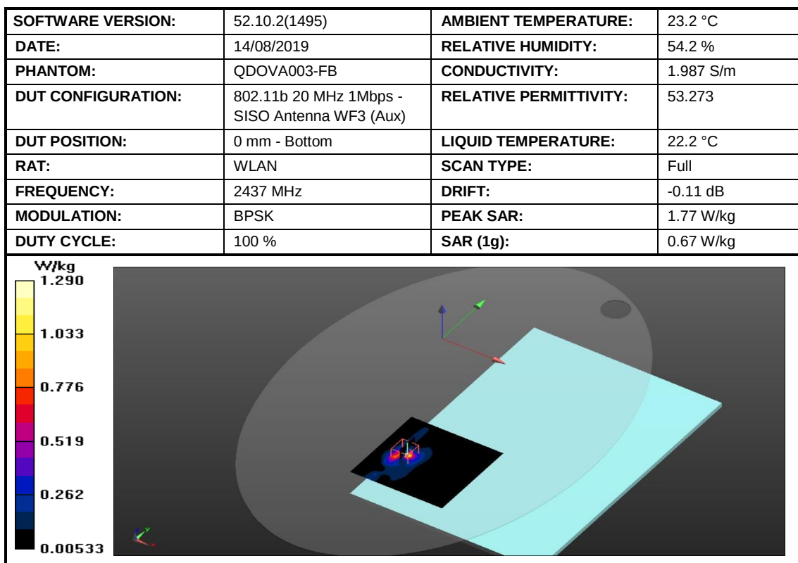
Figure 11: SAR Body Testing Results for the A2141 at 2437 MHz.
