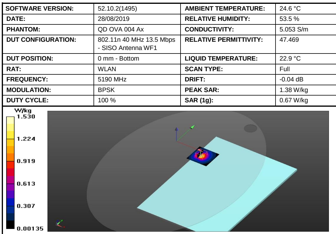
Figure 21: SAR Body Testing Results for the A2141 at 5190 MHz.
