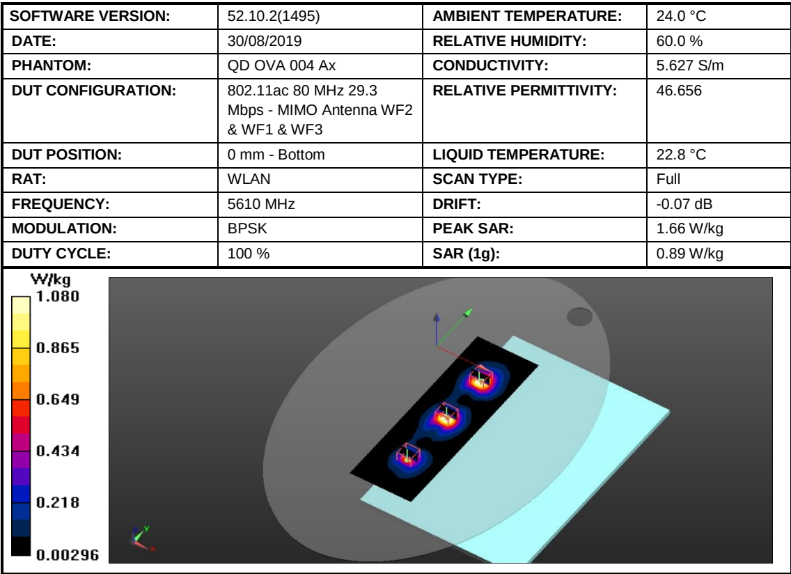
Figure 46: SAR Body Testing Results for the A2141 at 5610 MHz.
