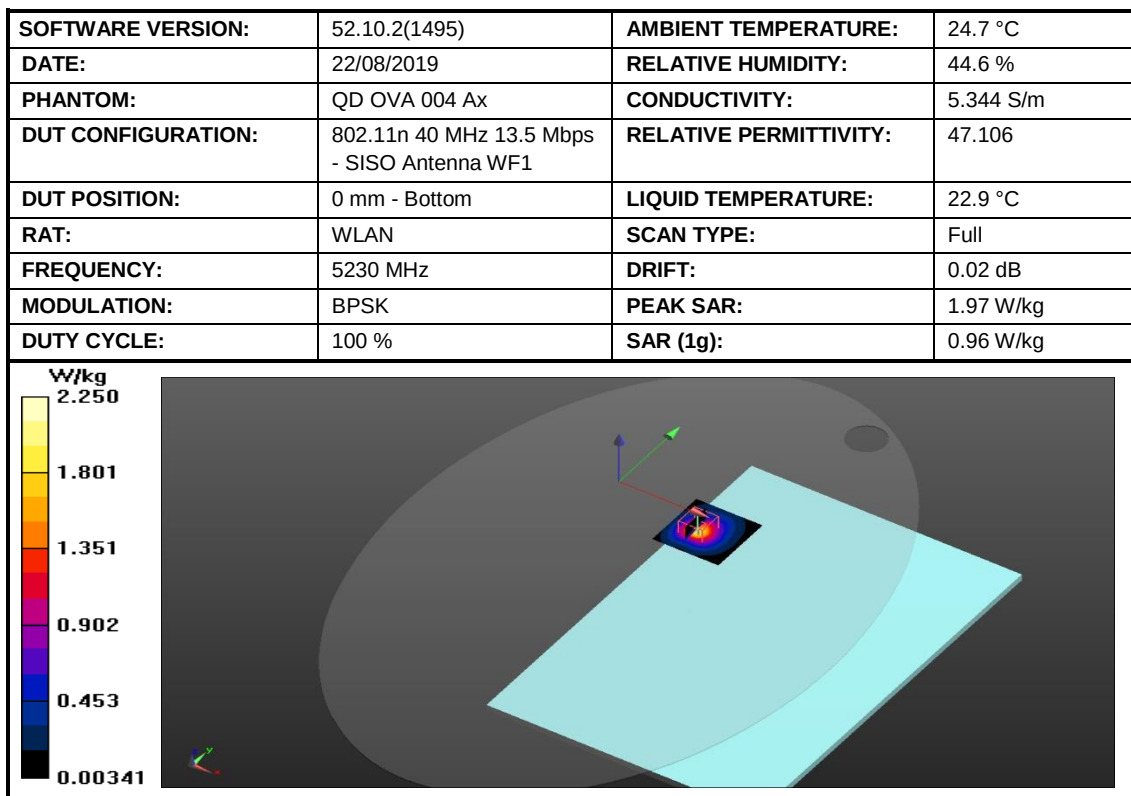
Figure 19: SAR Body Testing Results for the A2141 at 5230 MHz.
