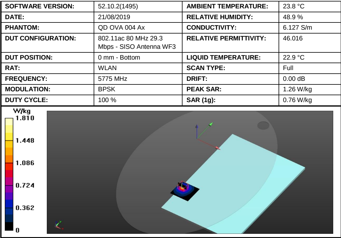
Figure 50: SAR Body Testing Results for the A2141 at 5775 MHz.
