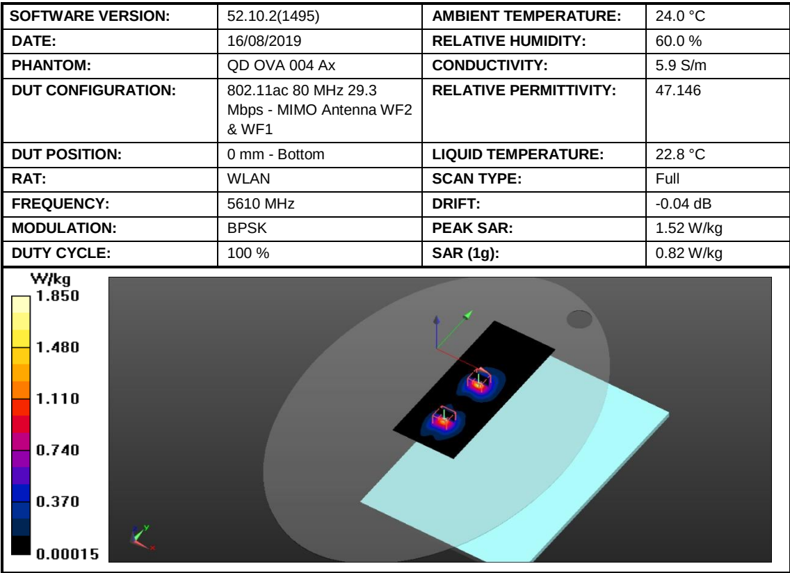
Figure 42: SAR Body Testing Results for the A2141 at 5610 MHz.
