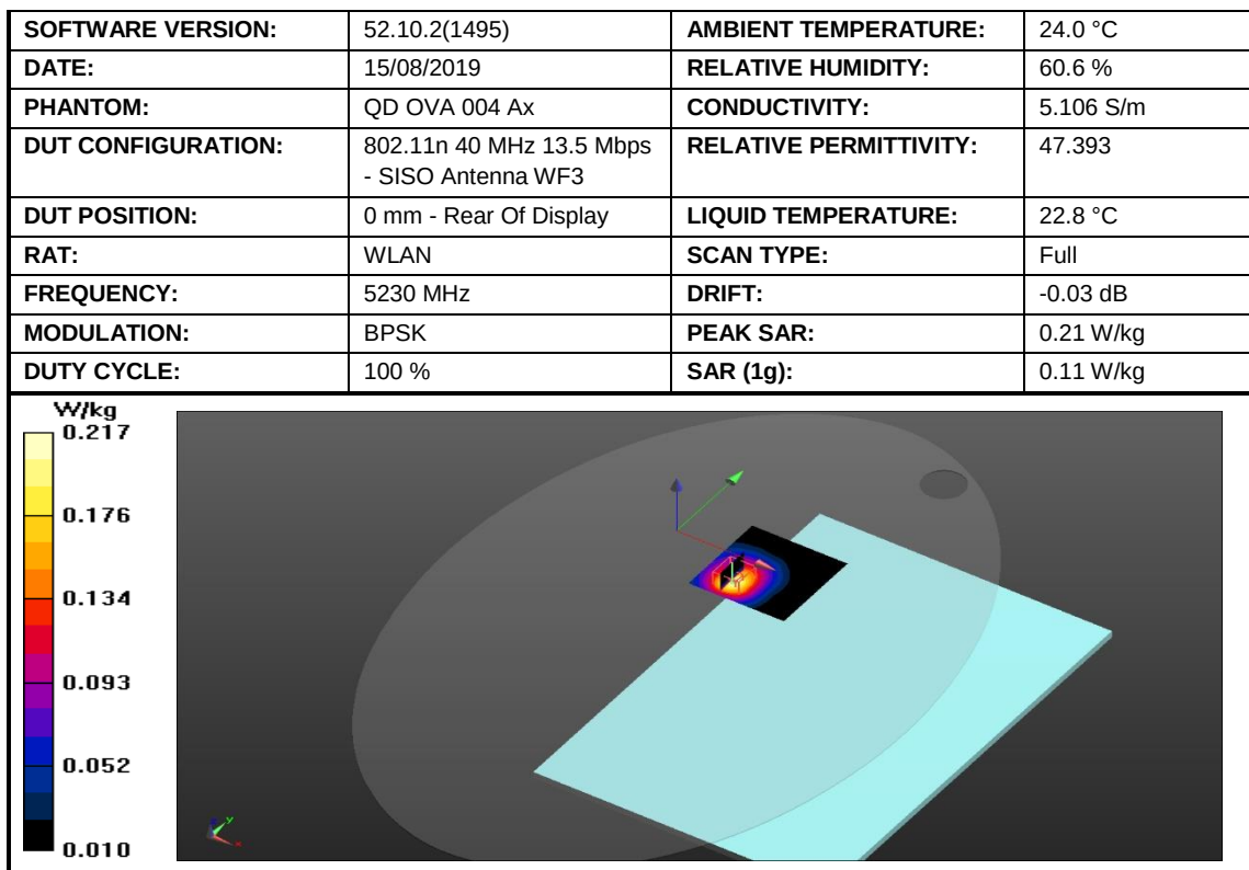
Figure 23: SAR Body Testing Results for the A2141 at 5230 MHz.
