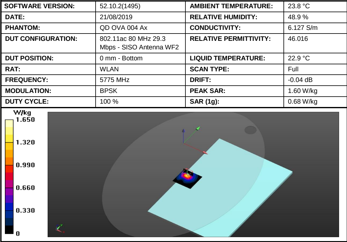
Figure 48: SAR Body Testing Results for the A2141 at 5775 MHz.
