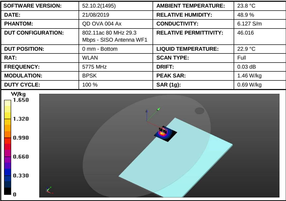
Figure 49: SAR Body Testing Results for the A2141 at 5775 MHz.
