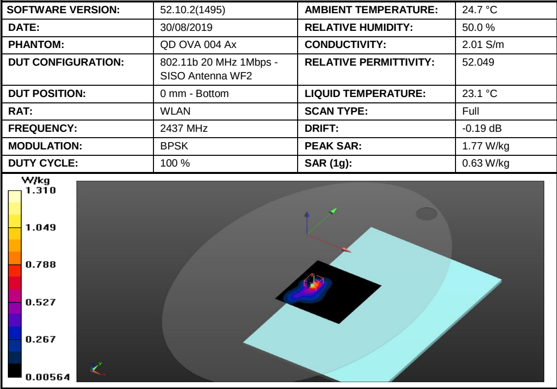
Figure 5: SAR Body Testing Results for the A2141 at 2437 MHz.
