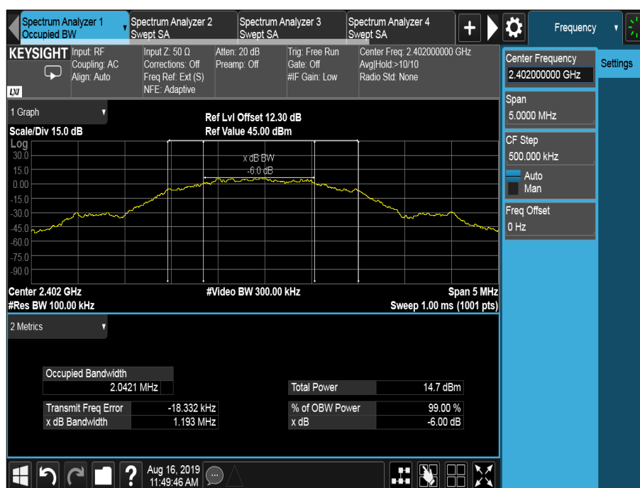
Figure 12 - 2402 MHz
