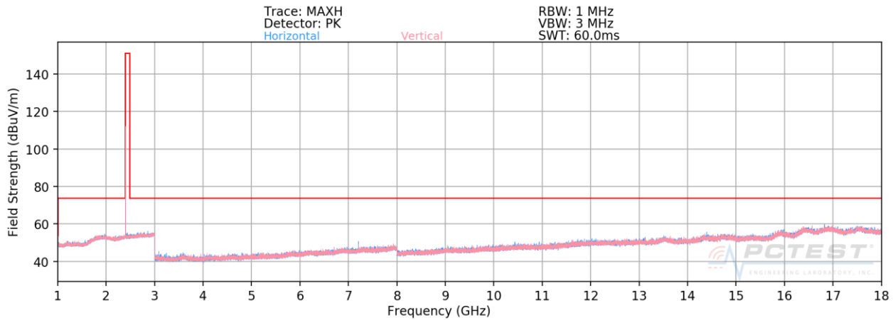
Plot 7-57. Radiated Spurious Plot Above 1GHz ANT 0 (1Mbps, ePA – Ch. 0)
