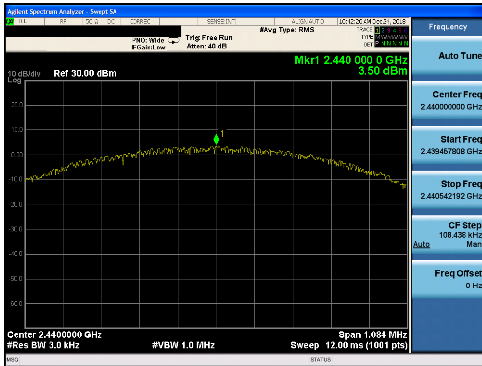
Plot 7-14. Power Spectral Density Plot ANT 0 (Bluetooth (LE), 1Mbps ePA – Ch. 19)
