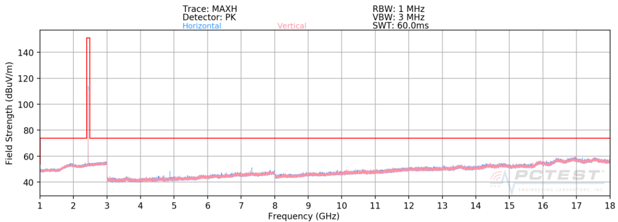
Plot 7-58. Radiated Spurious Plot Above 1GHz ANT 0 (1Mbps, ePA – Ch. 19)
