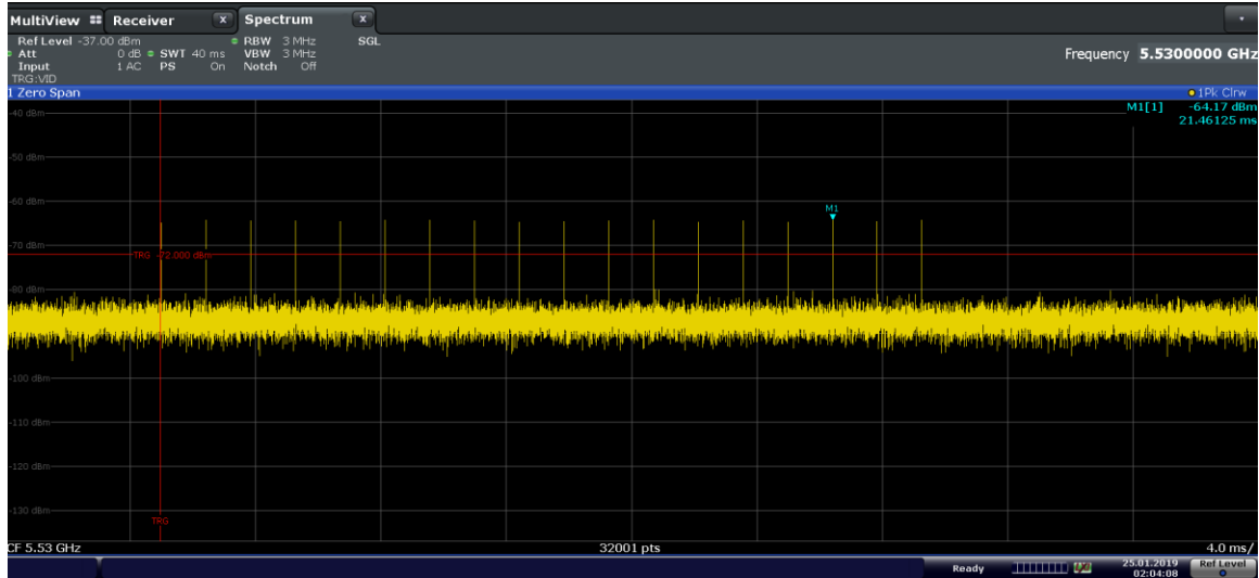
Figure 7-5. 5530MHz – Radar Pulse Type 0 (80MHz)
