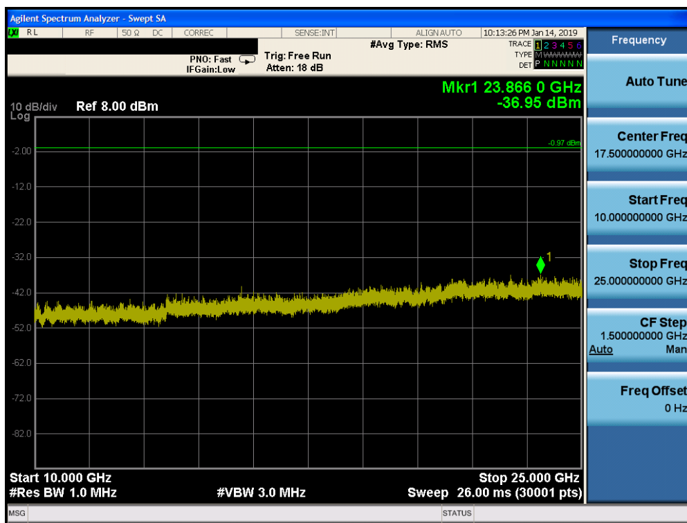
Plot 7-82. Conducted Spurious Plot ANT 1 (Bluetooth, GFSK, ePA Ch. 39)
